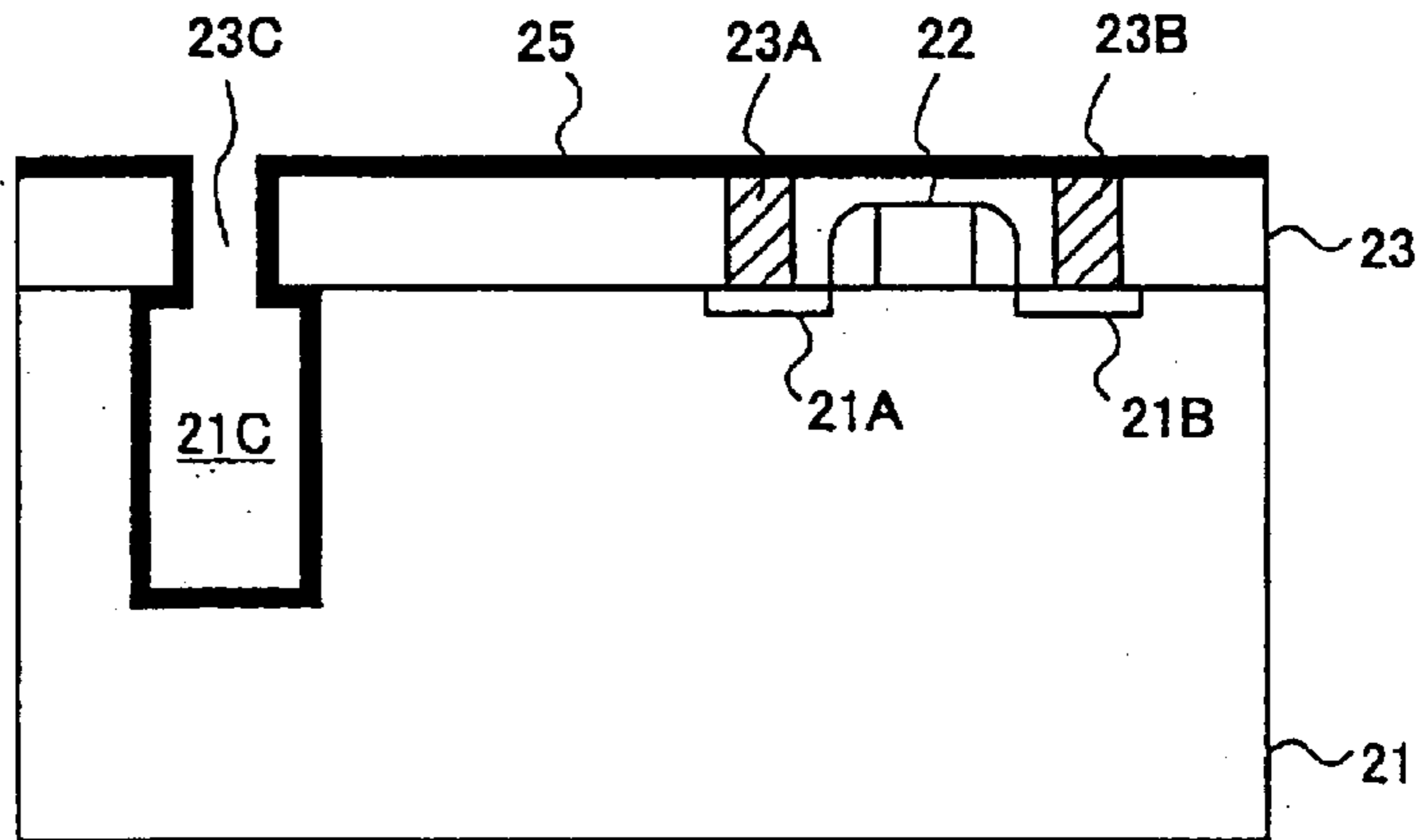
FIG. 4 PRIOR ART
