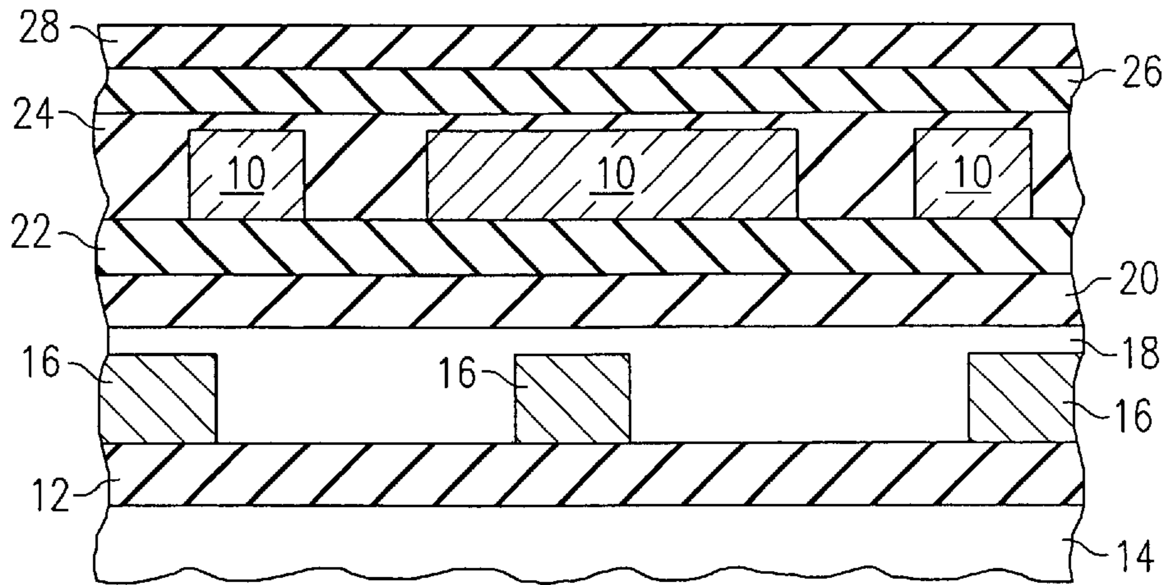
FIG. 1 (PRIOR ART)
