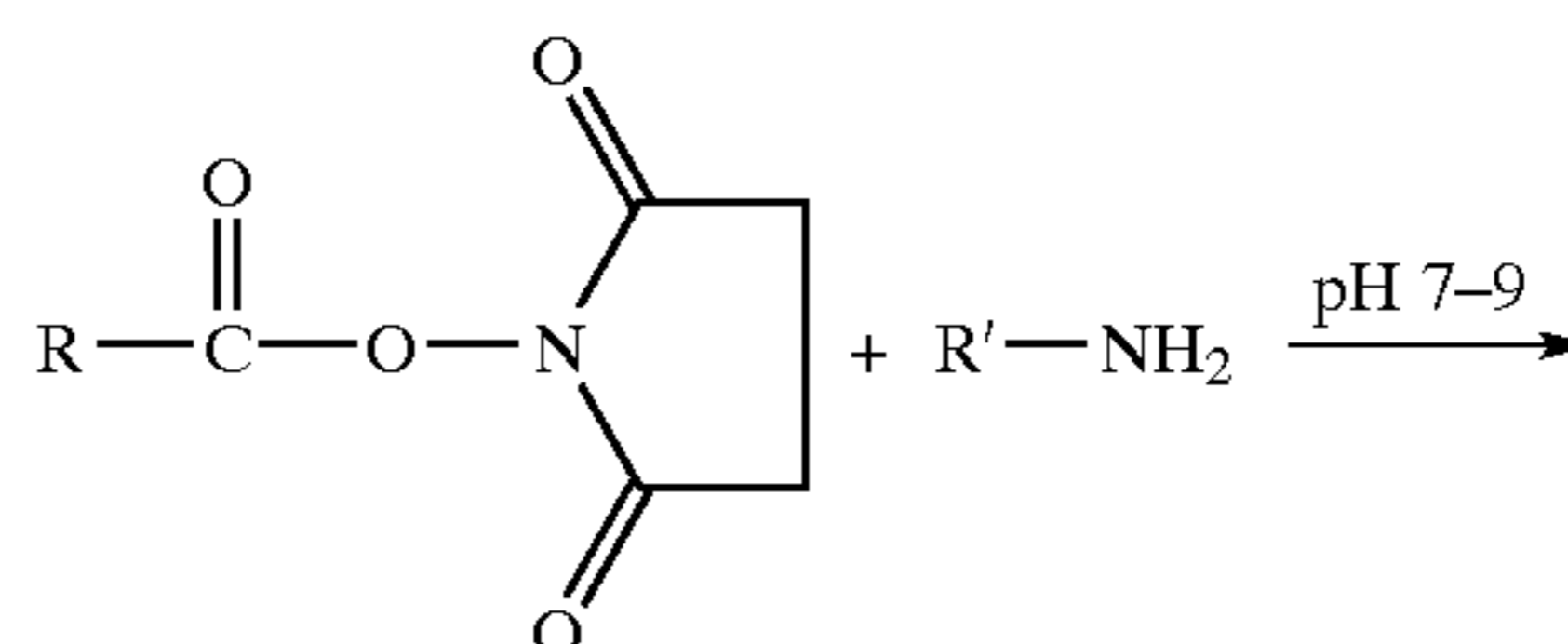
NHS-Ester Reaction Scheme
