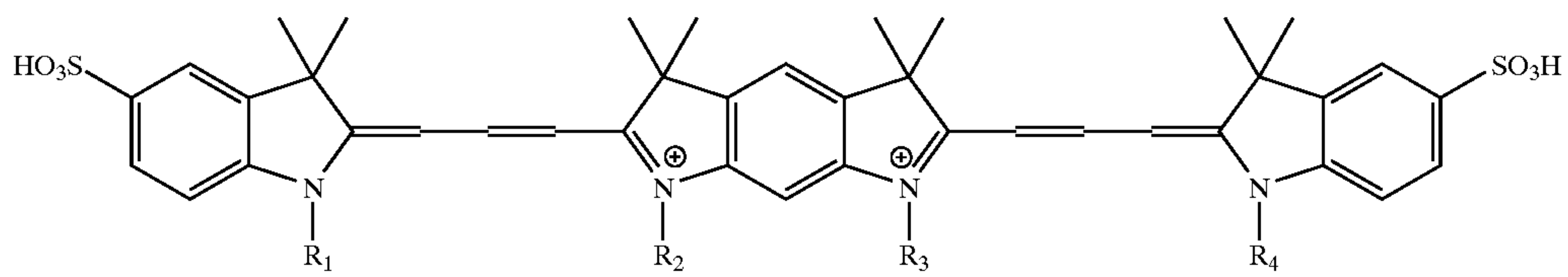
(Formula 11)
