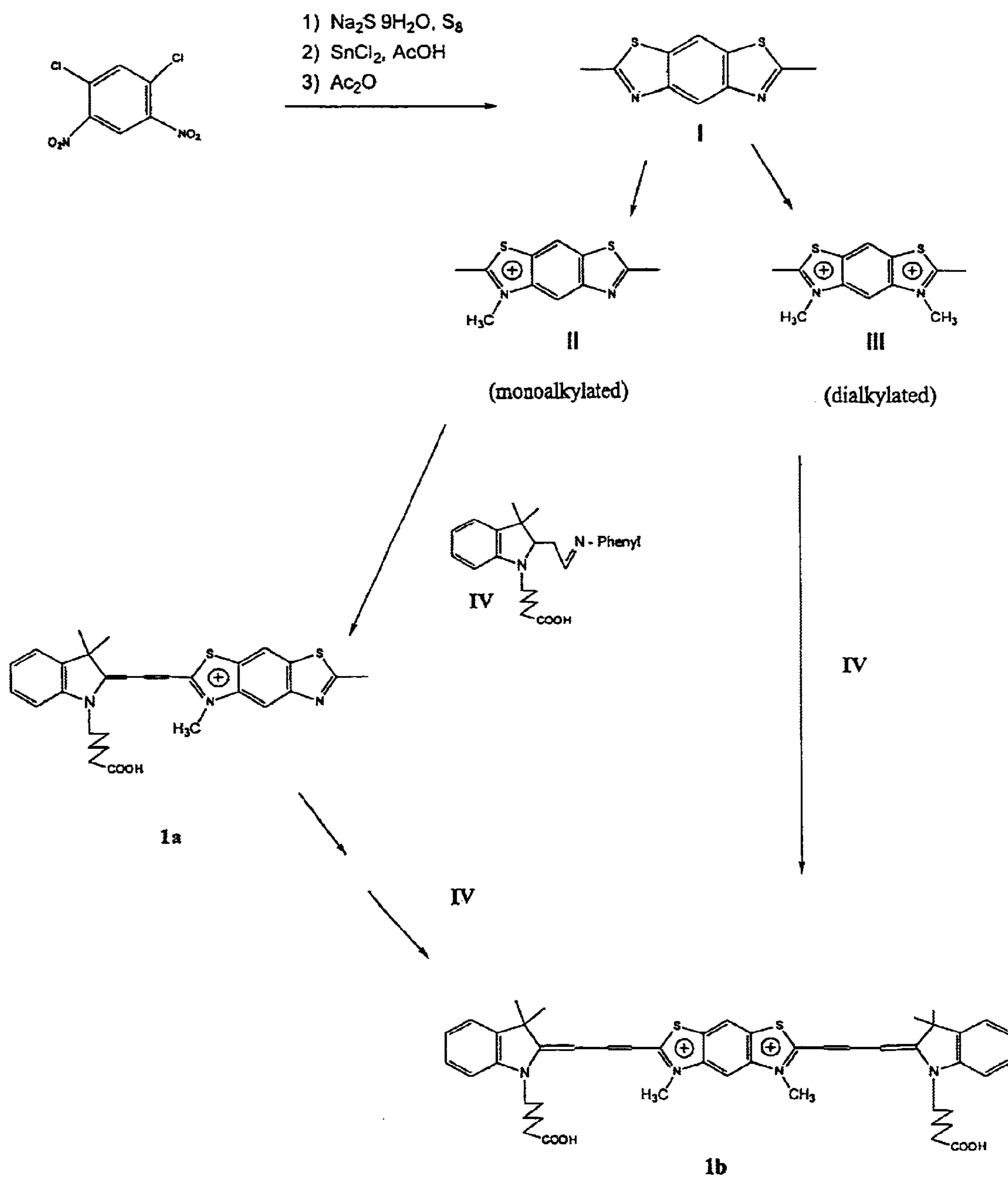
Figure 1 Dyes Containing a Linear Fused Heterocycle. Synthetic Scheme for the Synthesis of Dyes Containing the Benzo[1,2-d:5,4-d']bisthiazole Moiety
