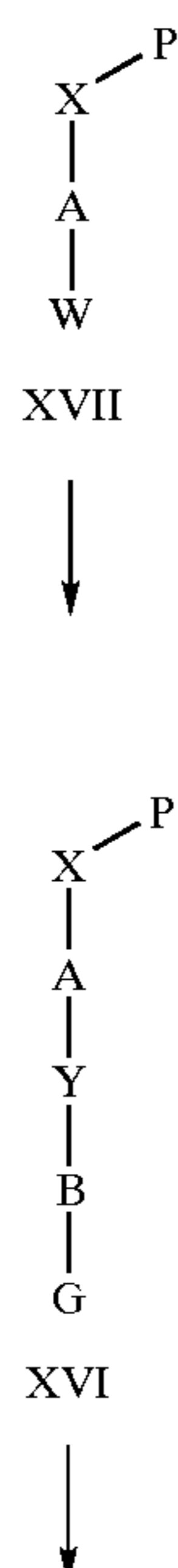
SCHEME 5
