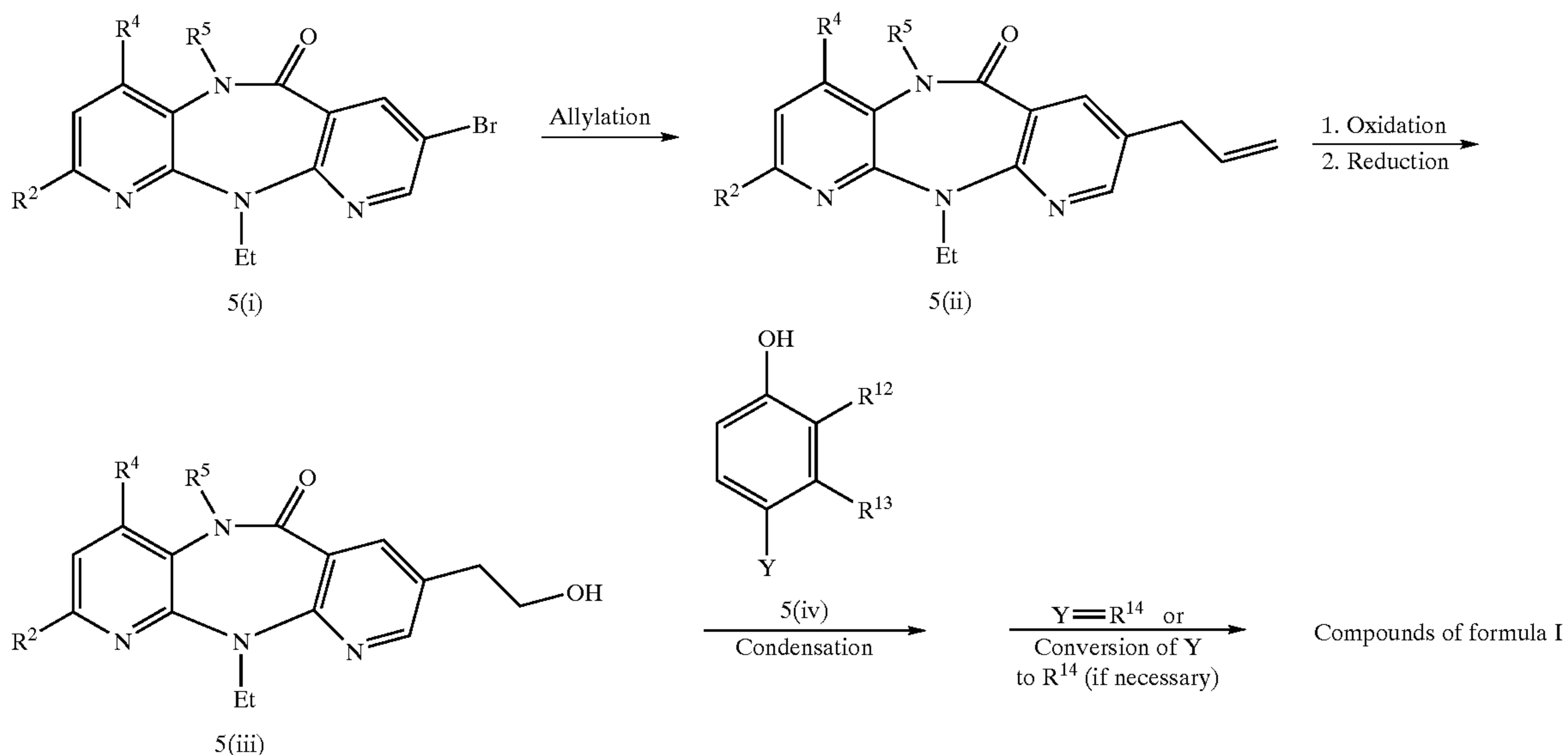
Scheme 5 Introduction of the benzoic acid derivatives
