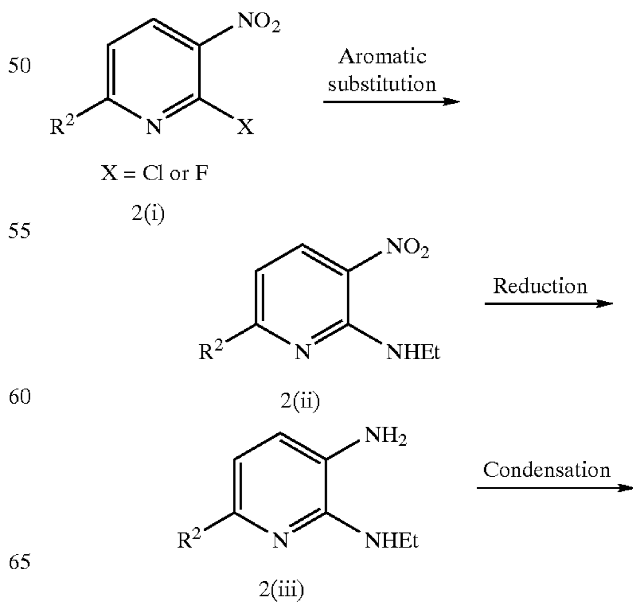
Scheme 2 Preparation of intermediates in which R^5 is Me
