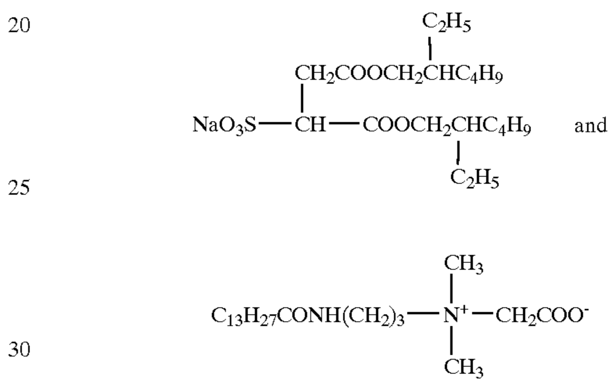
(Cpd-14)
