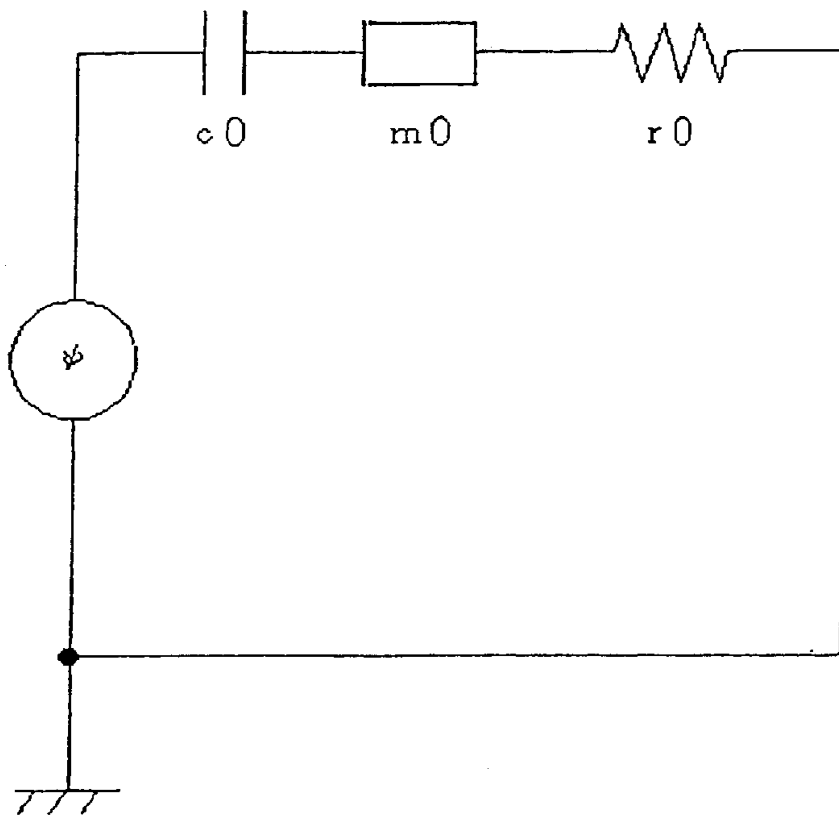
Driving system
