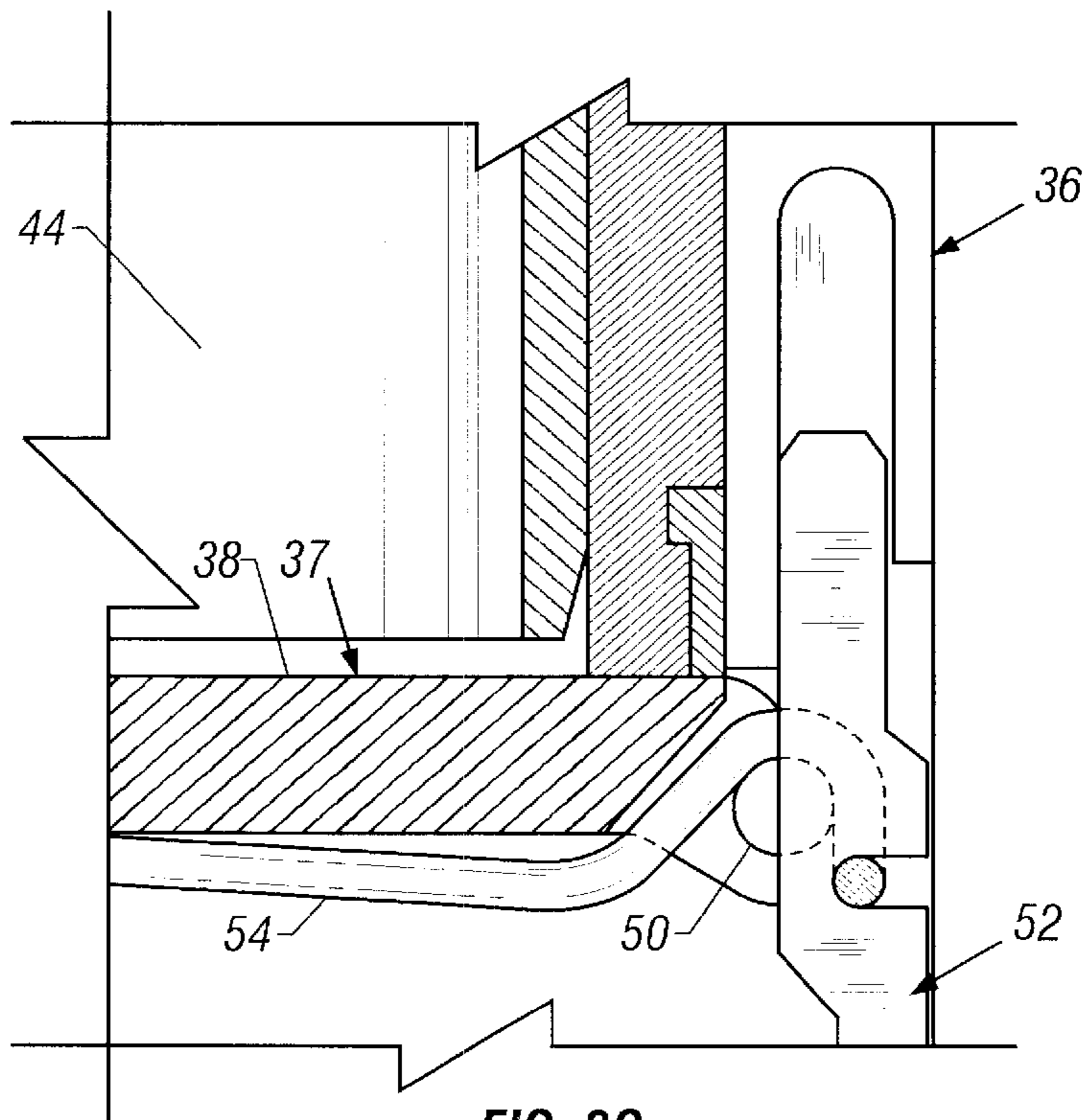
FIG. 3C (Prior Art)
