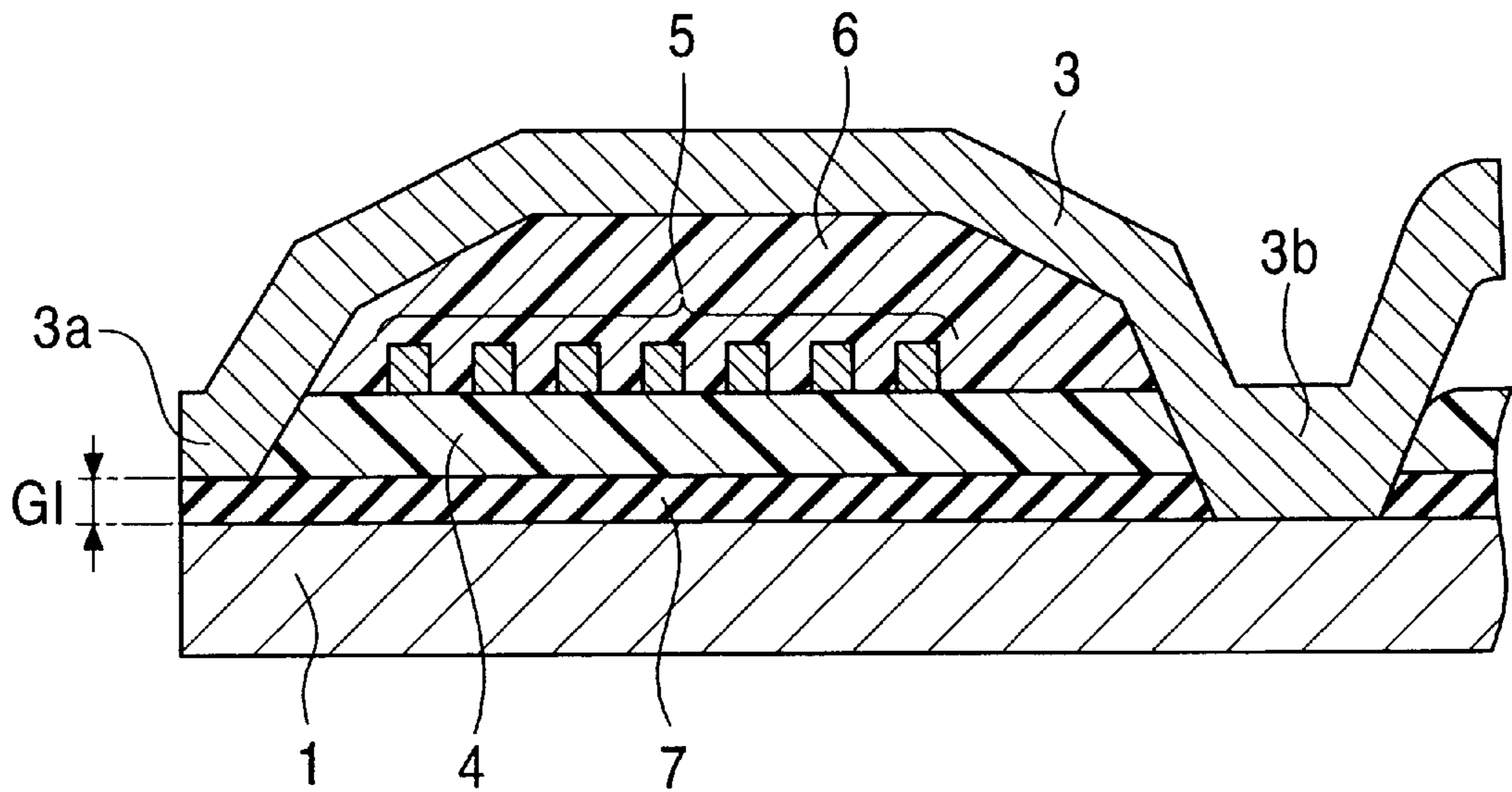
FIG. 13 PRIOR ART
