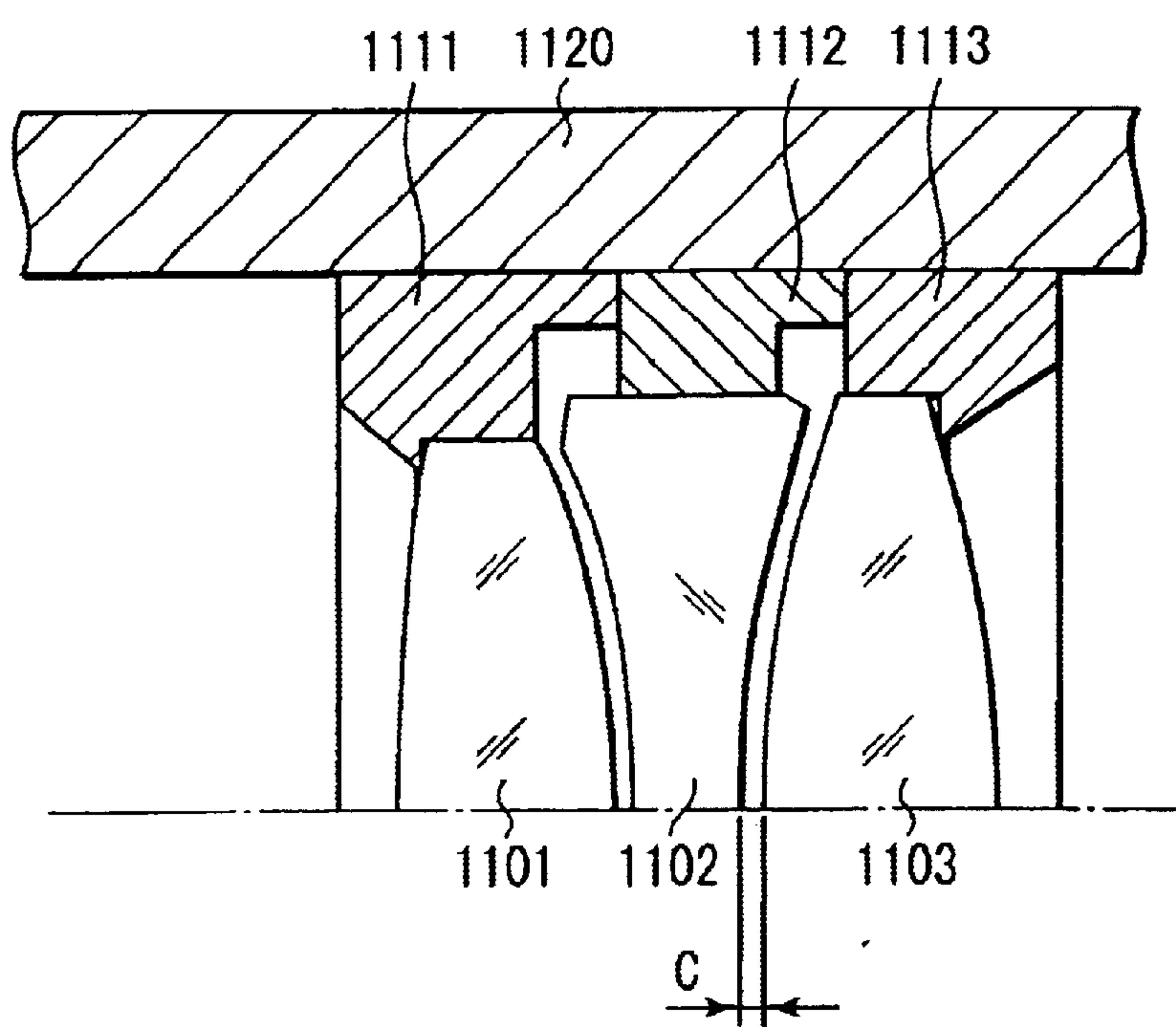
FIG. 18 (PRIOR ART)
