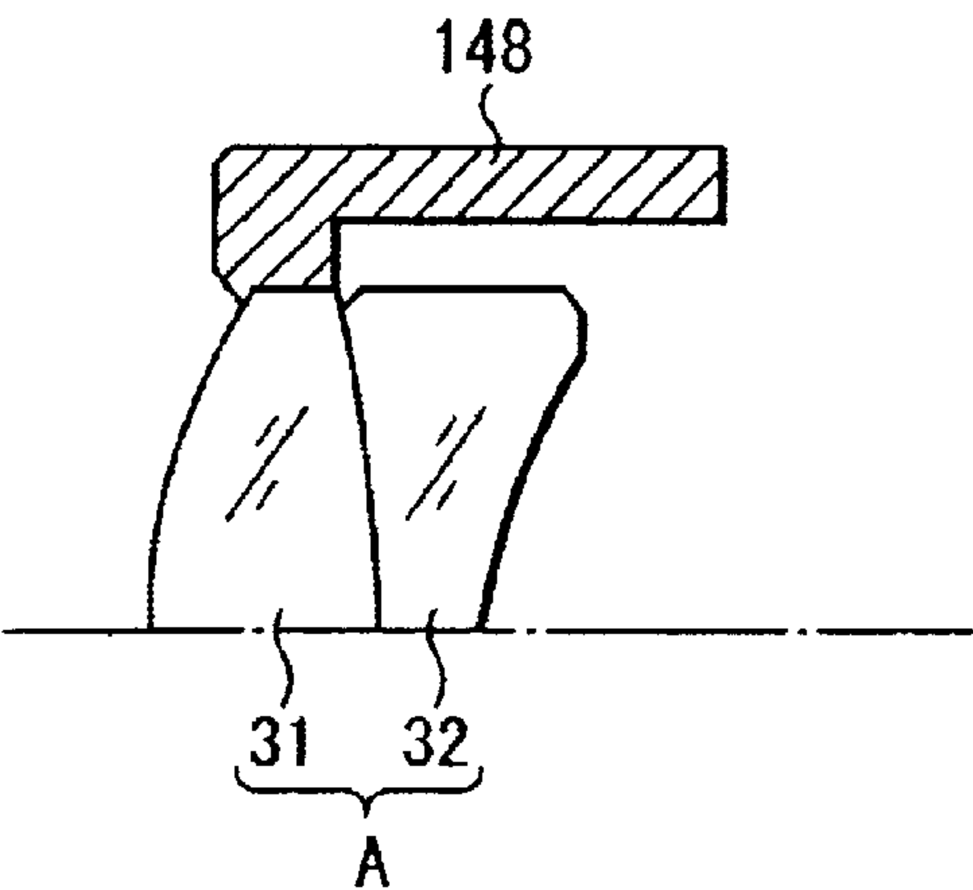
FIG. 12 (PRIOR ART)
