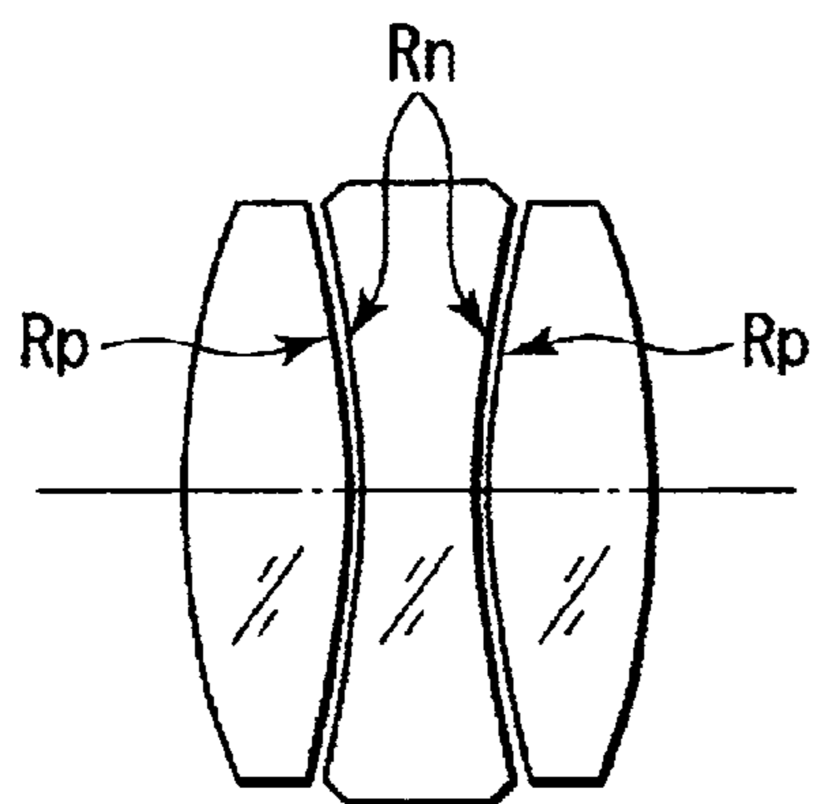
FIG. 11 (PRIOR ART)
