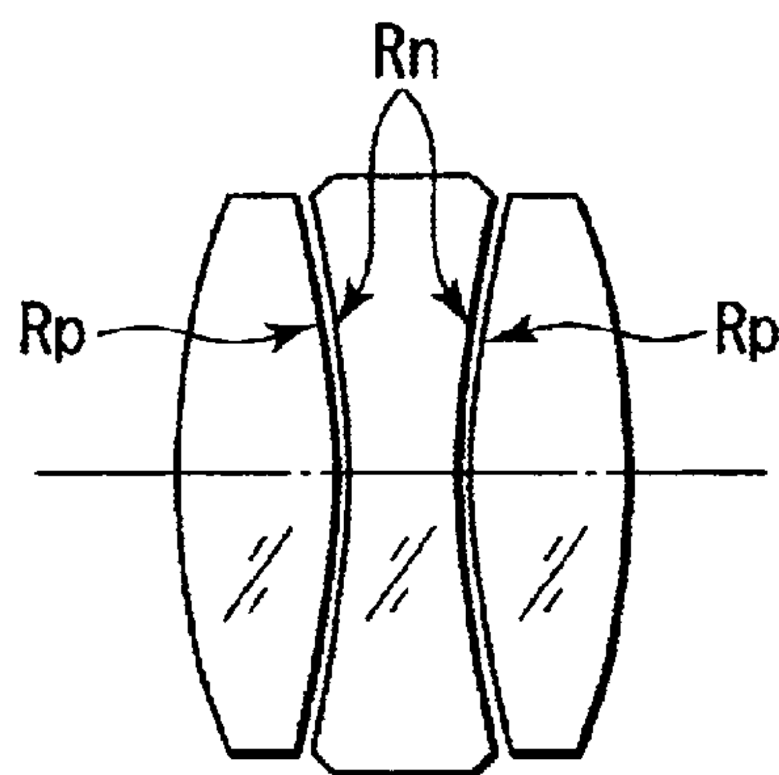
FIG. 11 (PRIOR ART)
