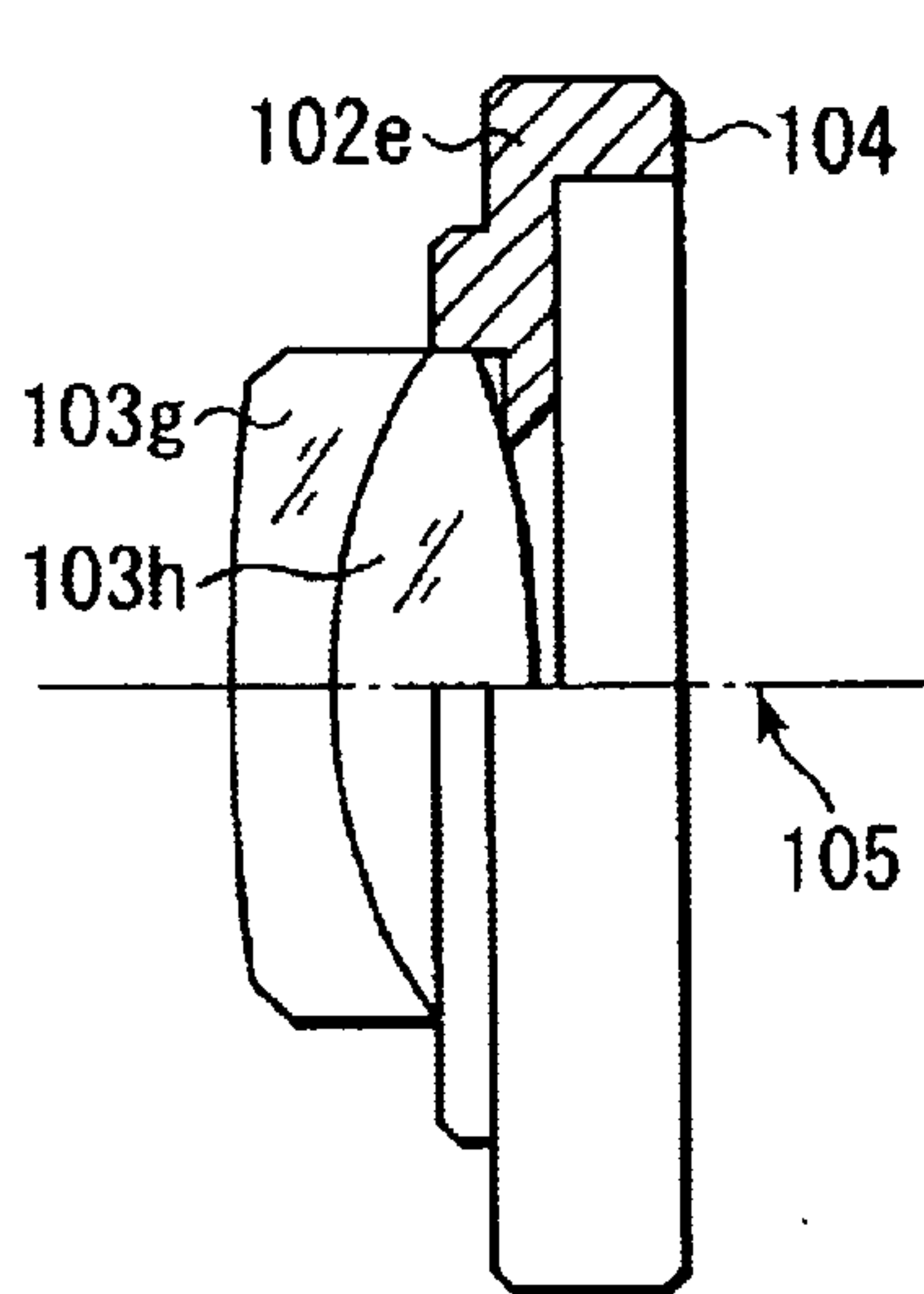
FIG. 8 (PRIOR ART)
