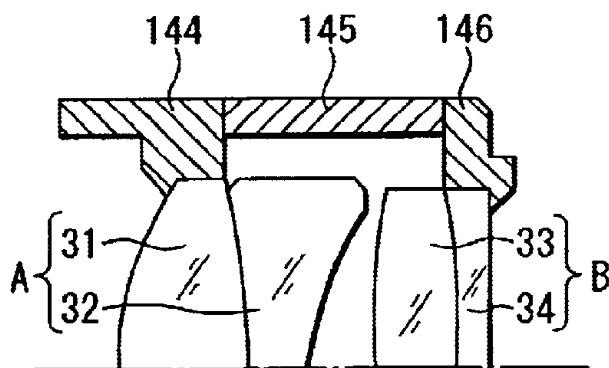
FIG. 10 (PRIOR ART)
