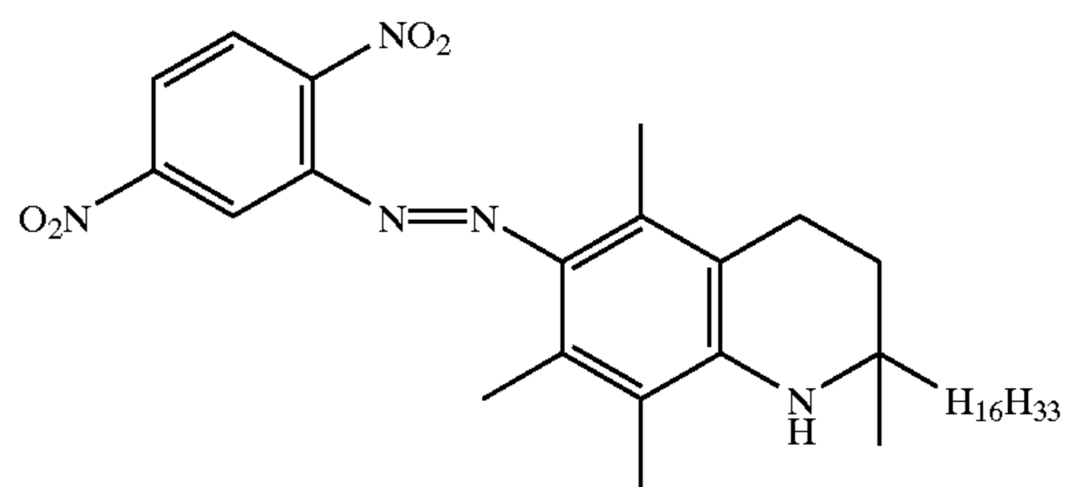
6-(2,4-Dinitrophenylazo(2,5,7,8-tetramethyl-2-(4,8,12-trimethyltridecyl)-1,2,3,4-tetrahydroquinoline (43)
