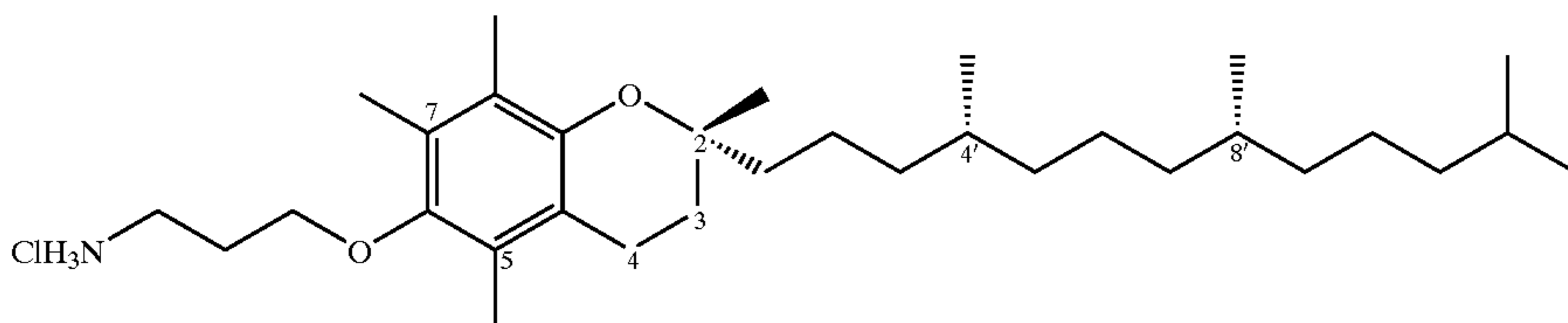
3-(2,5,7,8-Tetramethyl-(2R-(4R,8g,12-trimethyltridecyl)chroman-6-yloxy)propyl-1-ammonium Chloride (19)
