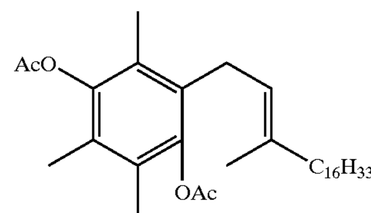
Phytyltrimethylhydroquinone Diacetate (32)
