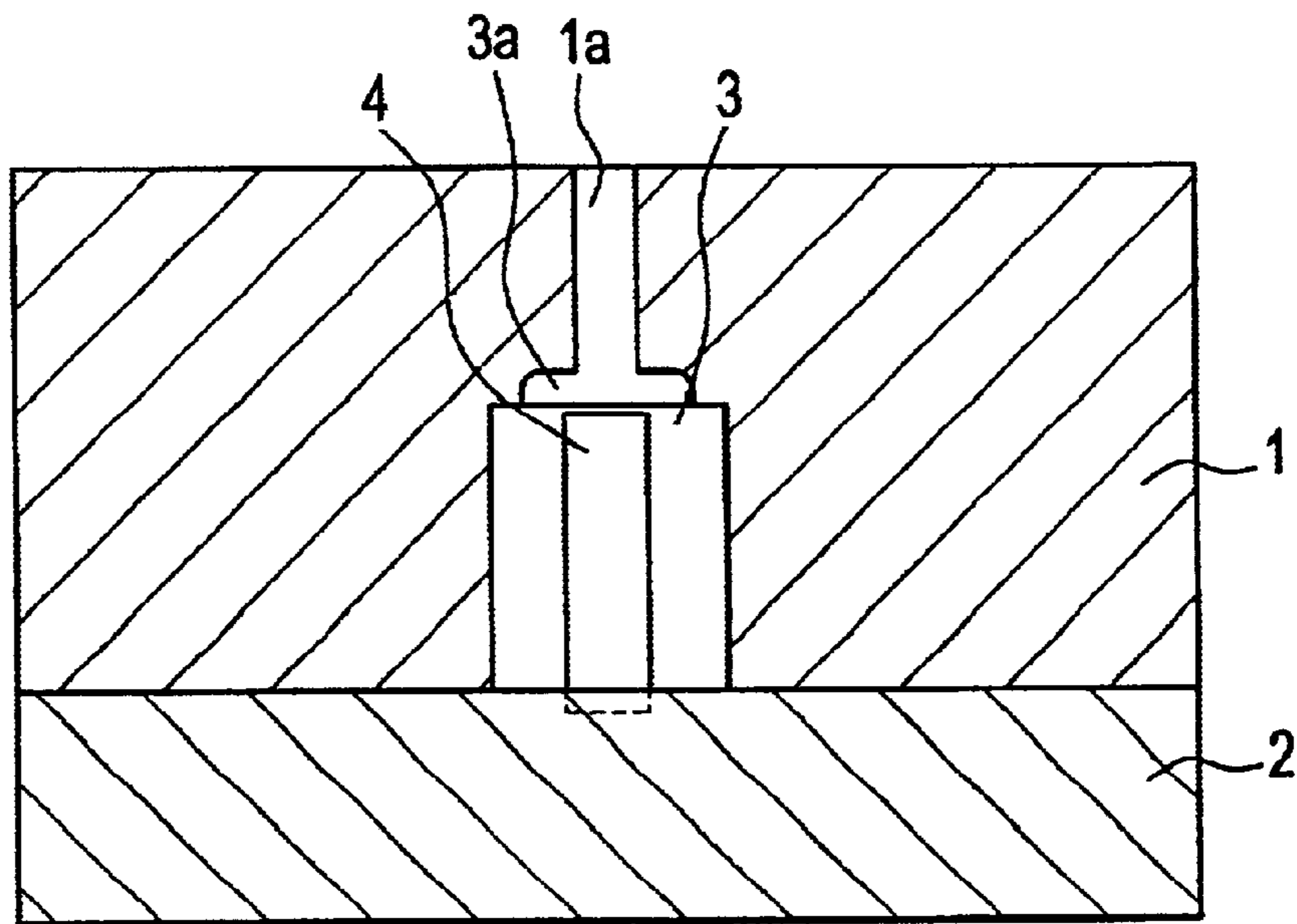
FIG. 6 PRIOR ART
