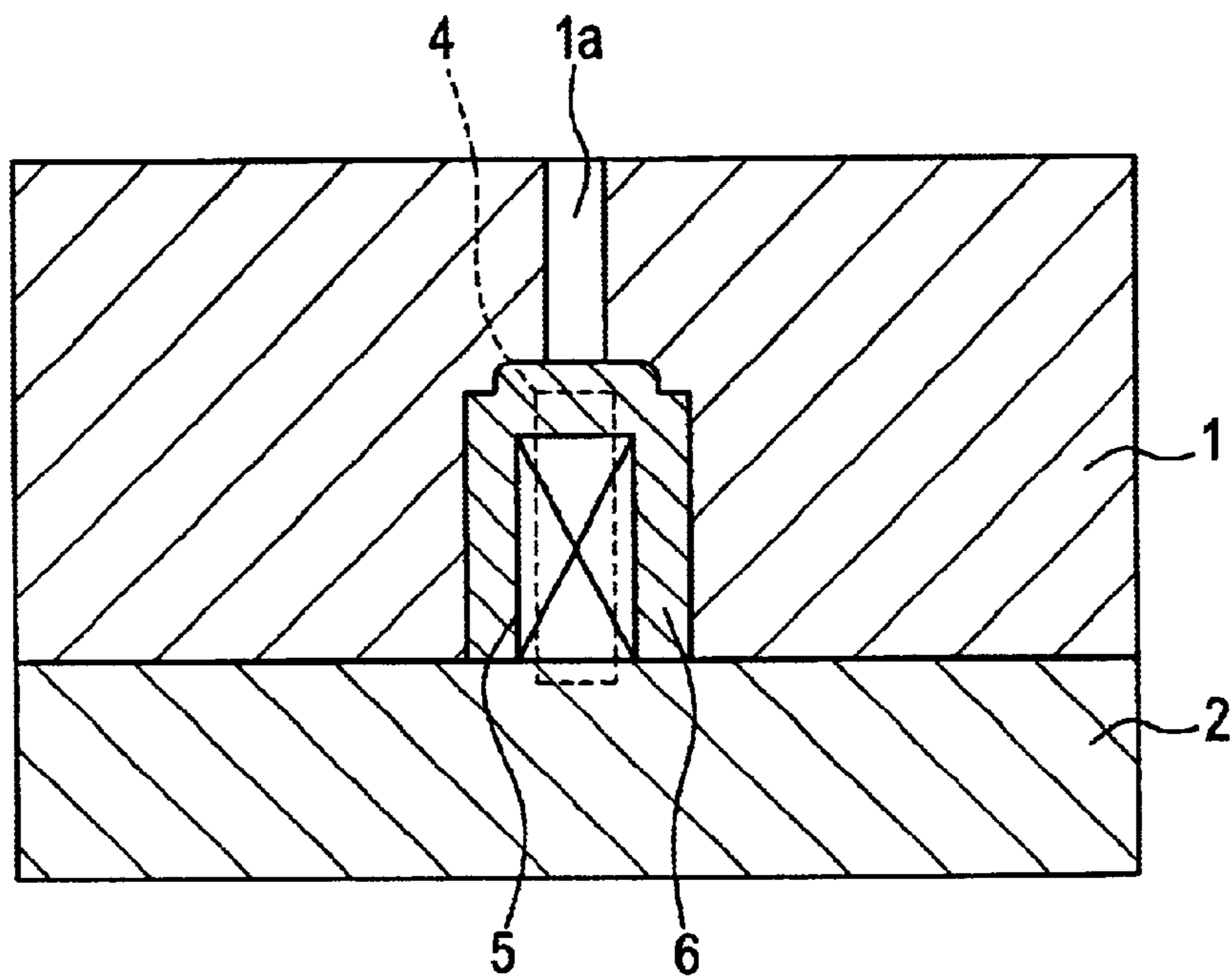
FIG. 7 PRIOR ART
