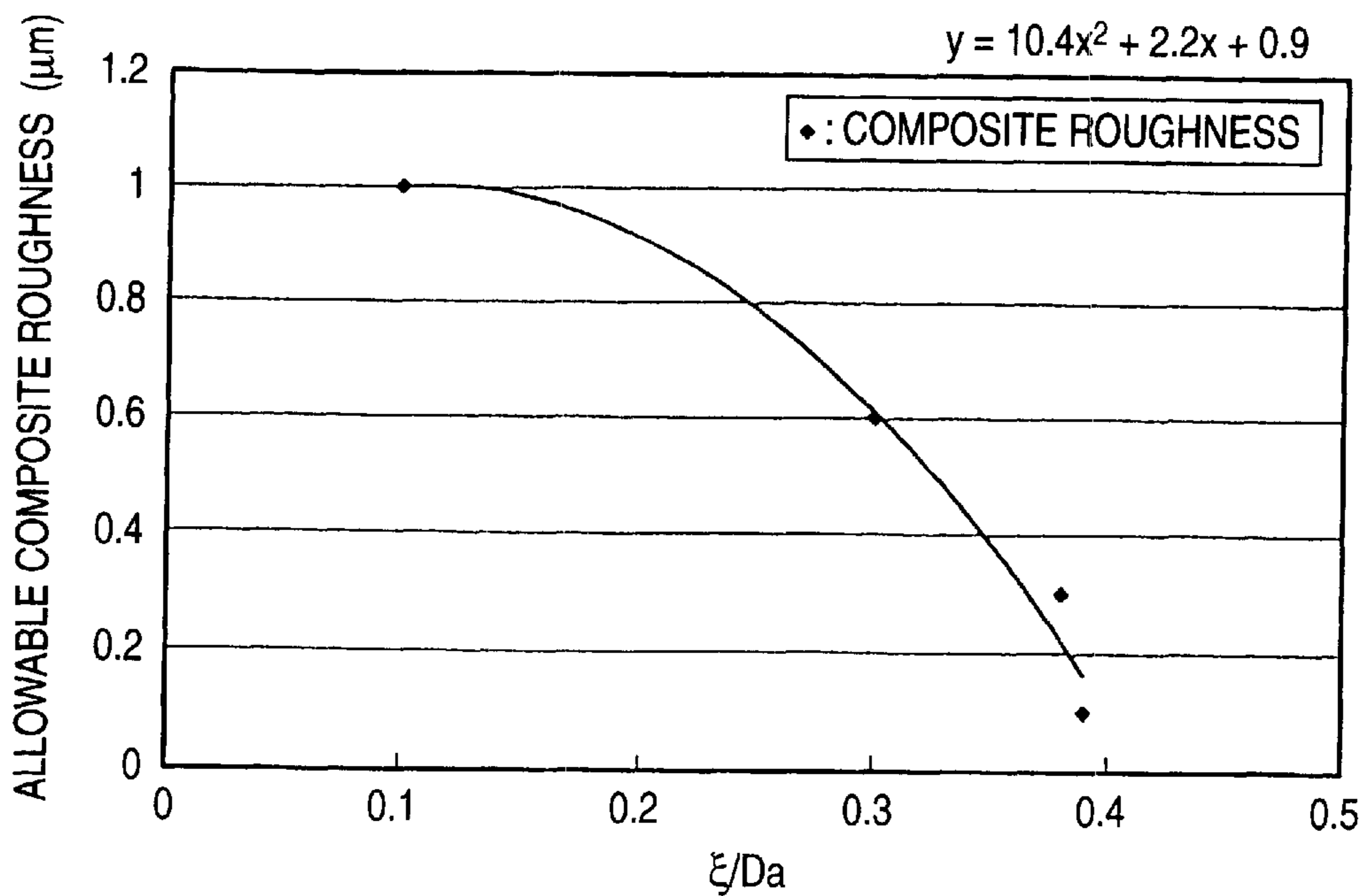
RELATIONSHIP BETWEEN \xi/Da AND ALLOWABLE COMPOSITE ROUGHNESS
