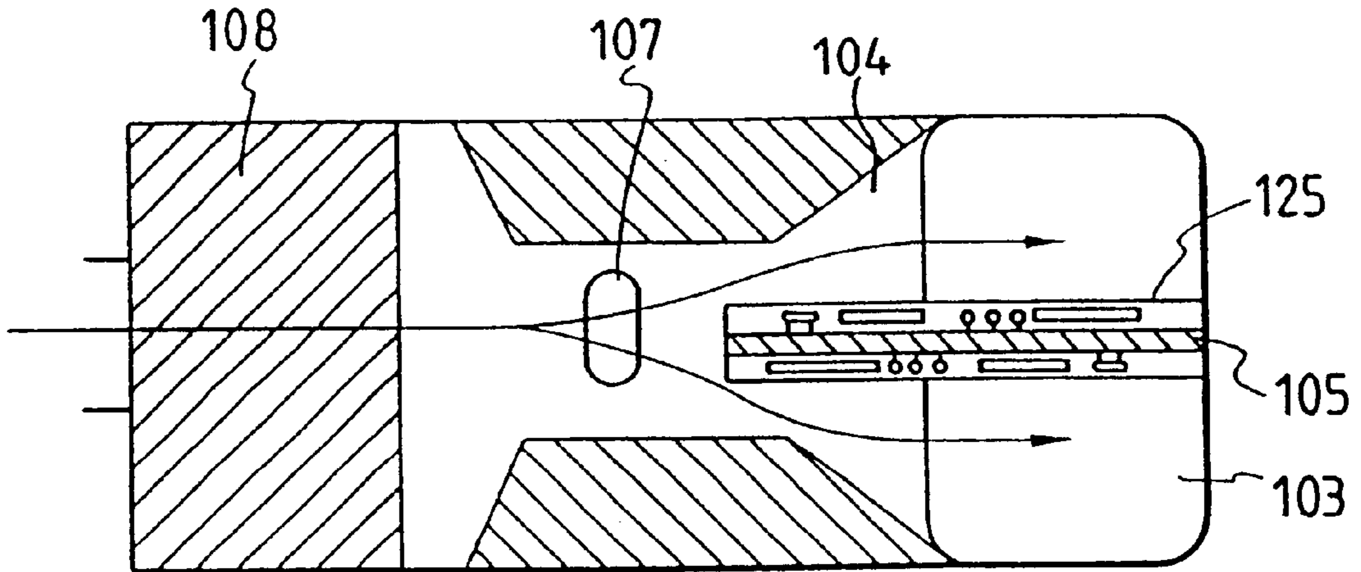
SECTION C-C
