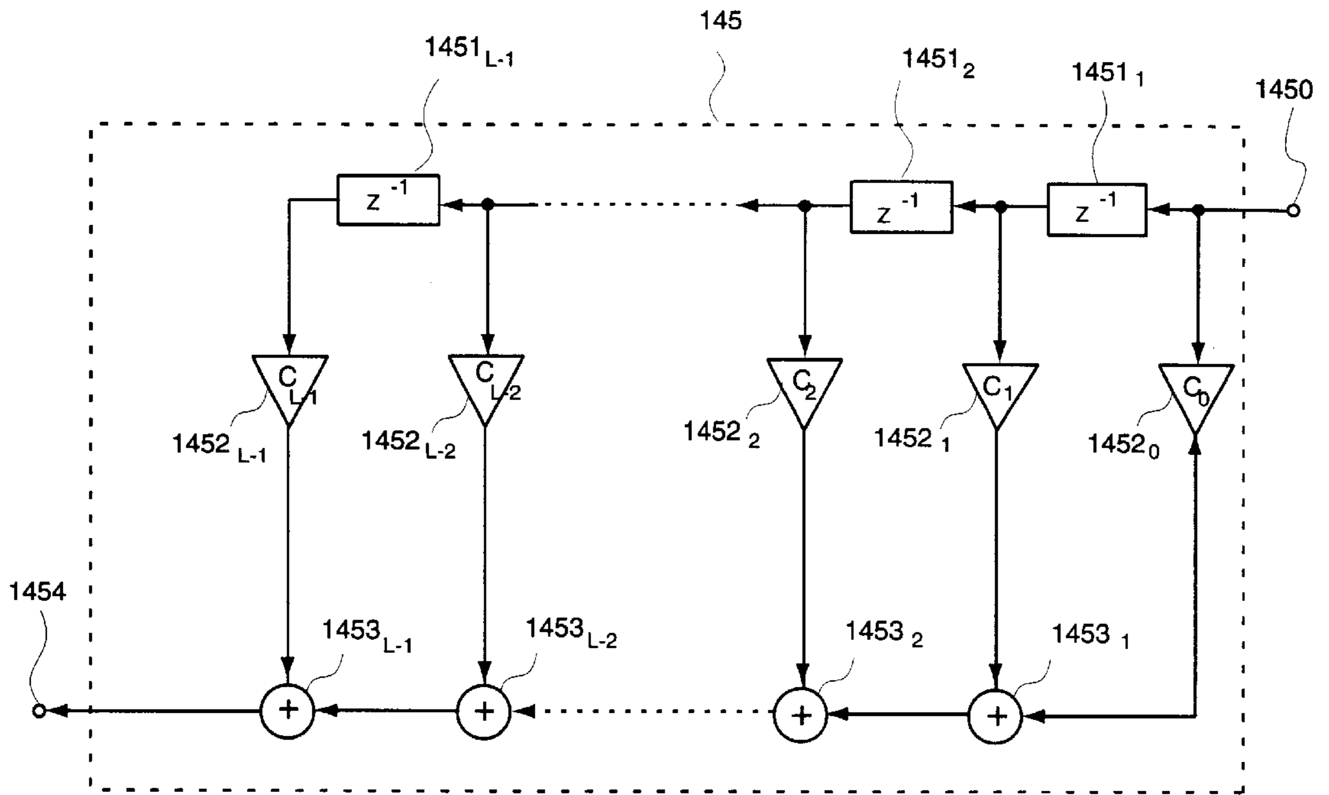
EXAMPLE OF THE FILTER CONFIGURATION
