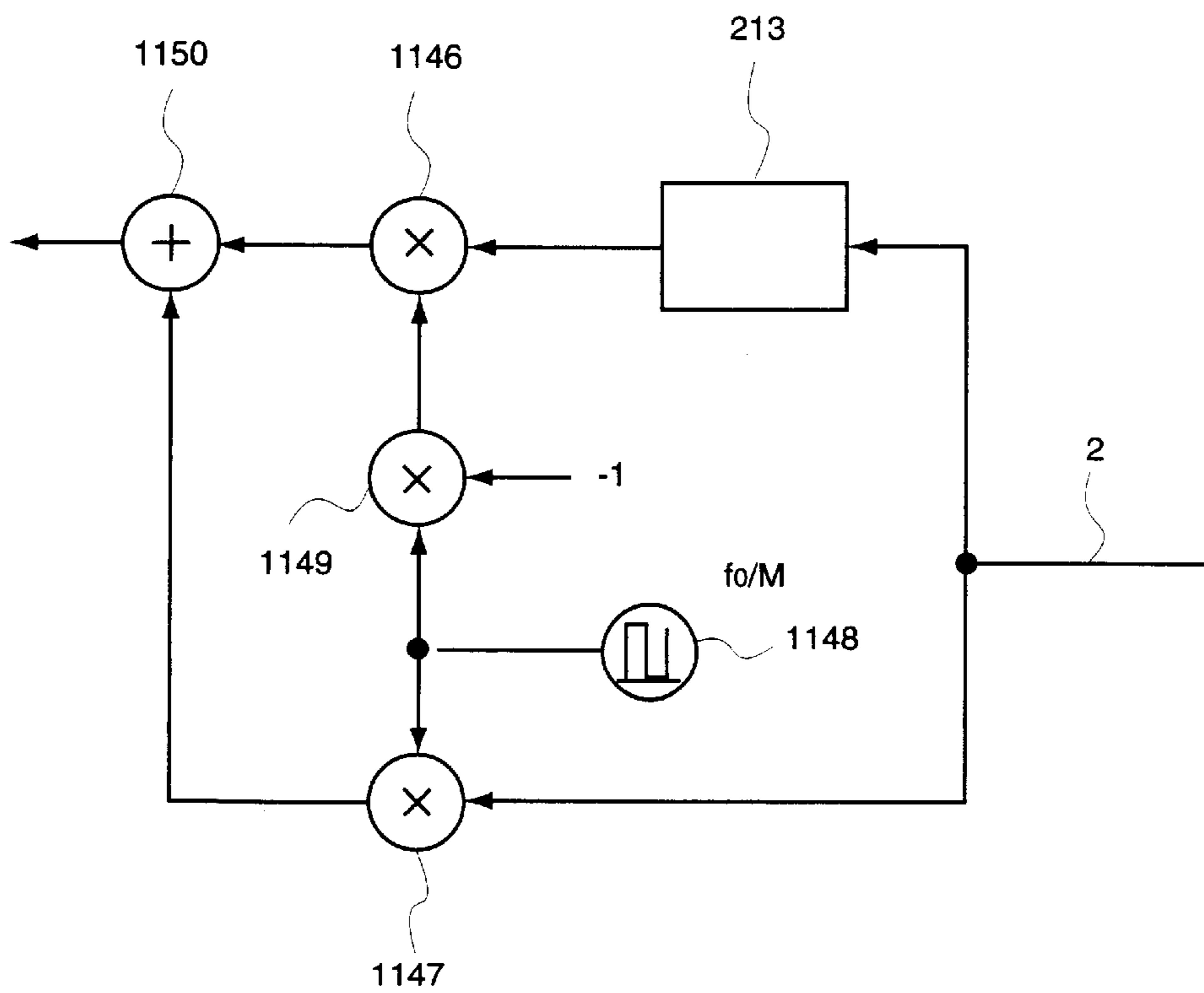
EQUIVALENT CIRCUIT
