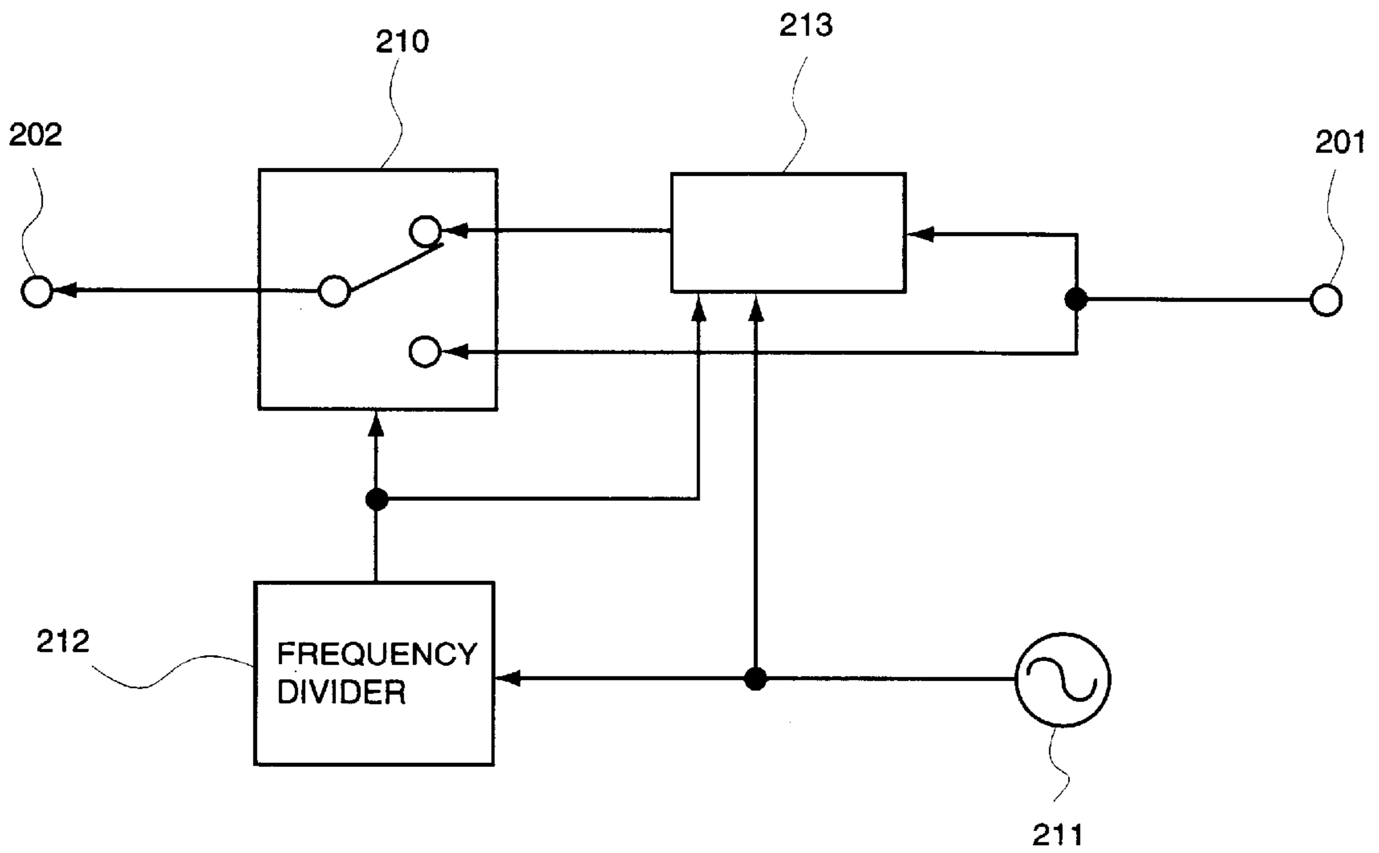
EXAMPLE OF THE PRE-PROCESSING CIRCUIT
