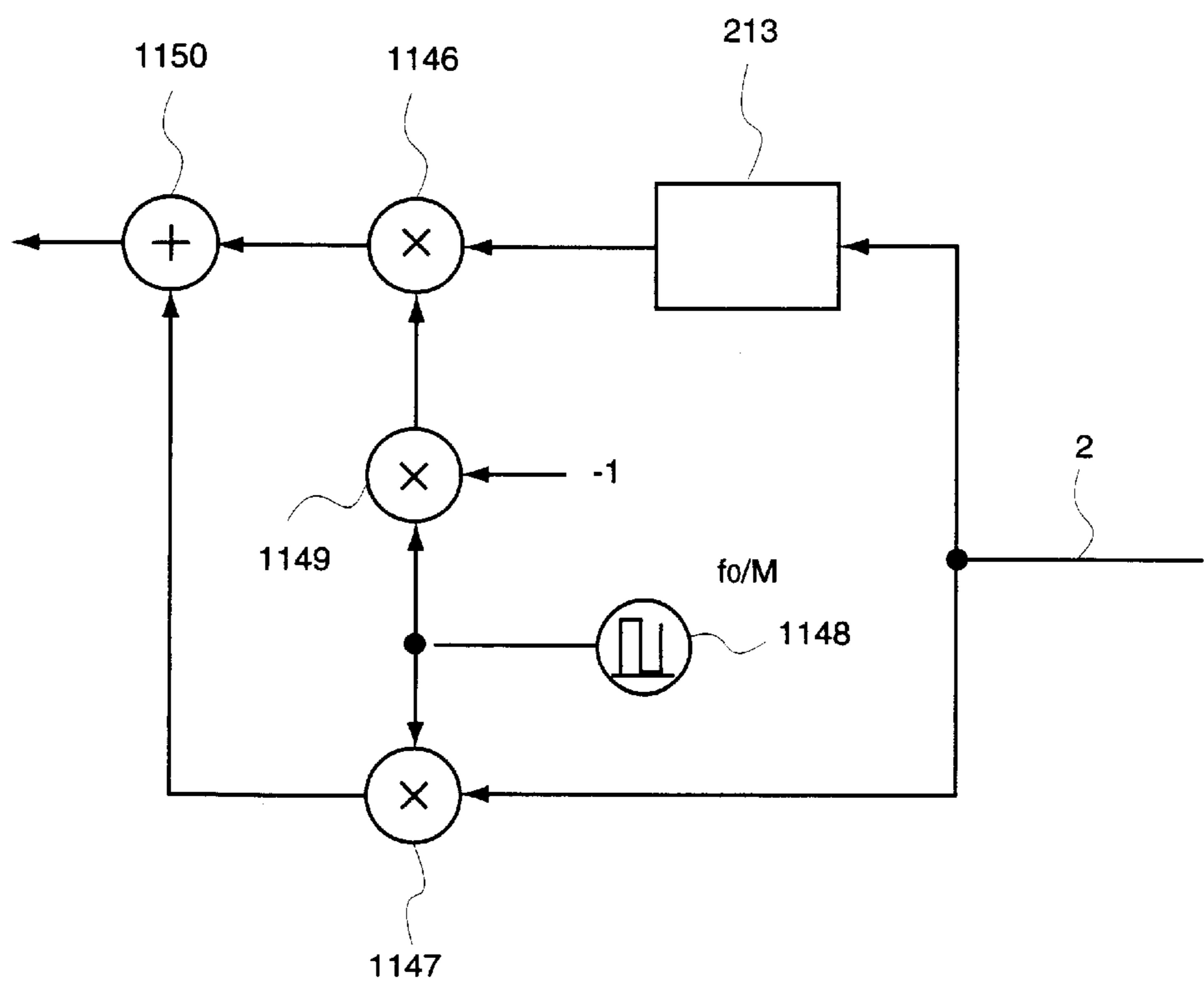
EQUIVALENT CIRCUIT
