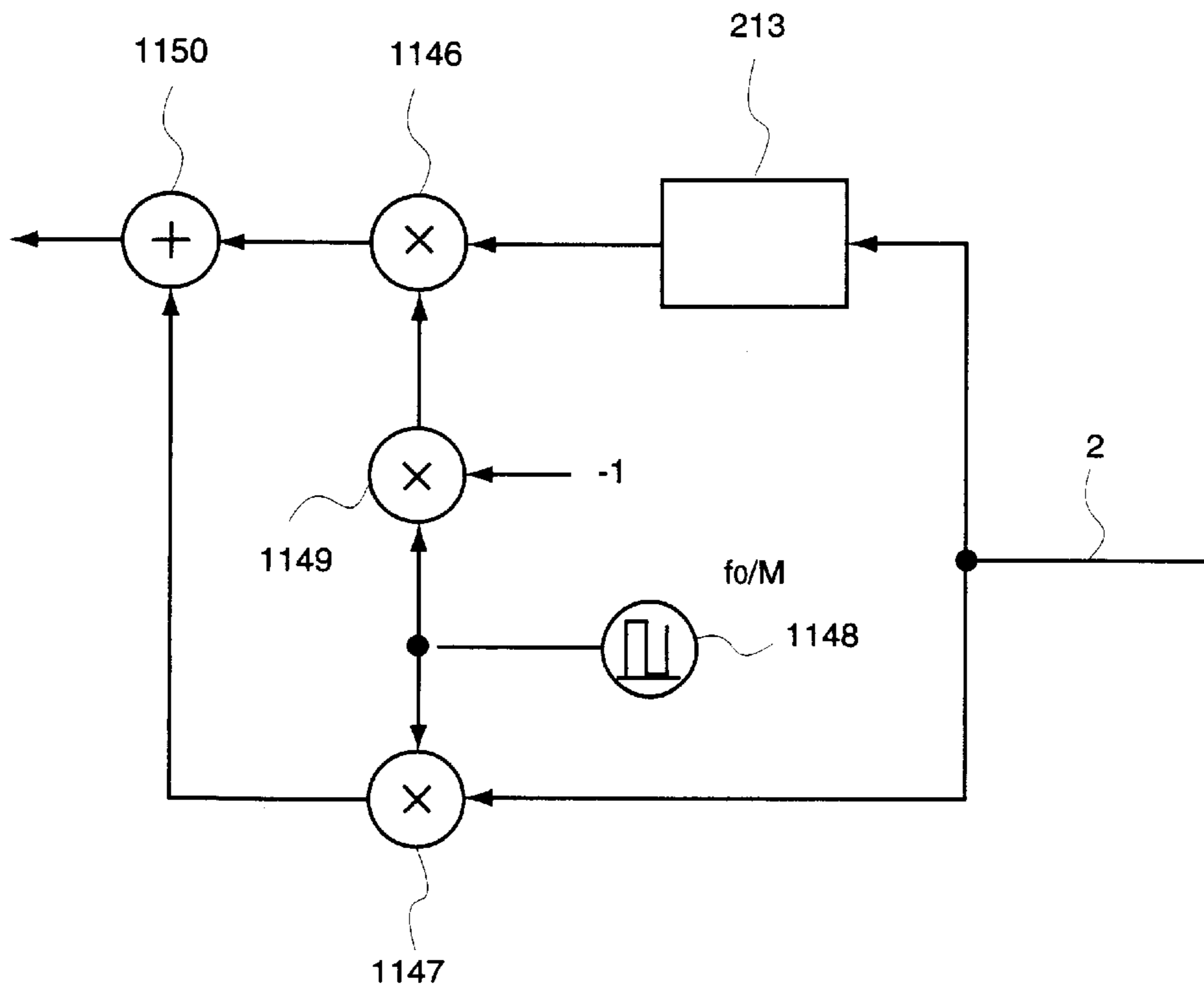
EQUIVALENT CIRCUIT
