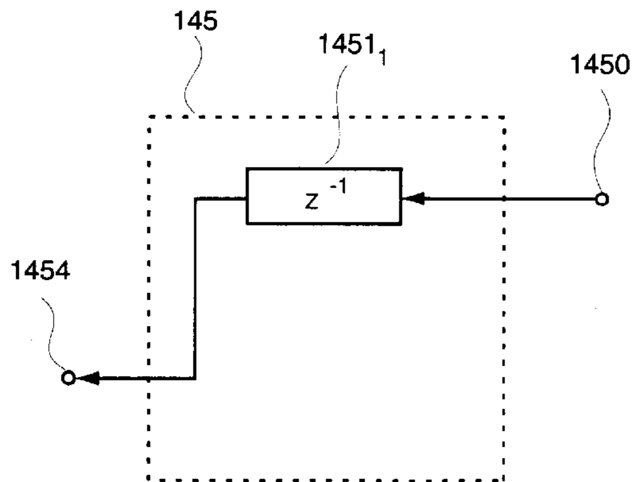
SPECIAL EXAMPLE OF THE FILTER CONFIGURATION
