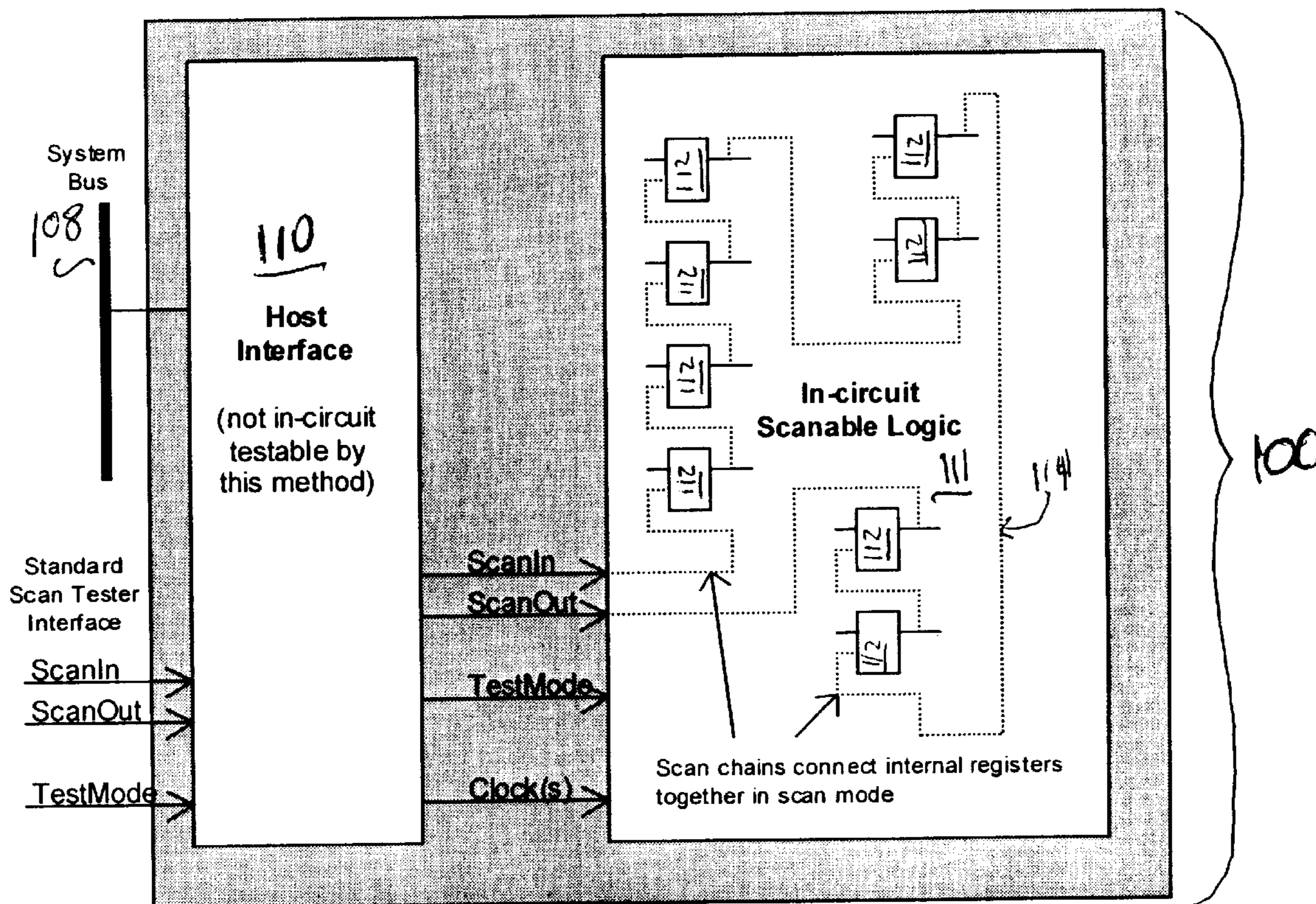
Main Elements of Chip In-Circuit Scan Test Configuration
