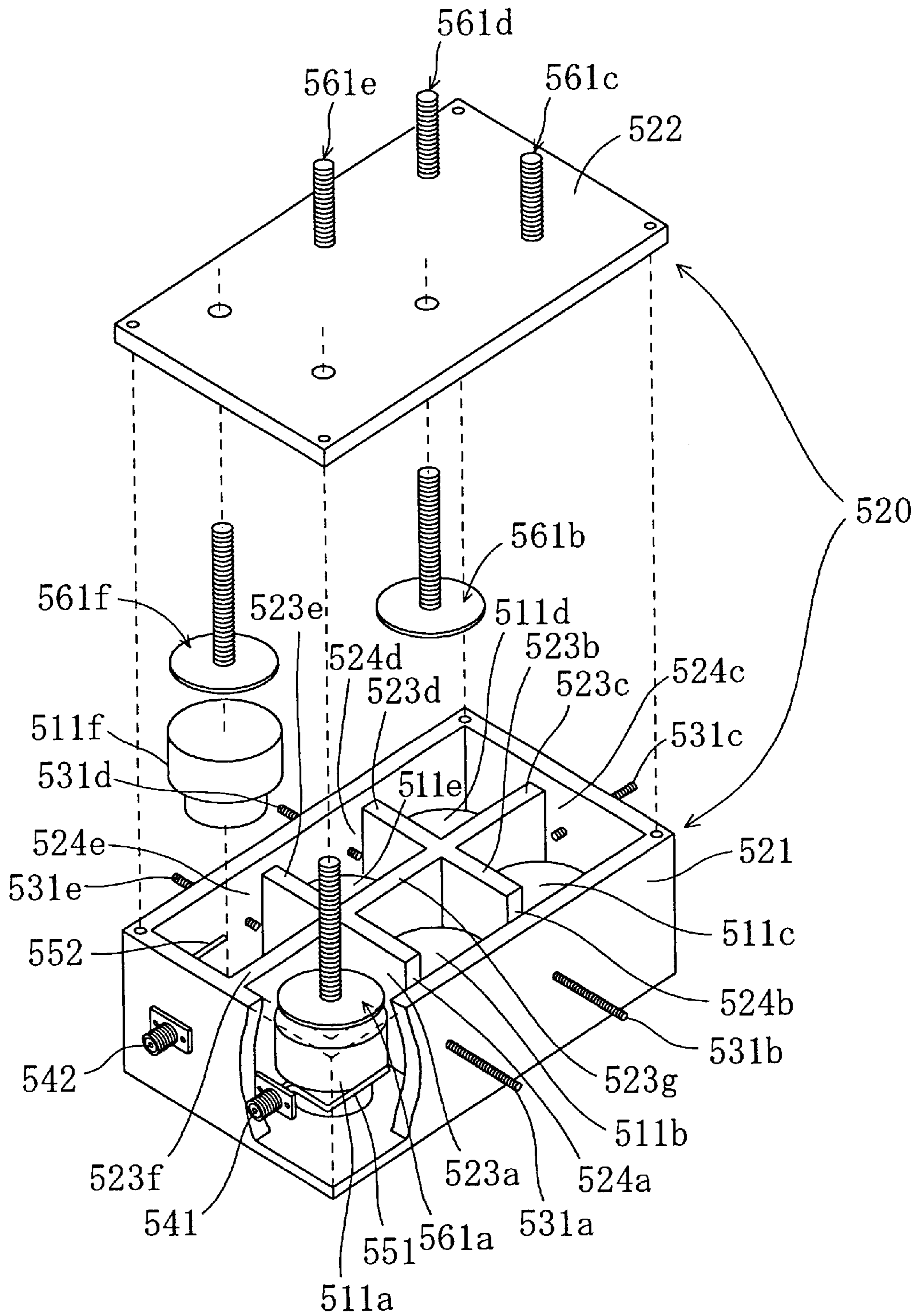
FIG. 21 PRIOR ART
