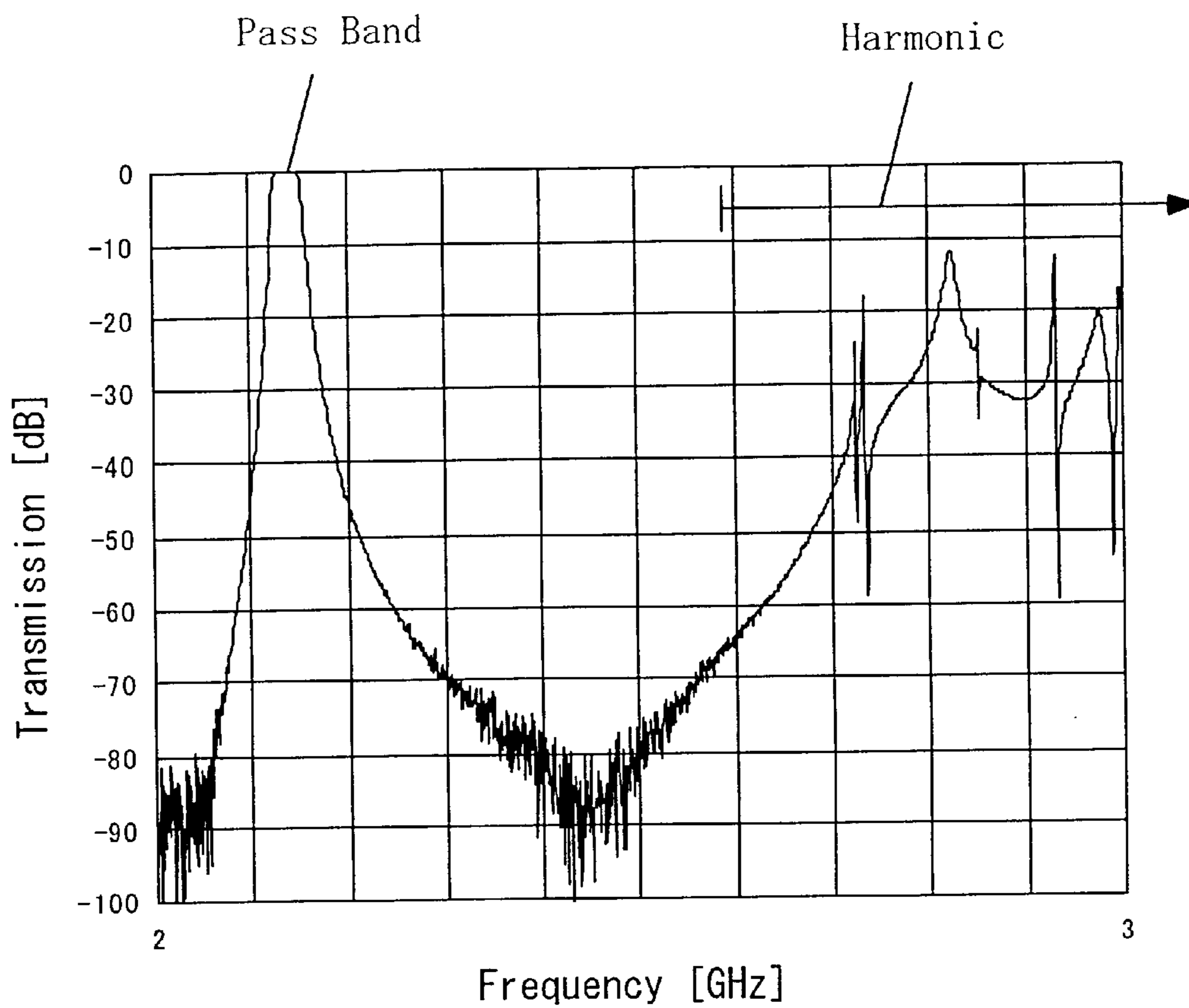
FIG. 25 PRIOR ART
