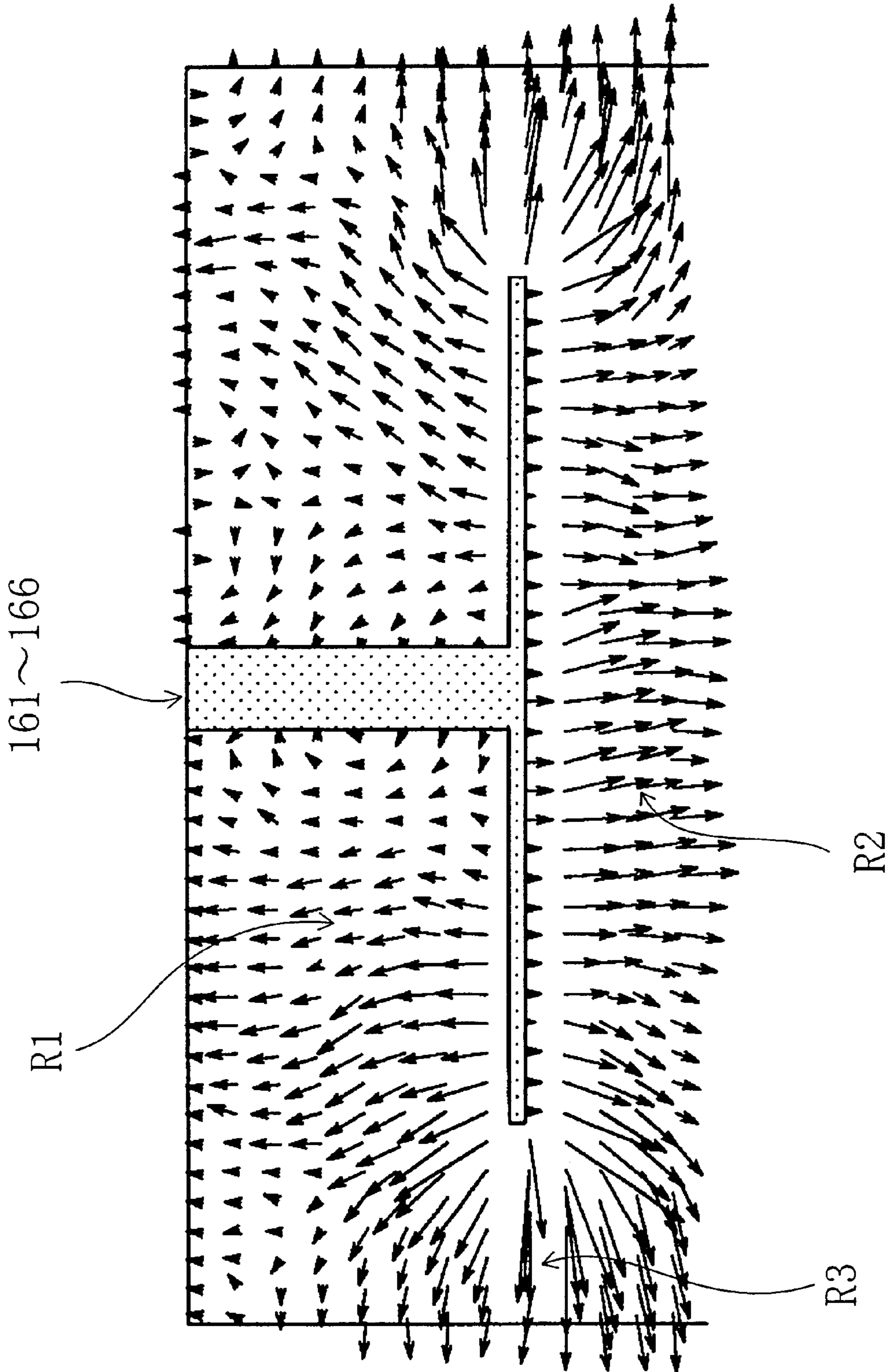
FIG. 22 PRIOR ART
