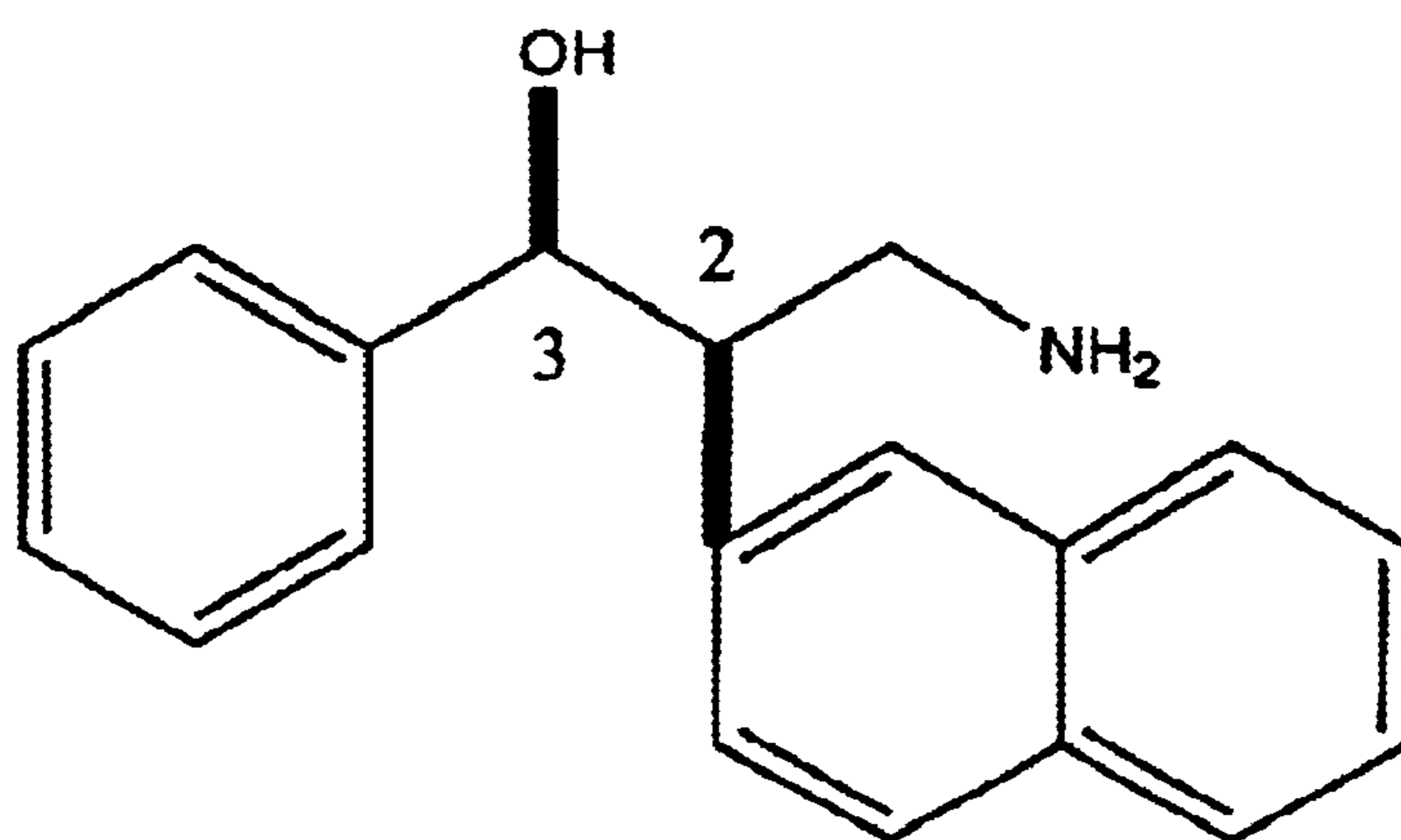
(2R,3S) -3-hydroxy-2-(2'-naphthyl)-3-phenylpropylamine
