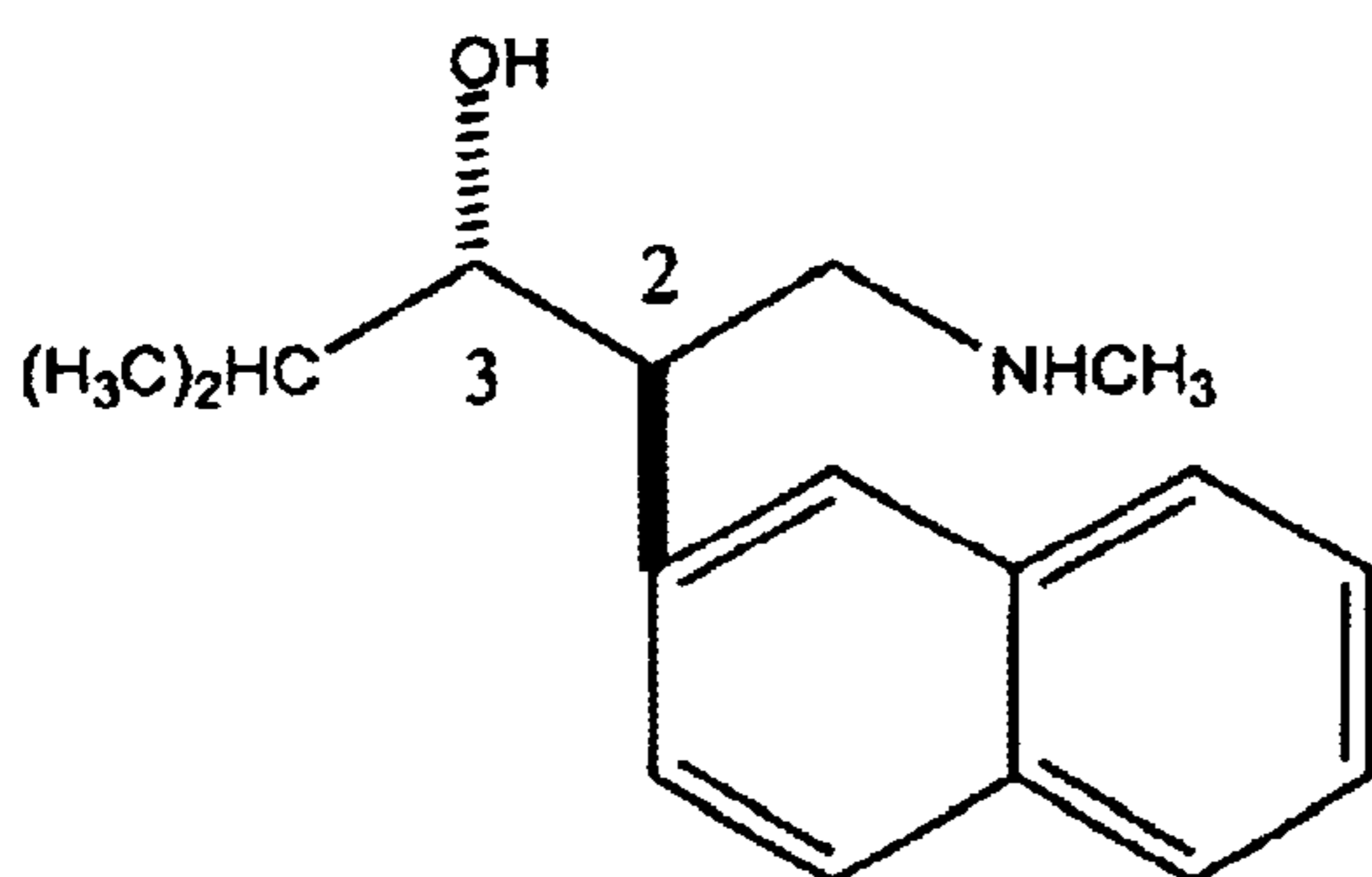
(2 R ,3 S )- N -methyl-3-hydroxy-4-methyl-2-(2'-naphthyl)pentylamine
