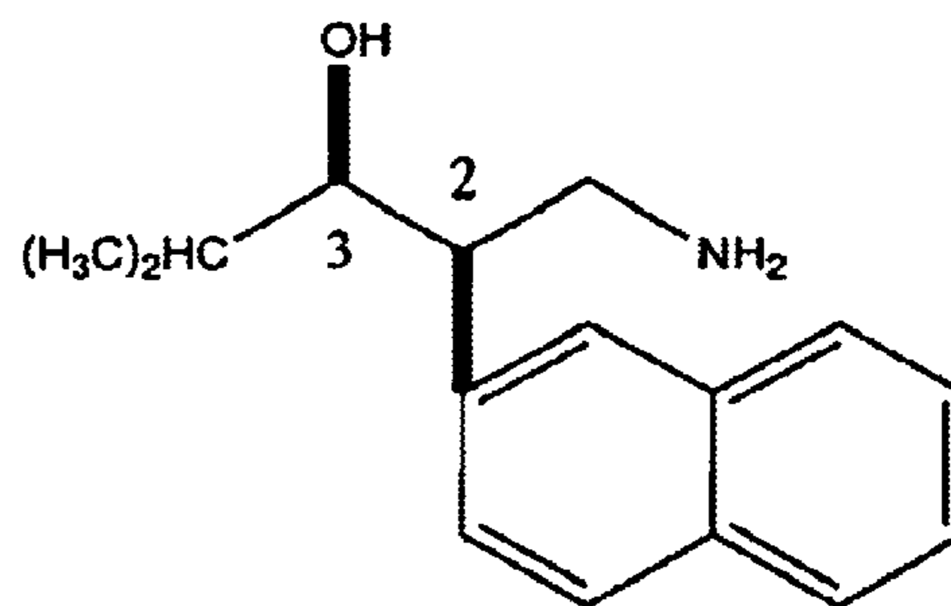
(2 R ,3 R )-3-hydroxy-4-methyl-2-(2'-naphthyl)pentylamine
