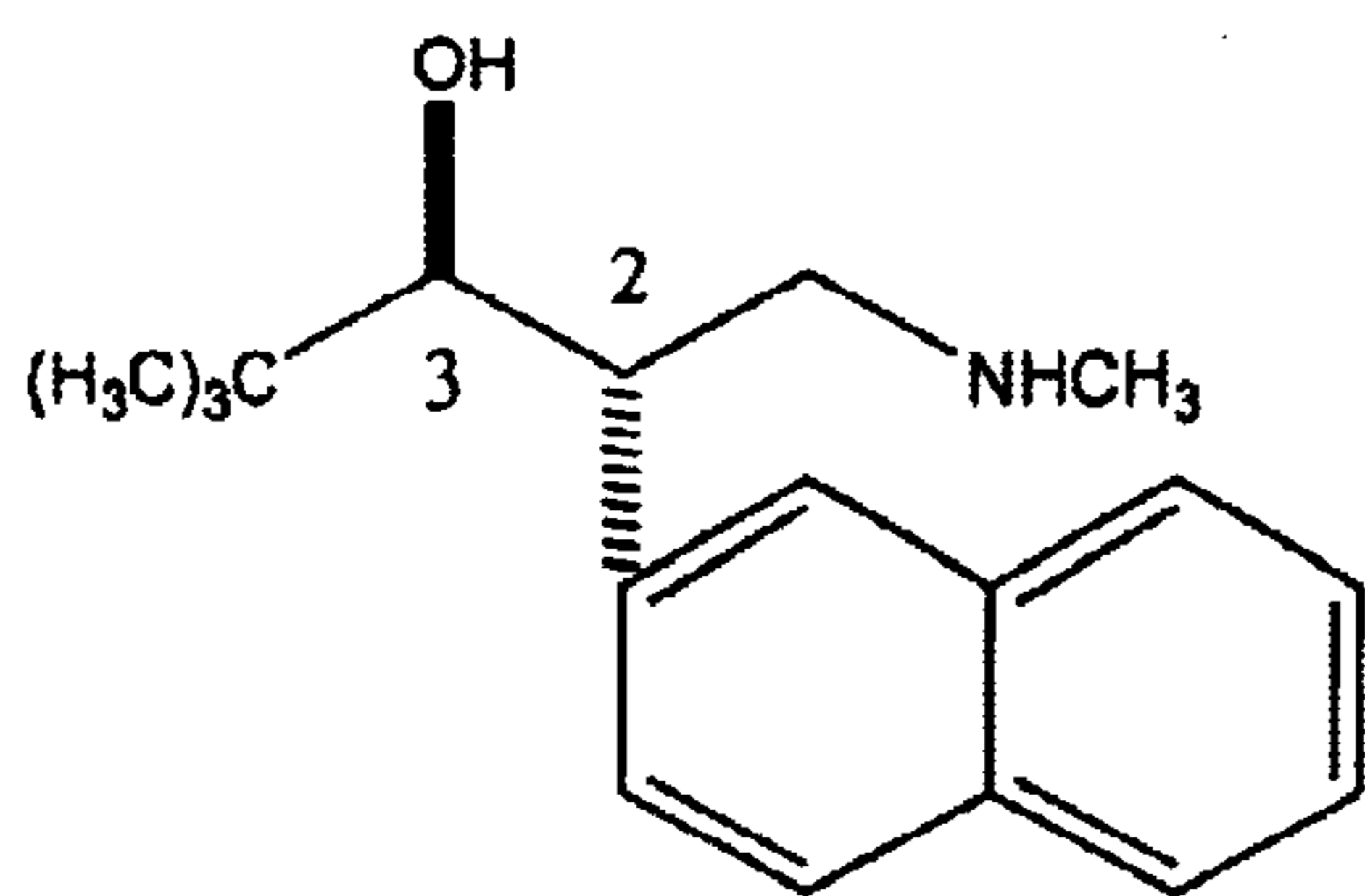
(2 S ,3 S )- N -methyl-3-hydroxy-4,4-dimethyl-2-(2'-naphthyl)pentylamine
