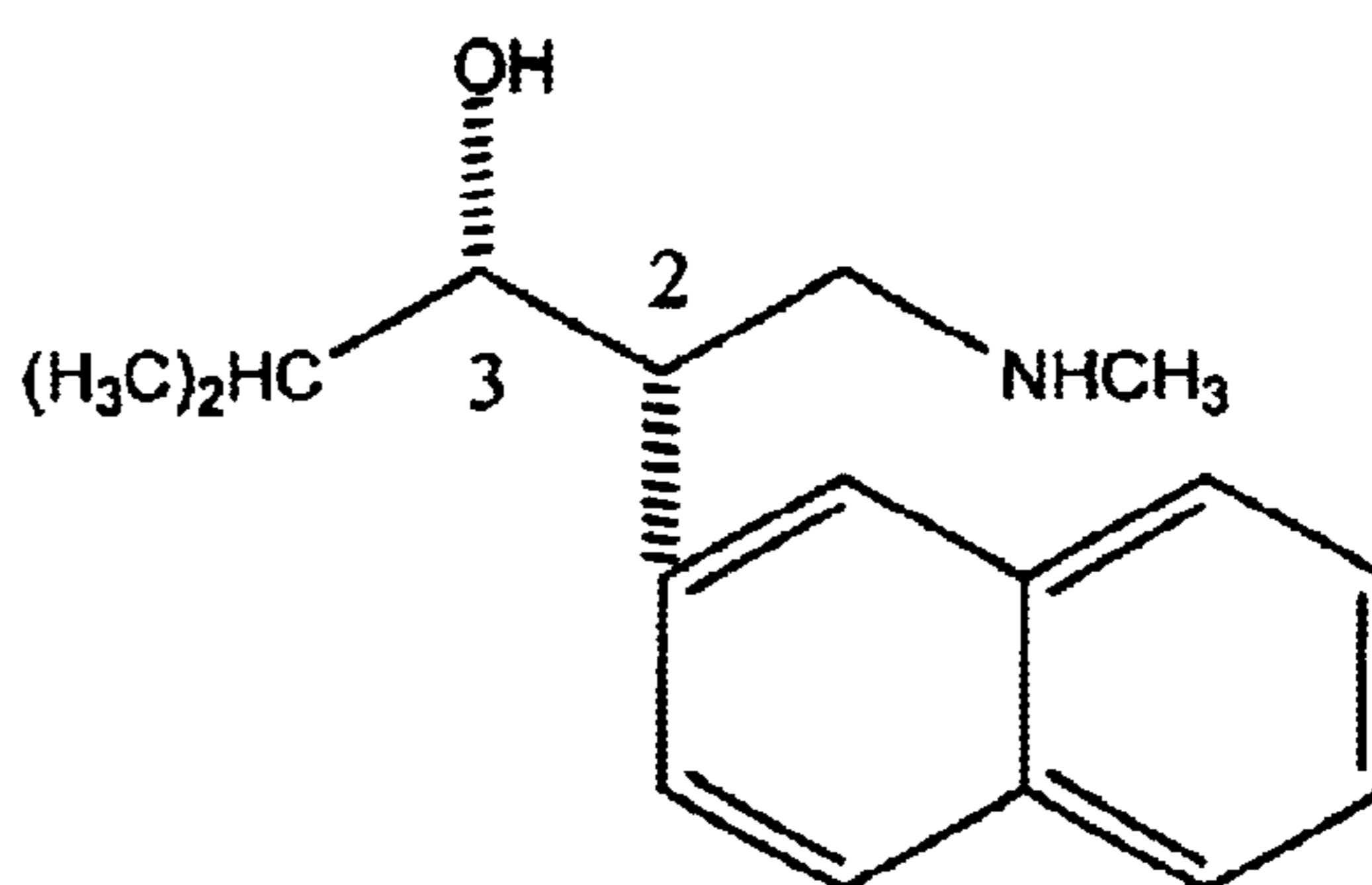
(2 S ,3 S )- N -methyl-3-hydroxy-4-methyl-2-(2'-naphthyl)pentylamine
