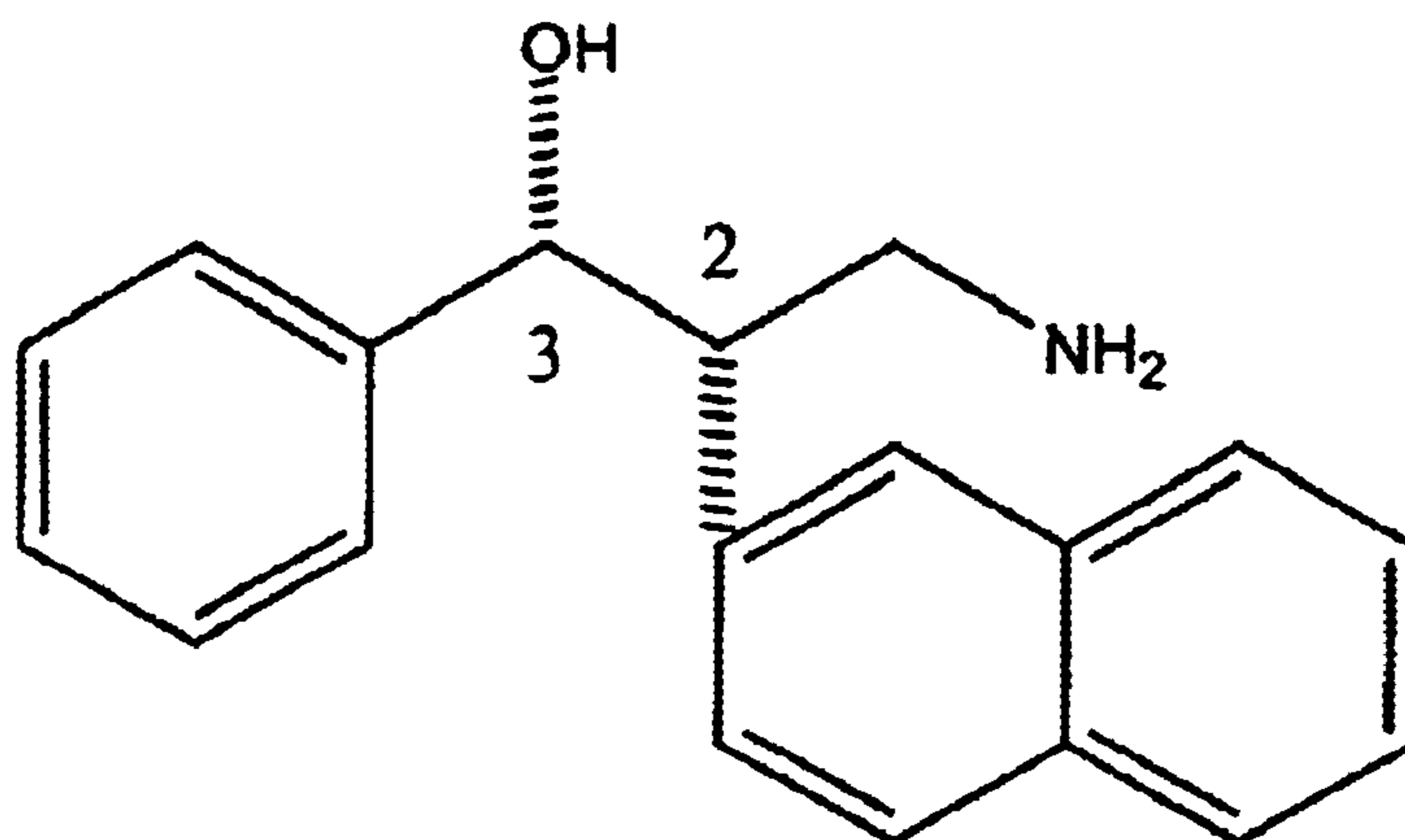
(2S,3R) -3-hydroxy-2-(2'-naphthyl)-3-phenylpropylamine
