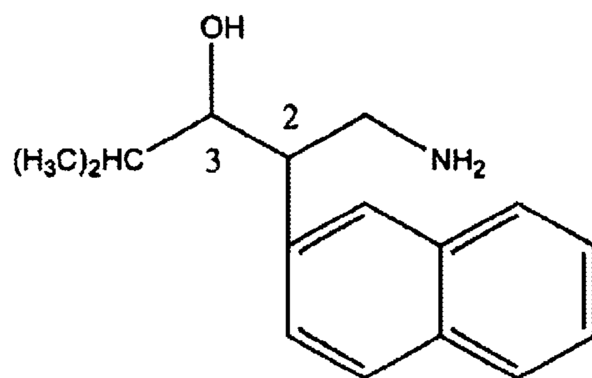
3-hydroxy-4-methyl-2-(2'-naphthyl)pentylamine
