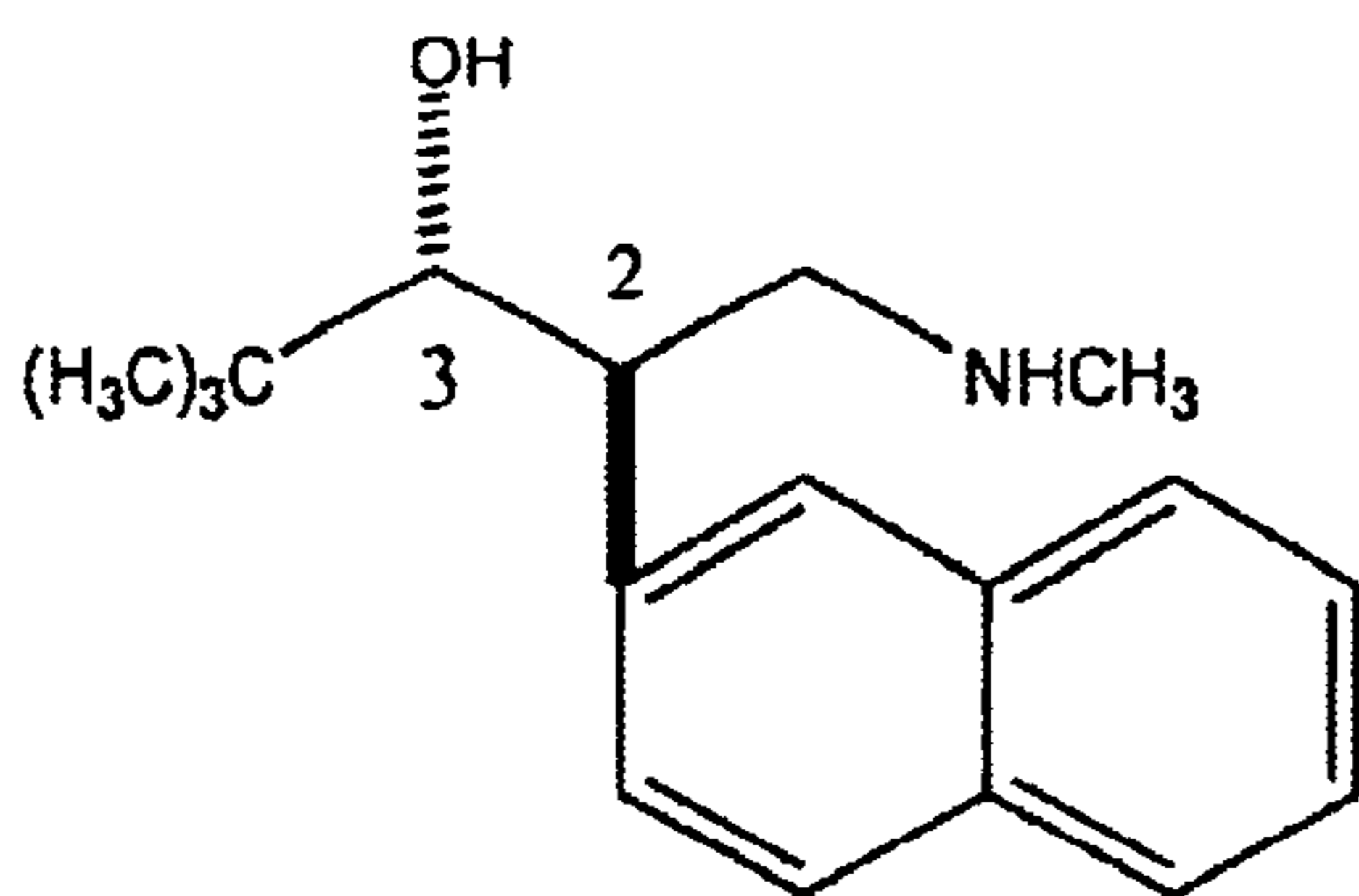
(2 R ,3 R )- N -methyl-3-hydroxy-4,4-dimethyl-2-(2'-naphthyl)pentylamine
