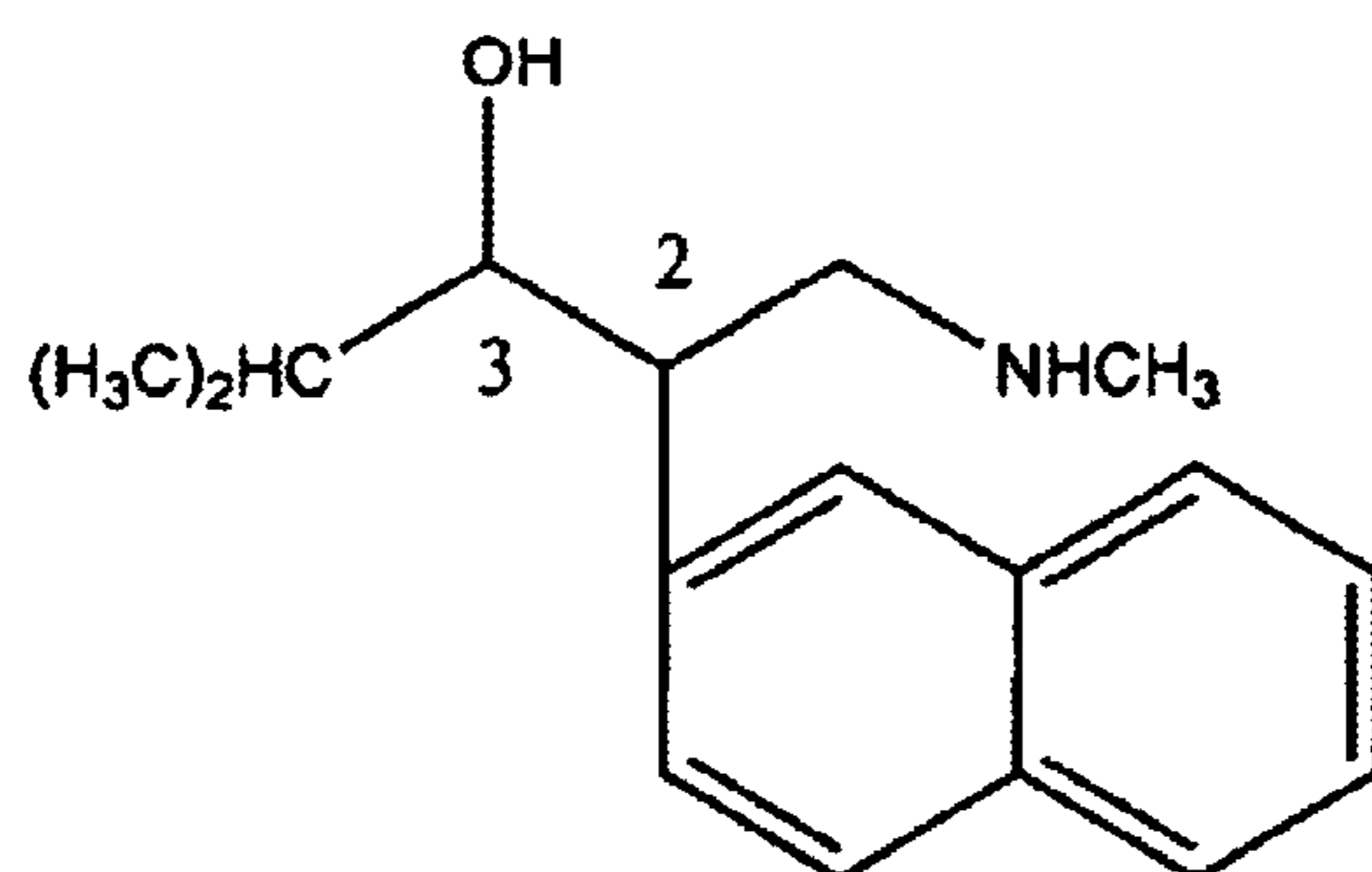
N -methyl-3-hydroxy-4-methyl-2-(2'-naphthyl)pentylamine
