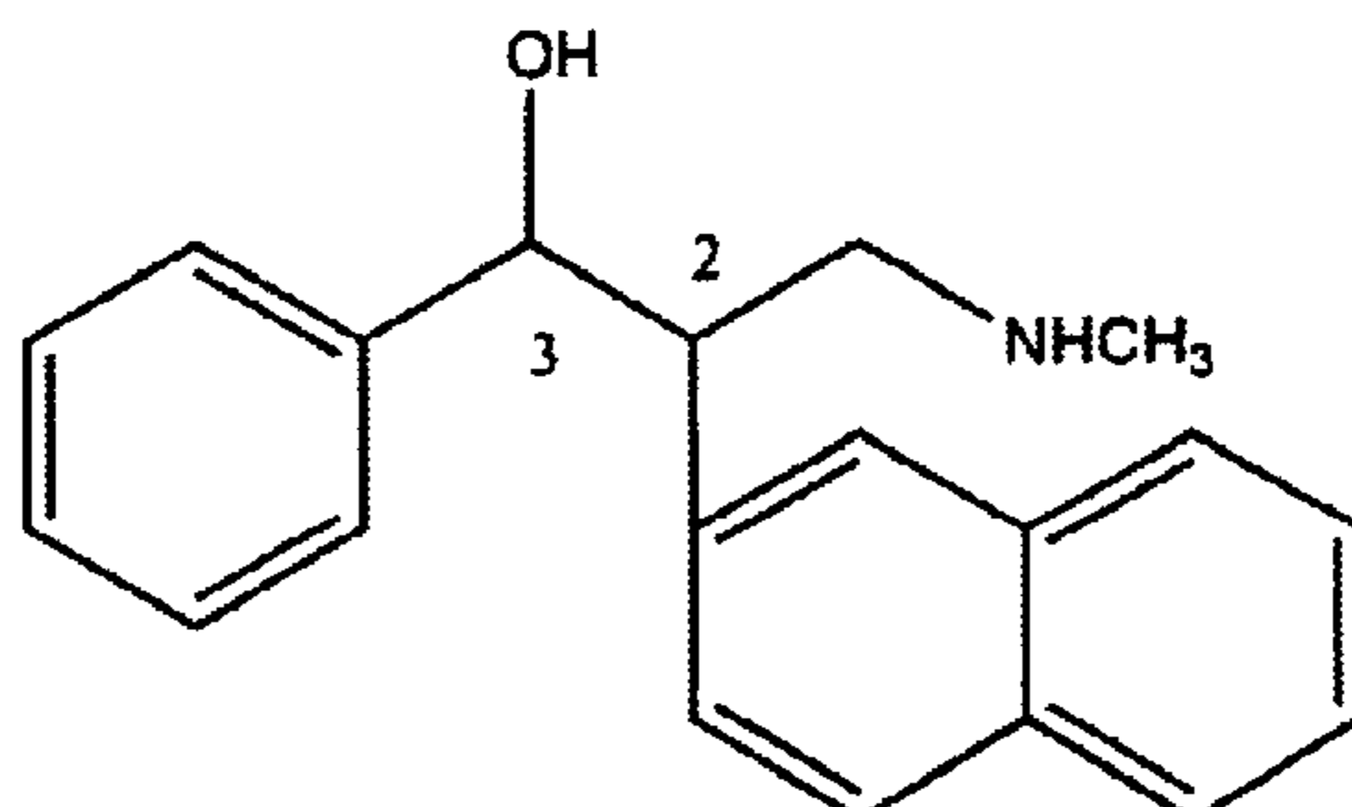
N -methyl-3-hydroxy-2-(2'-naphthyl)-3-phenylpropylamine
