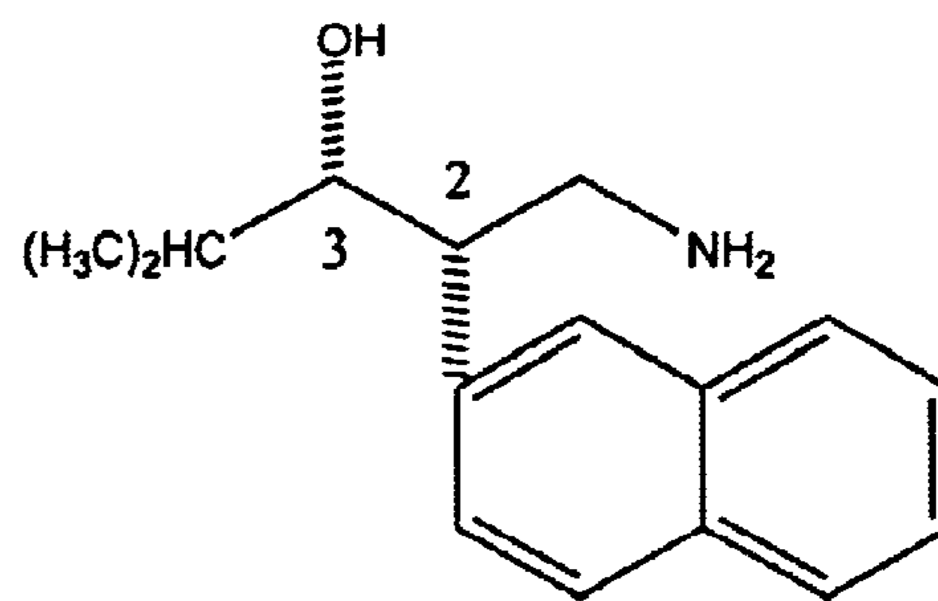
(2 S ,3 S )-3-hydroxy-4-methyl-2-(2'-naphthyl)pentylamine
