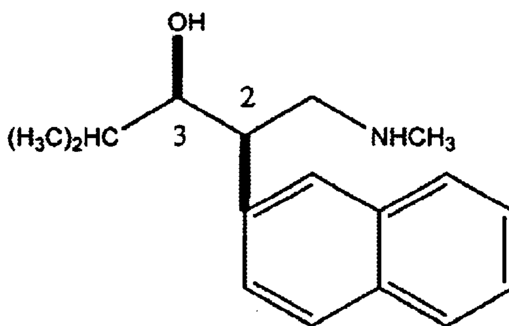
(2 R ,3 R )- N -methyl-3-hydroxy-4-methyl-2-(2'-naphthyl)pentylamine
