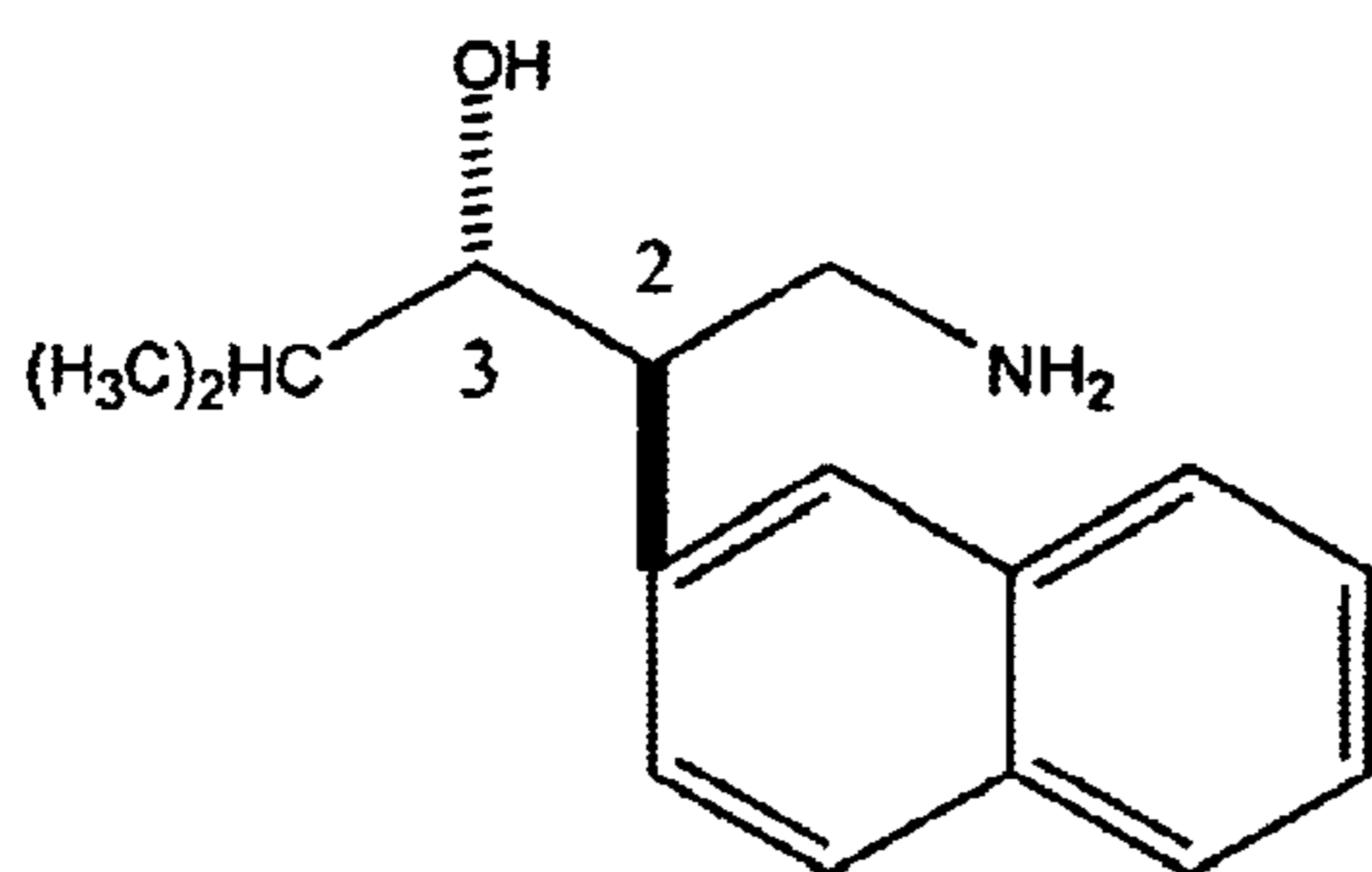
(2 R ,3 S )-3-hydroxy-4-methyl-2-(2'-naphthyl)pentylamine
