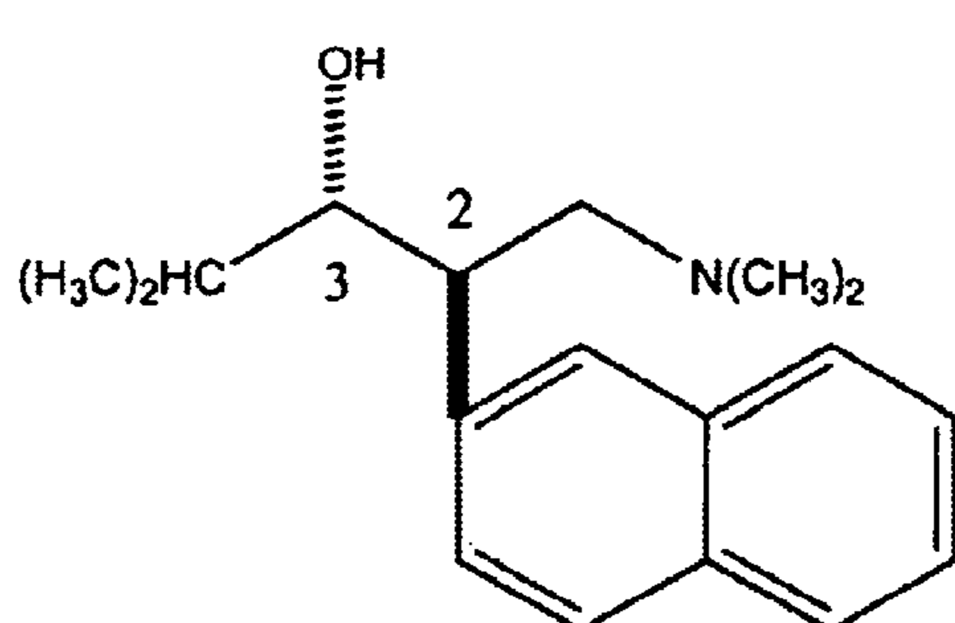
(2R,3S) - N,N -dimethyl-3-hydroxy-4-methyl-2-(2'-naphthyl)pentylamine
