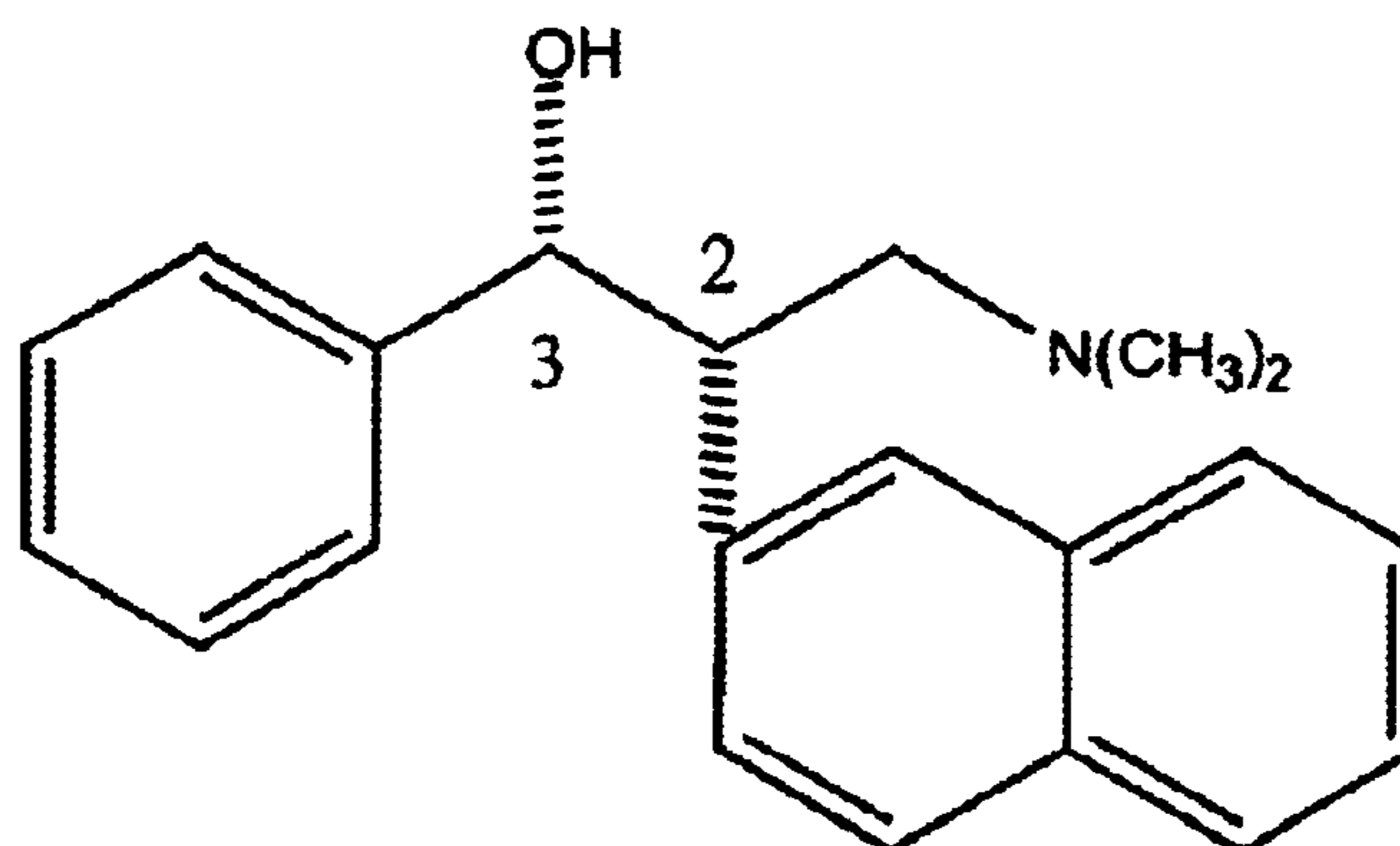
(2S,3R) - N,N -dimethyl-3-hydroxy-2-(2'-naphthyl)-3-phenylpropylamine
