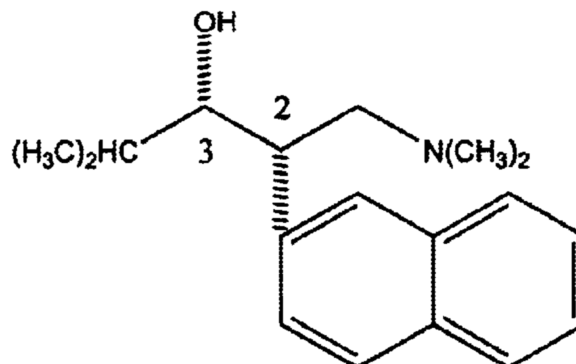
(2S,3S) - N,N -dimethyl-3-hydroxy-4-methyl-2-(2'-naphthyl)pentylamine
