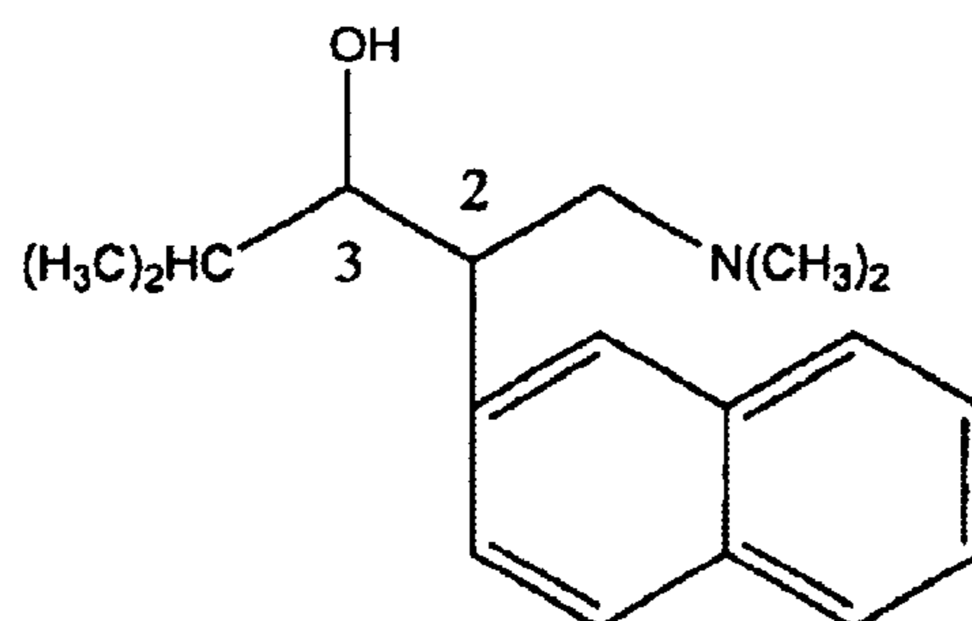
N,N -dimethyl-3-hydroxy-4-methyl-2-(2'-naphthyl)pentylamine
