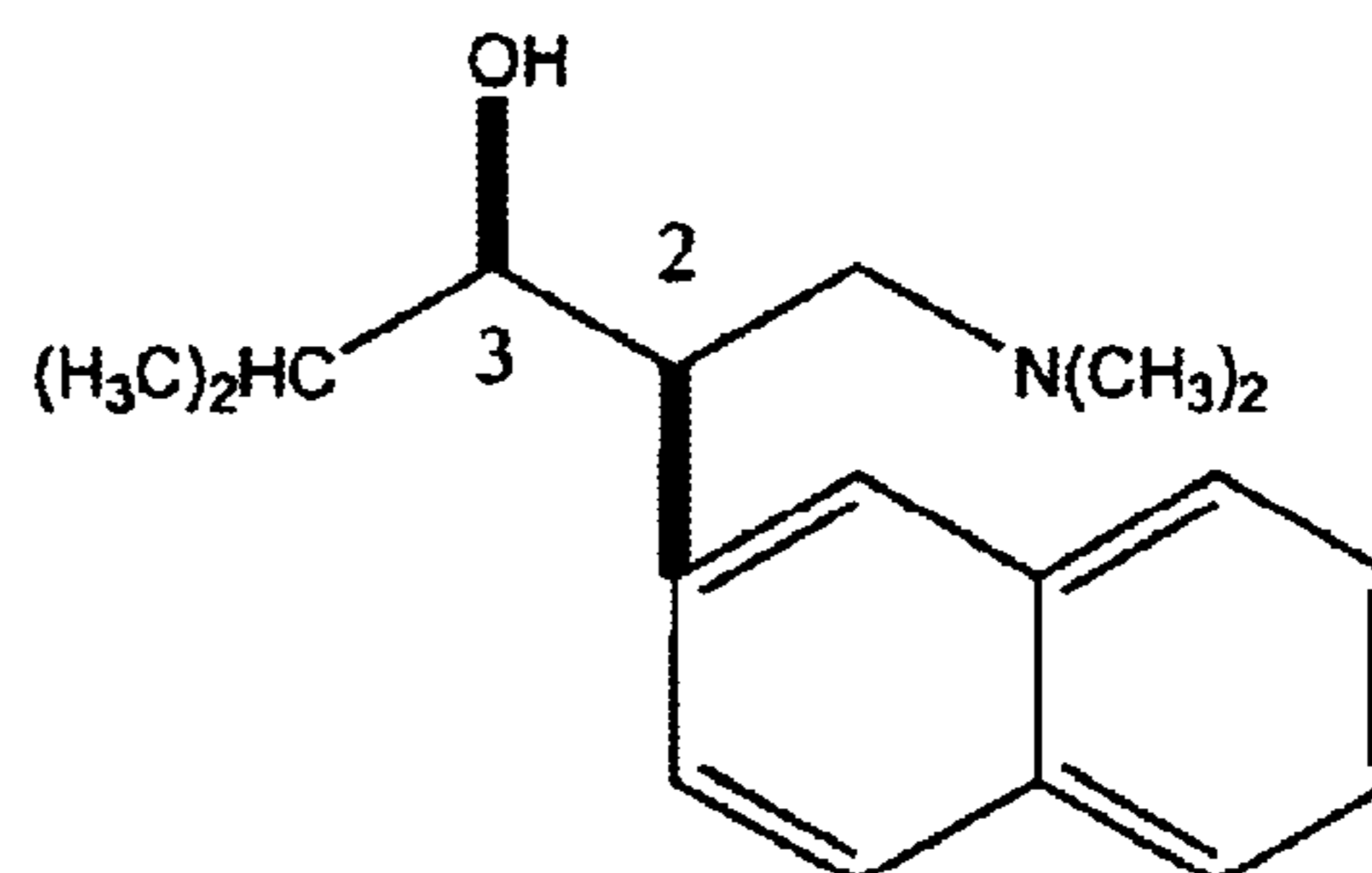
(2R,3R) - N,N -dimethyl-3-hydroxy-4-methyl-2-(2'-naphthyl)pentylamine
