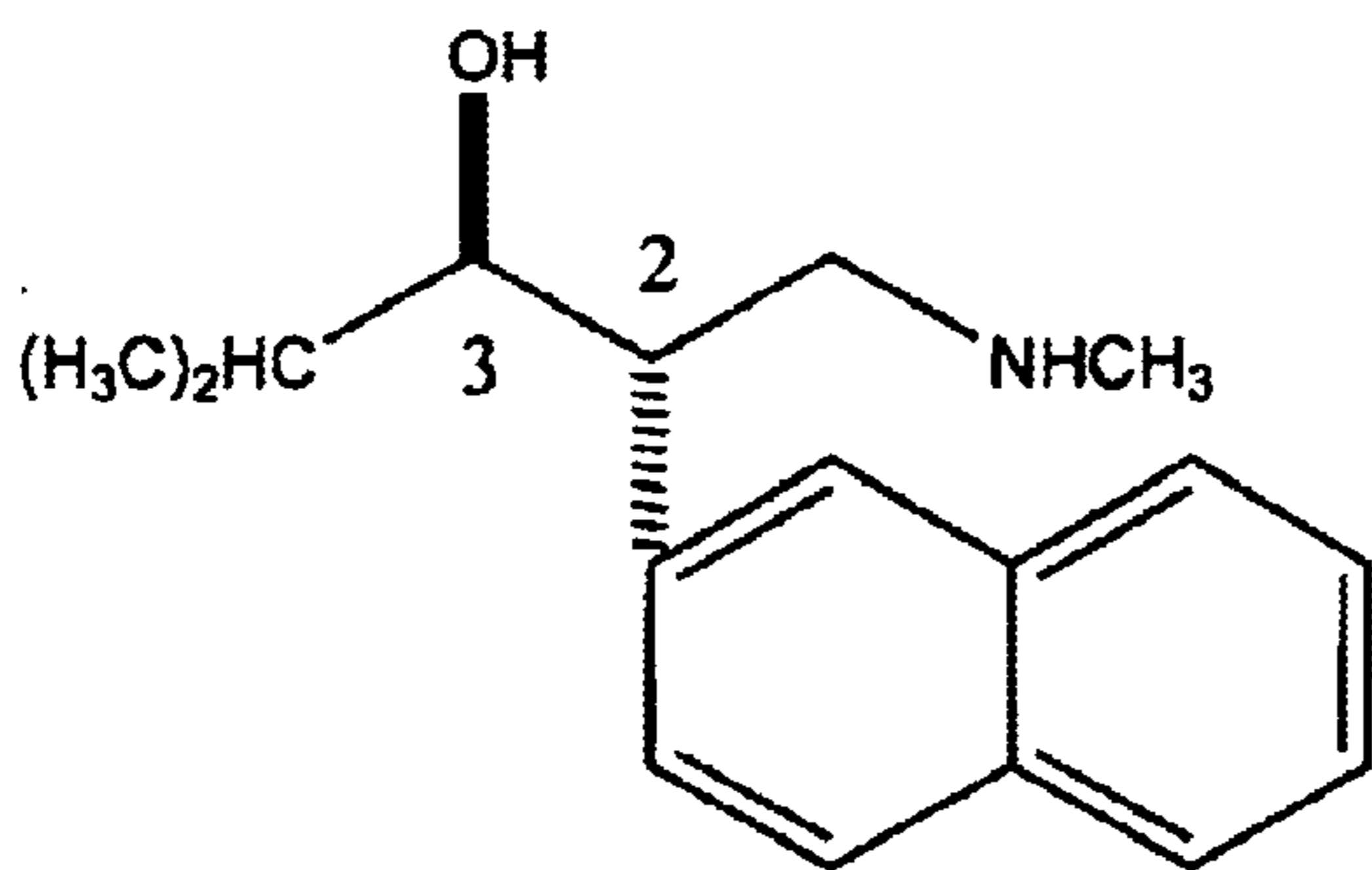
(2 S ,3 R )- N -methyl-3-hydroxy-4-methyl-2-(2'-naphthyl)pentylamine
