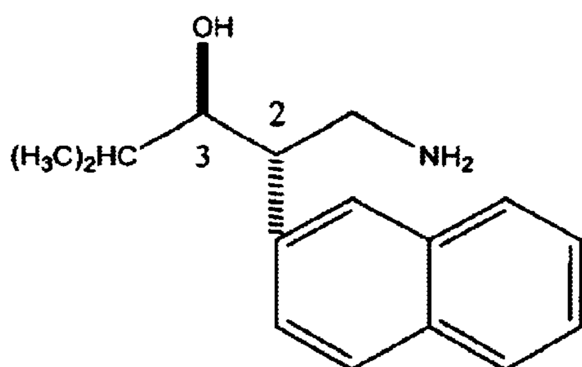
(2 S ,3 R )-3-hydroxy-4-methyl-2-(2'-naphthyl)pentylamine
