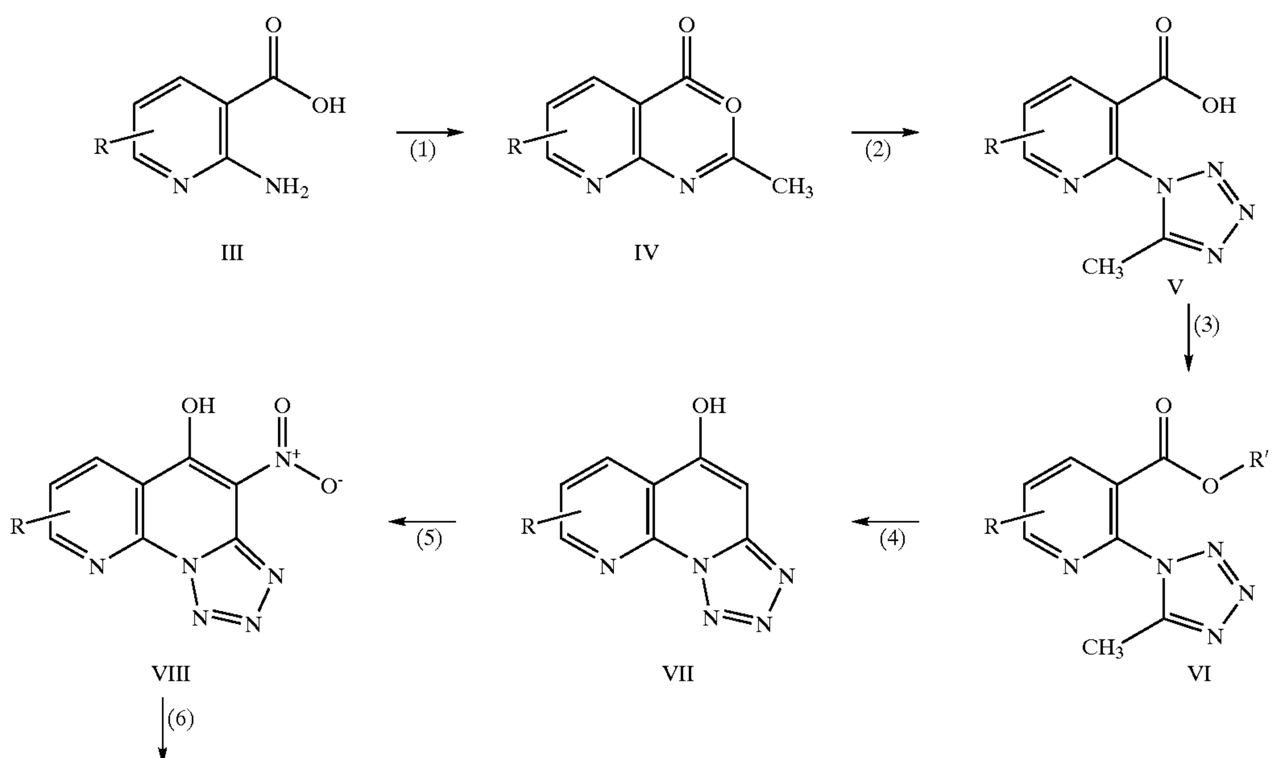
Reaction Scheme I
