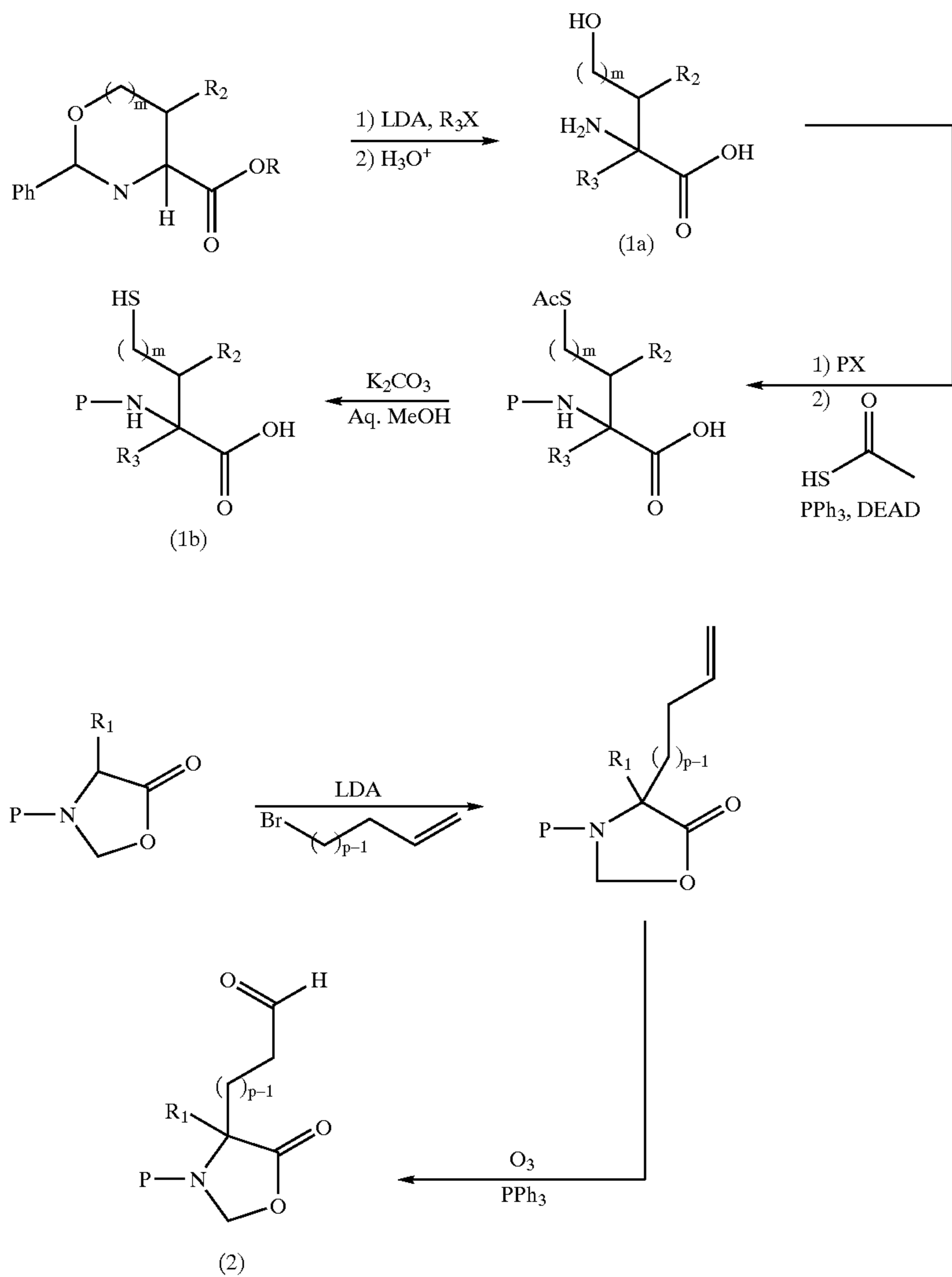
Reaction Scheme (14)
