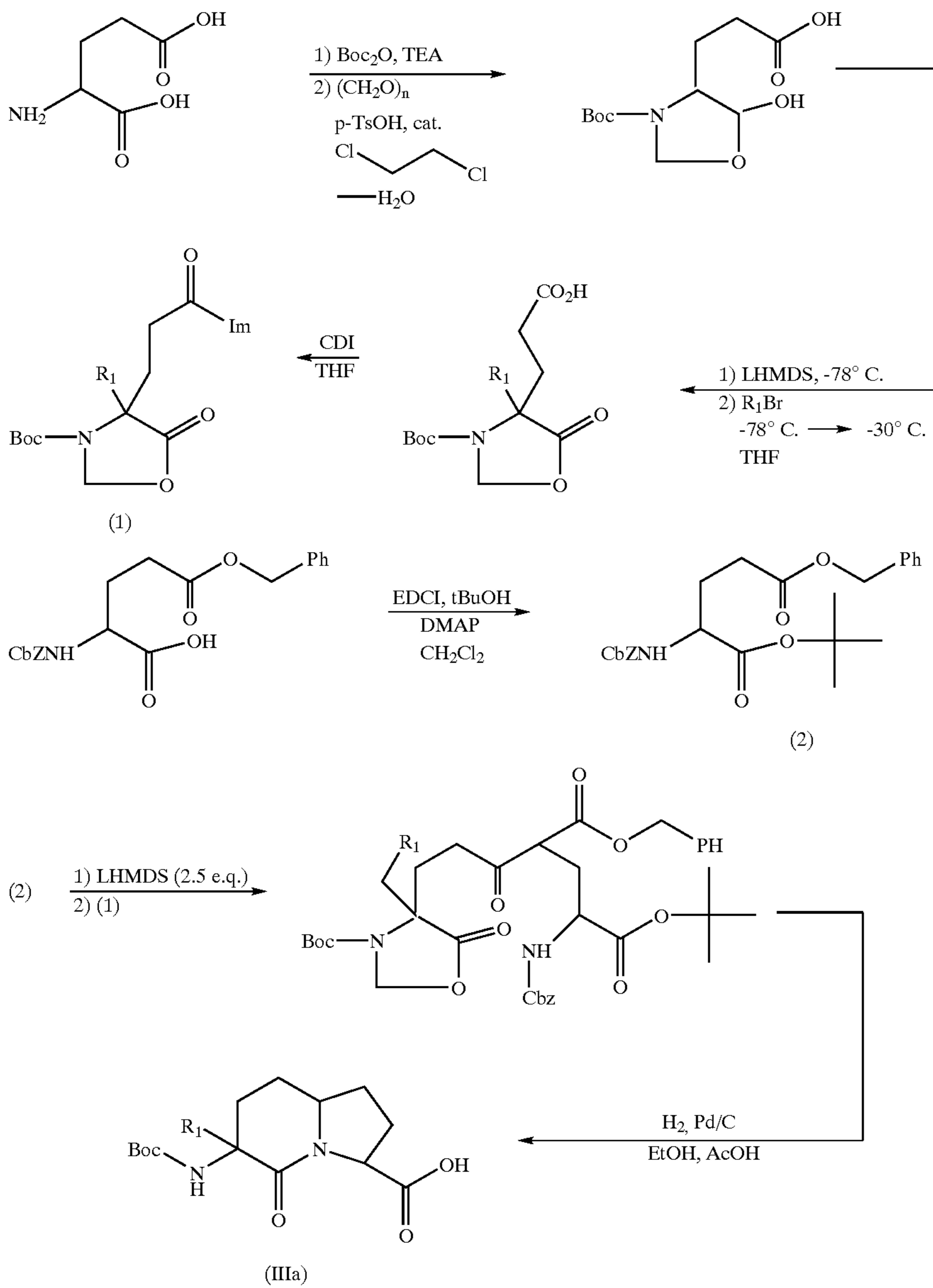
Reaction Scheme (2)
