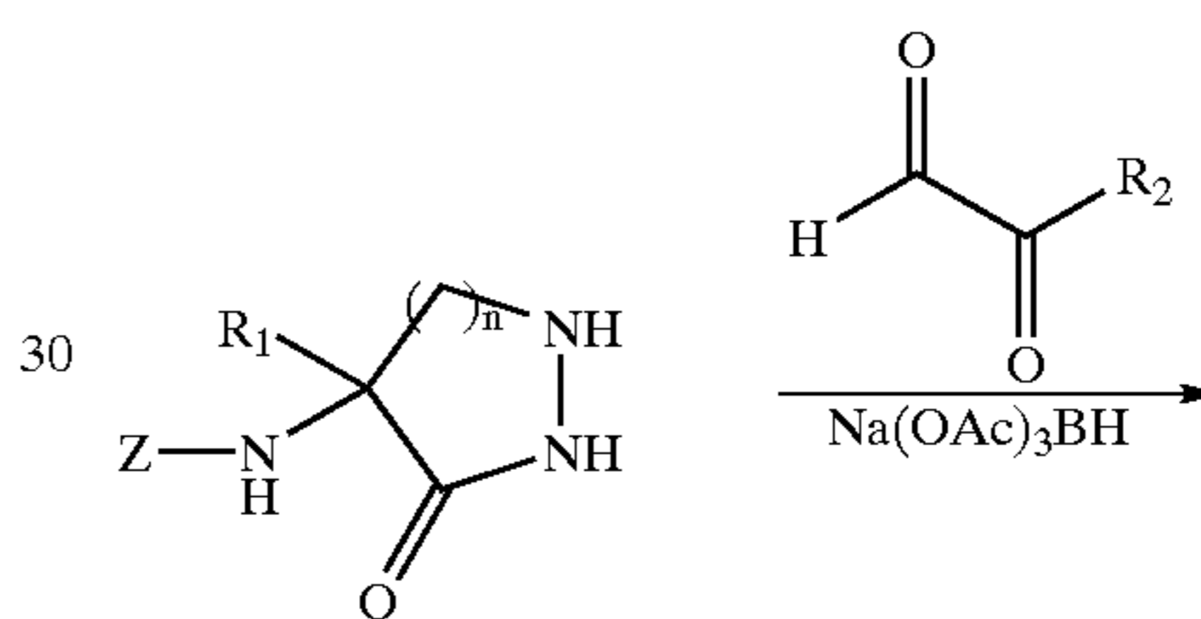
Reaction Scheme (16)
