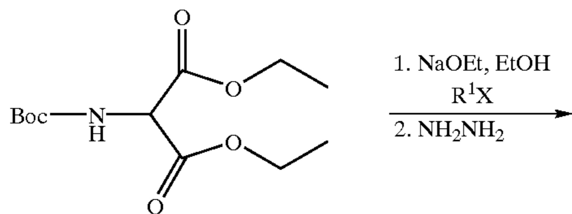
Reaction Scheme (15)
