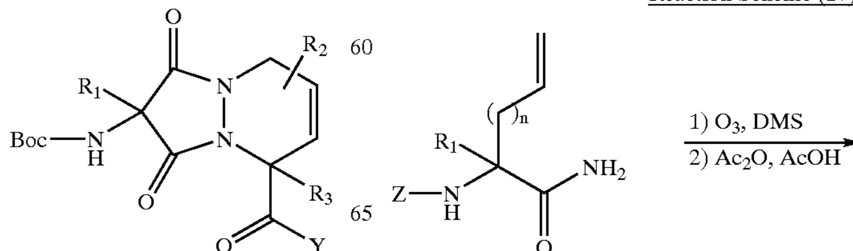
Reaction Scheme (17)
