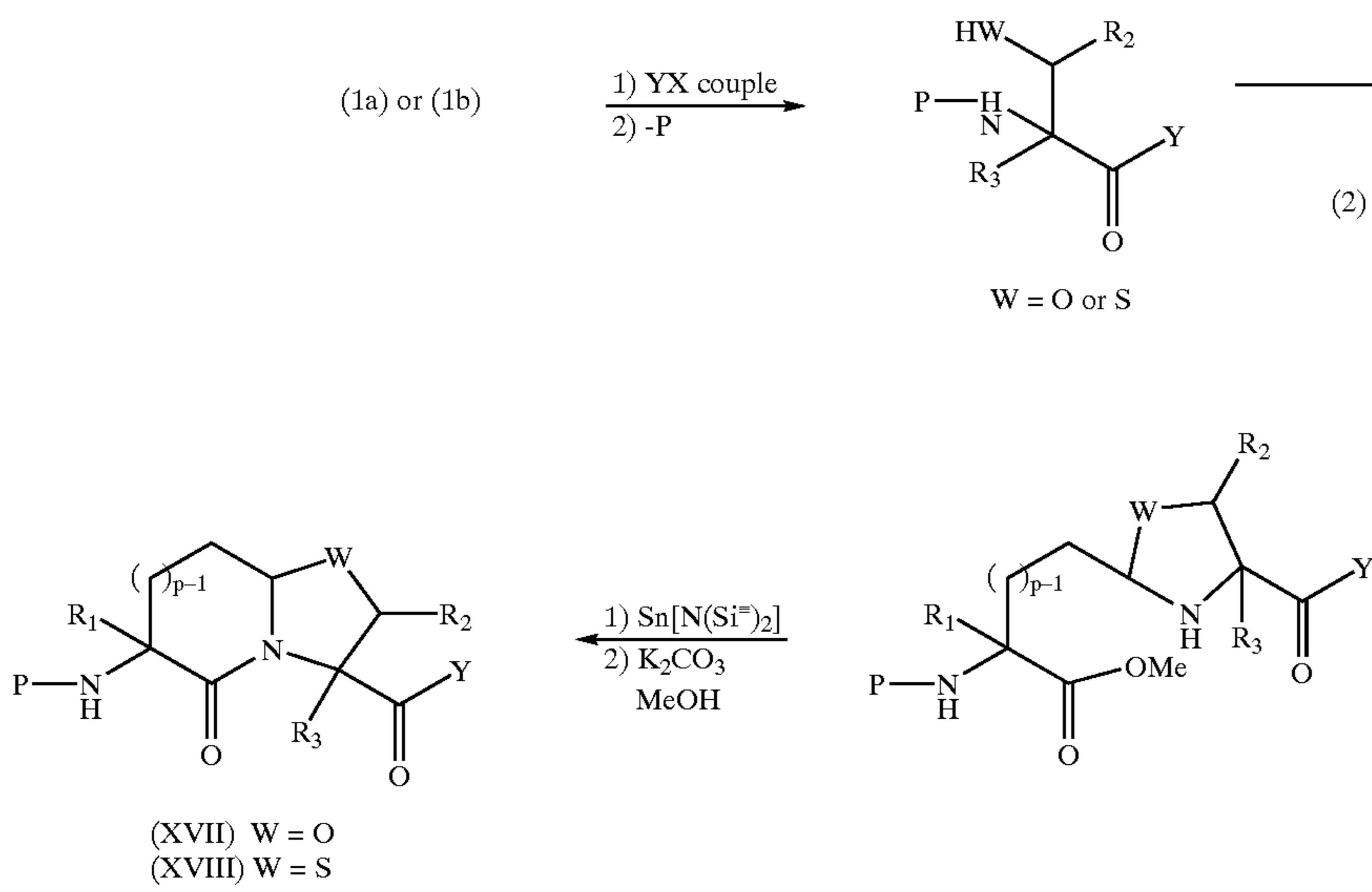
Reaction Scheme (14)
