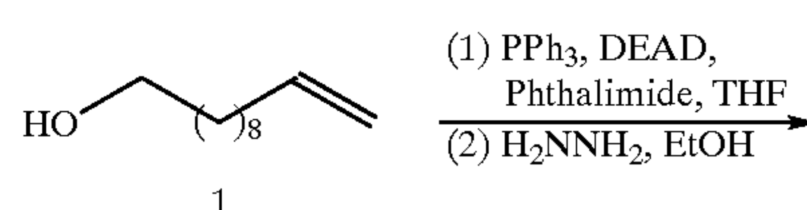
Scheme 1
