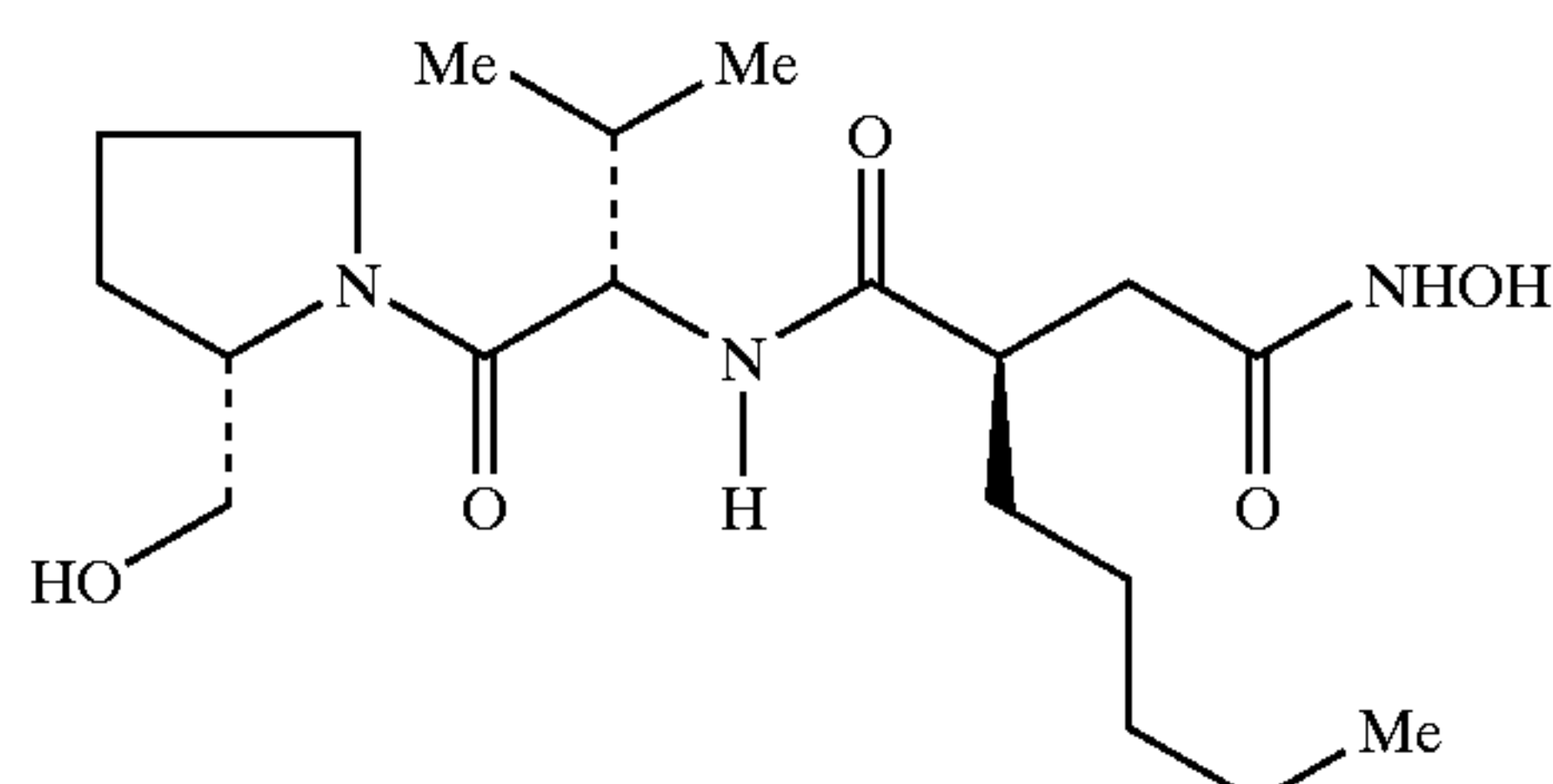
Actinonin
