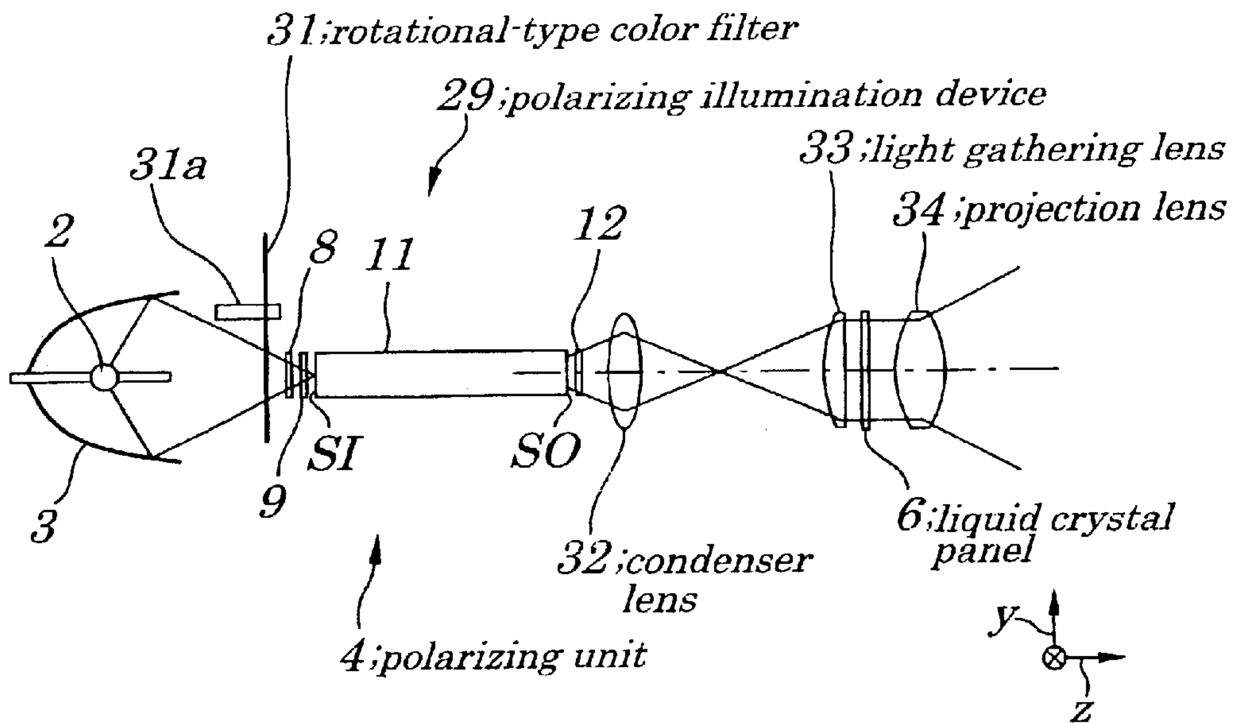
28 ; projection display device
