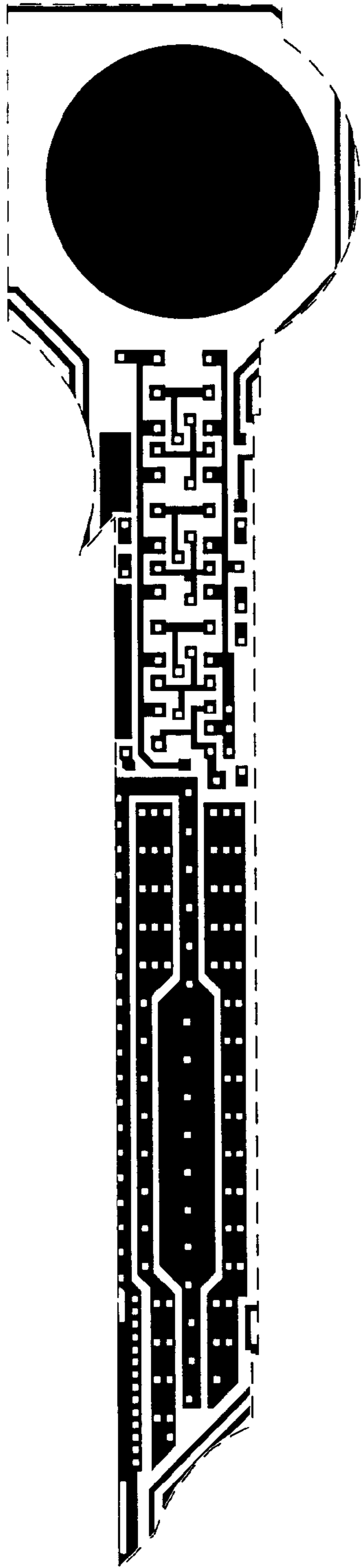
Metal 1 mask
