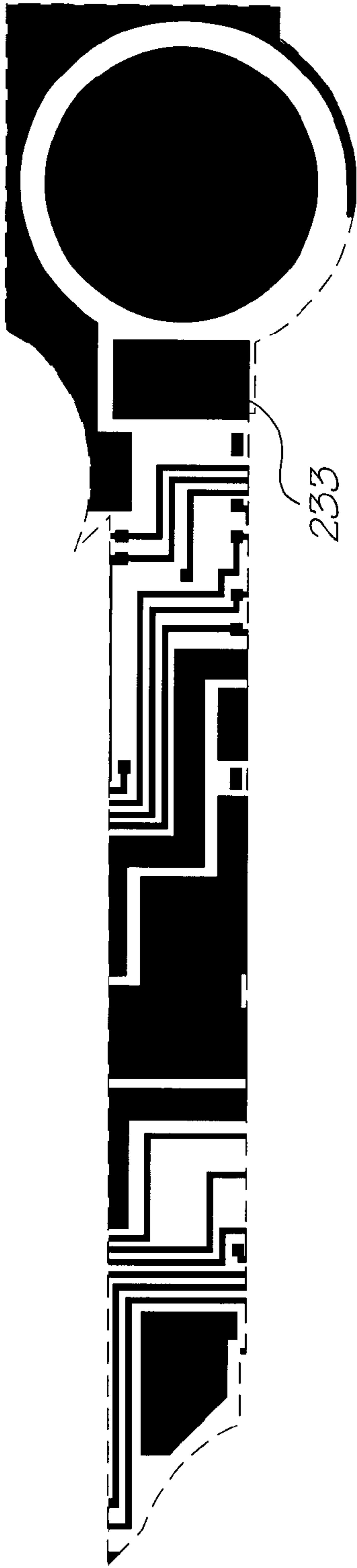
Metal 2 mask
