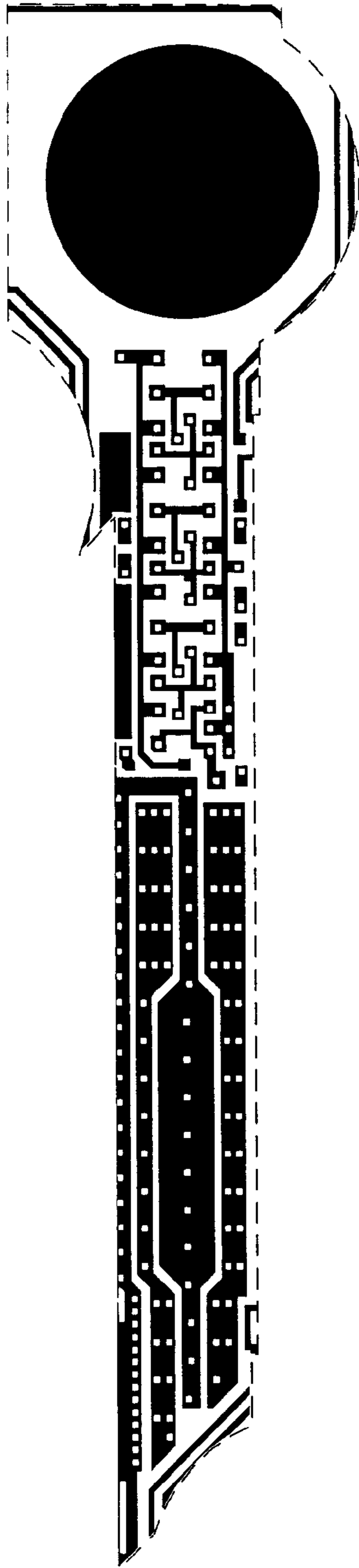
Metal 1 mask
