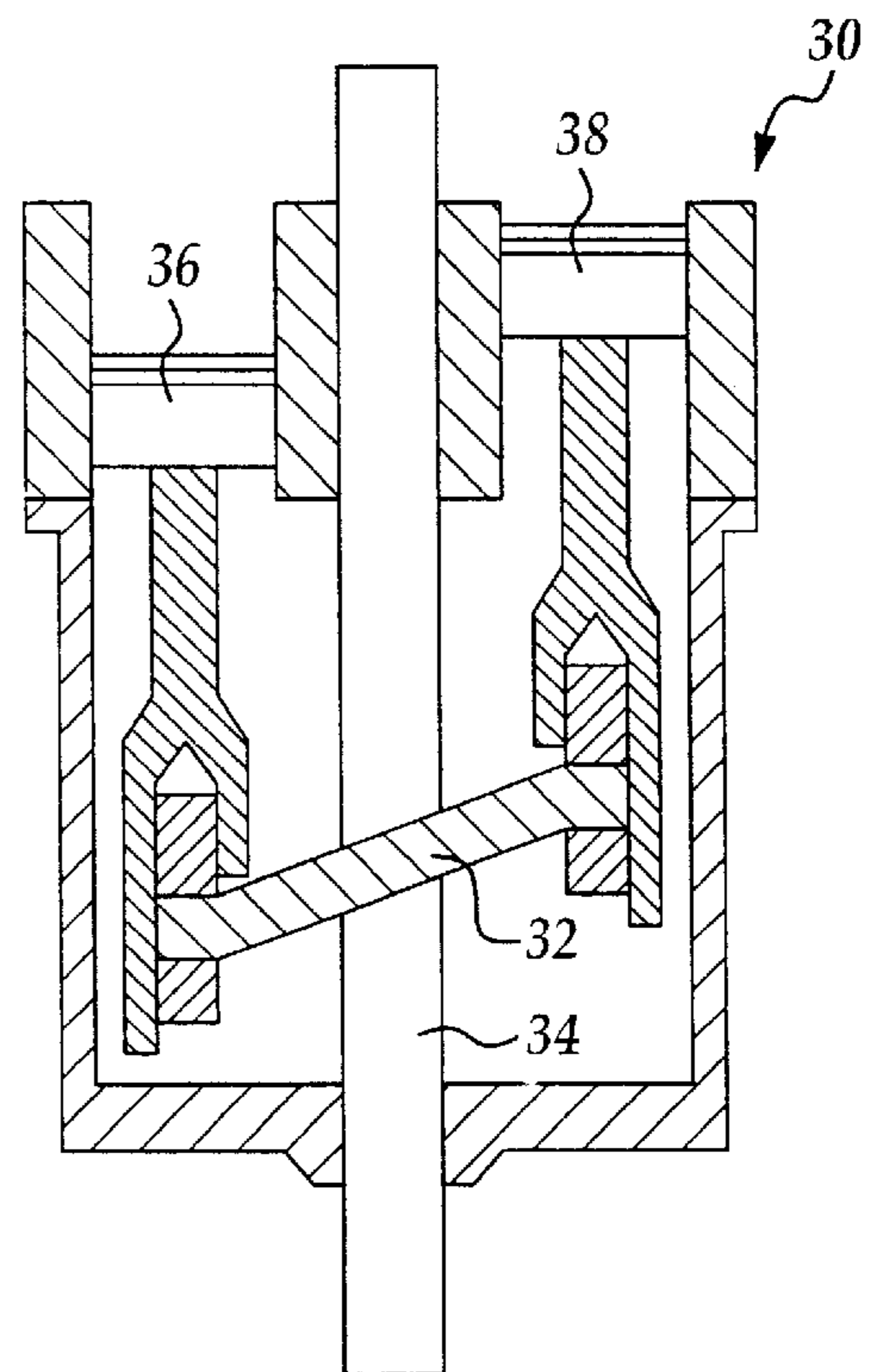
Figure 2A Prior Art
