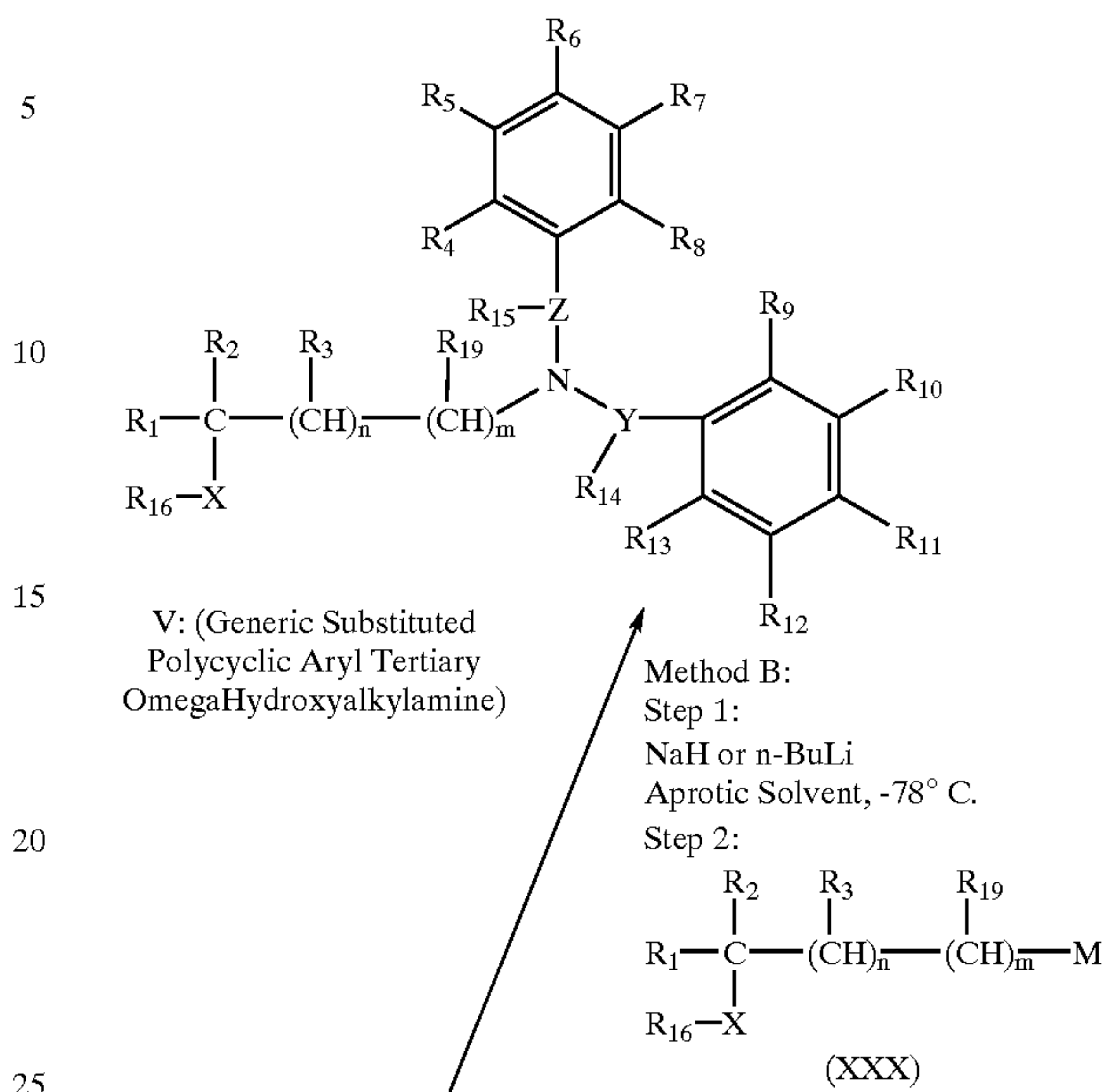
Scheme 5
