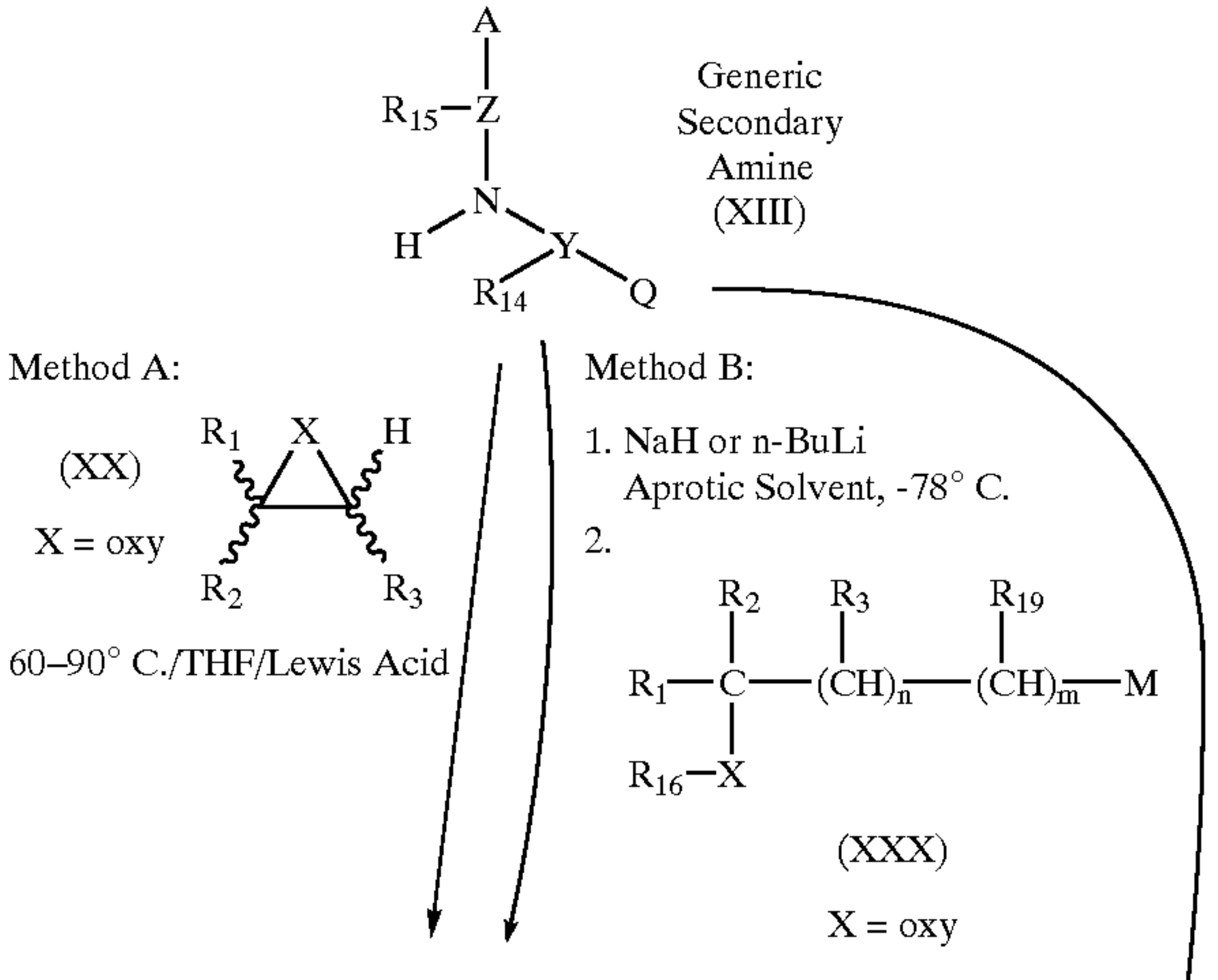
Scheme 2
