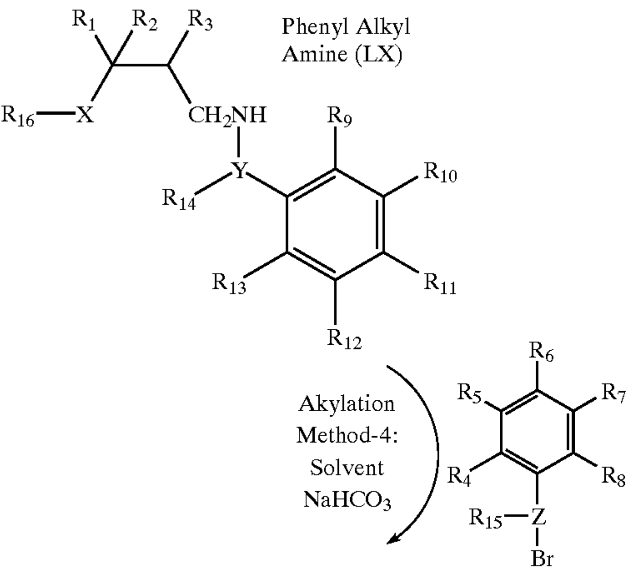
Scheme 34
