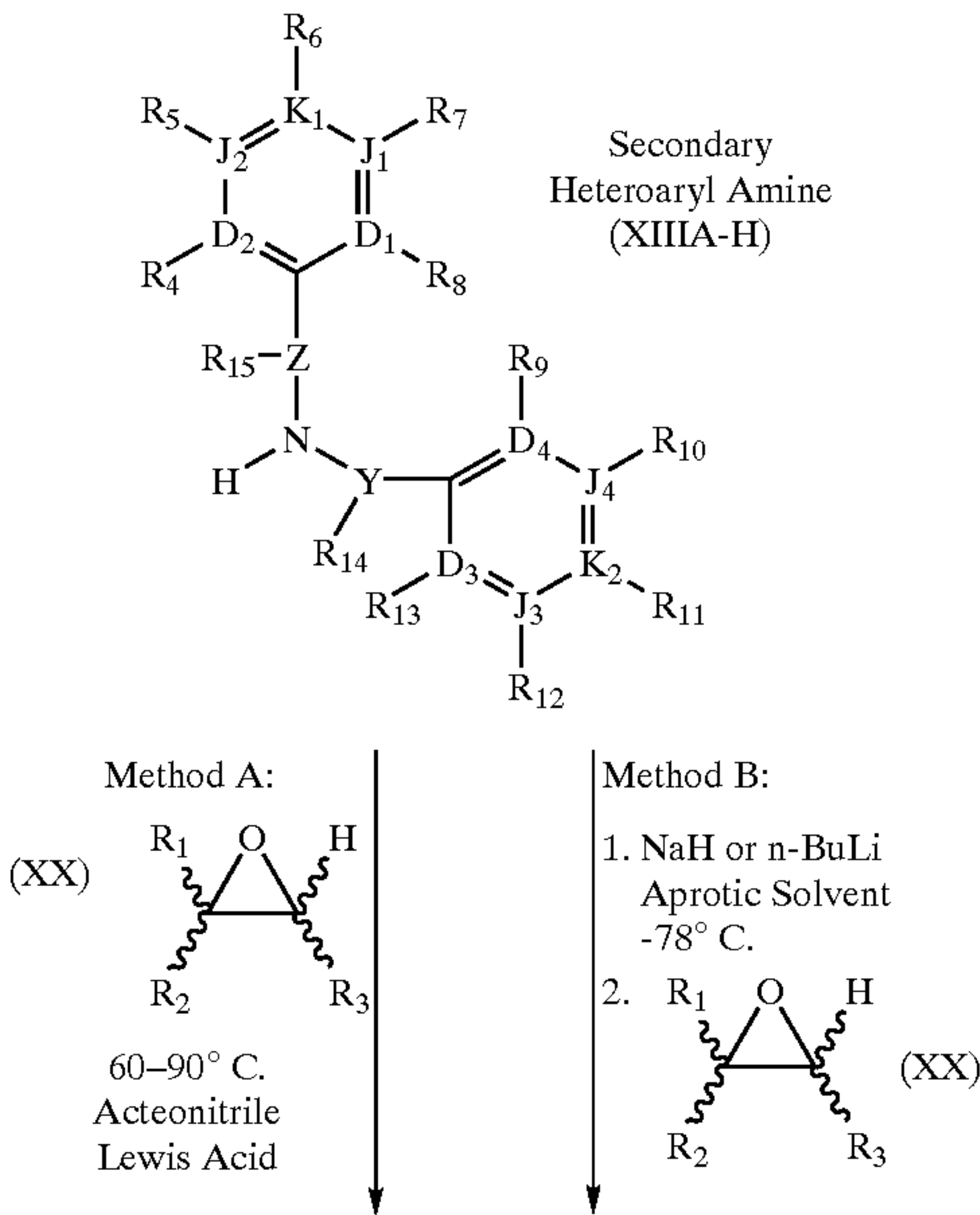
Scheme 7
