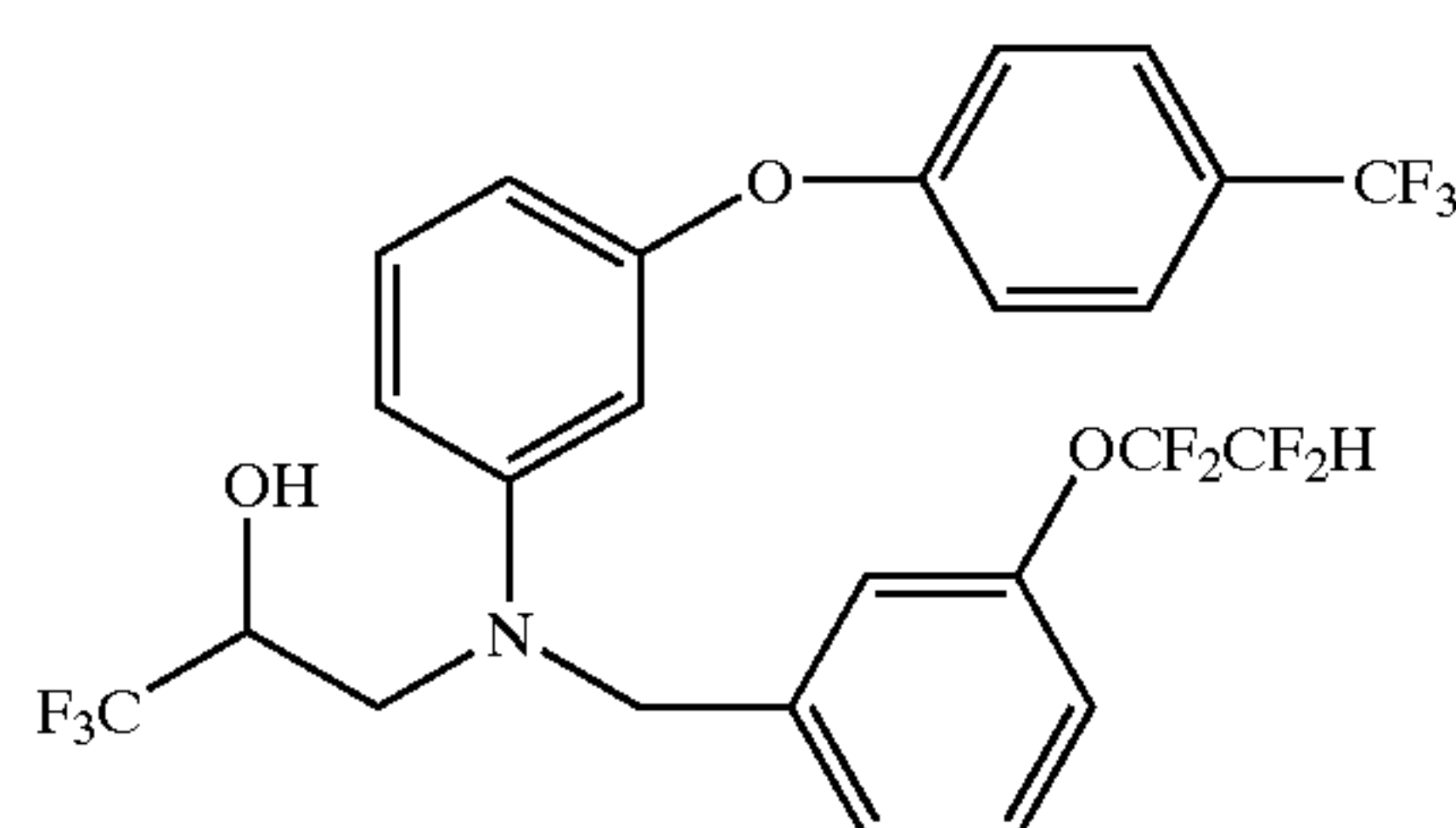
3-[[3-(4-trifluoromethylphenoxy)phenyl][[3-(1,1,2,2-tetrafluoroethoxy)-phenyl]methyl]amino]-1,1,1-trifluoro-2-propanol
