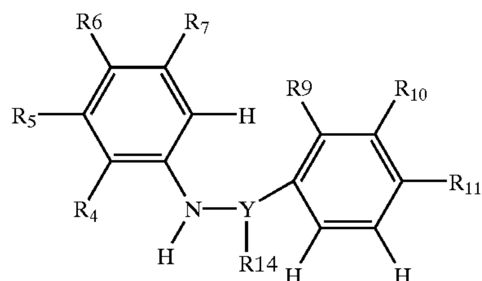
Structure of “Secondary Phenyl Amine” Reagents.
