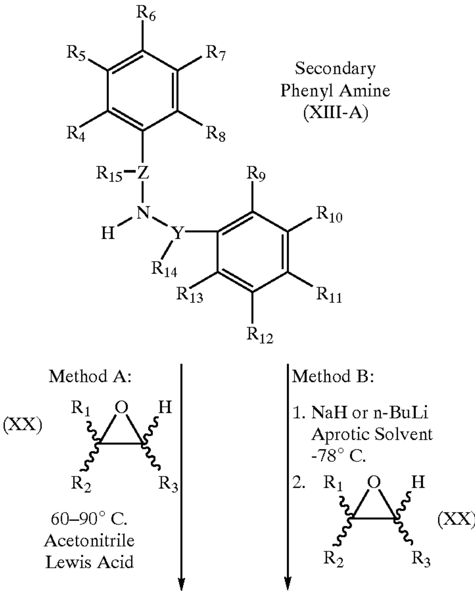
Scheme 11
