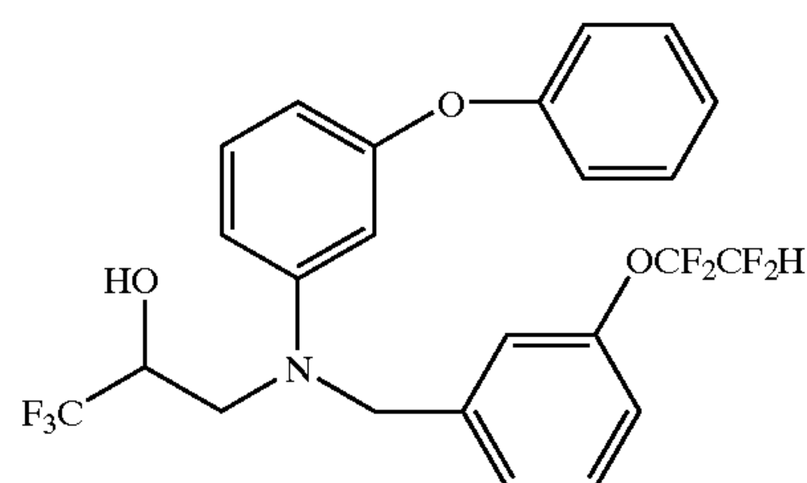
3-[(3-phenoxyphenyl)[3-(1,1,2,2-tetrafluoroethoxy)phenyl]methyl]amino]-1,1,1-trifluoro-2-propanol
