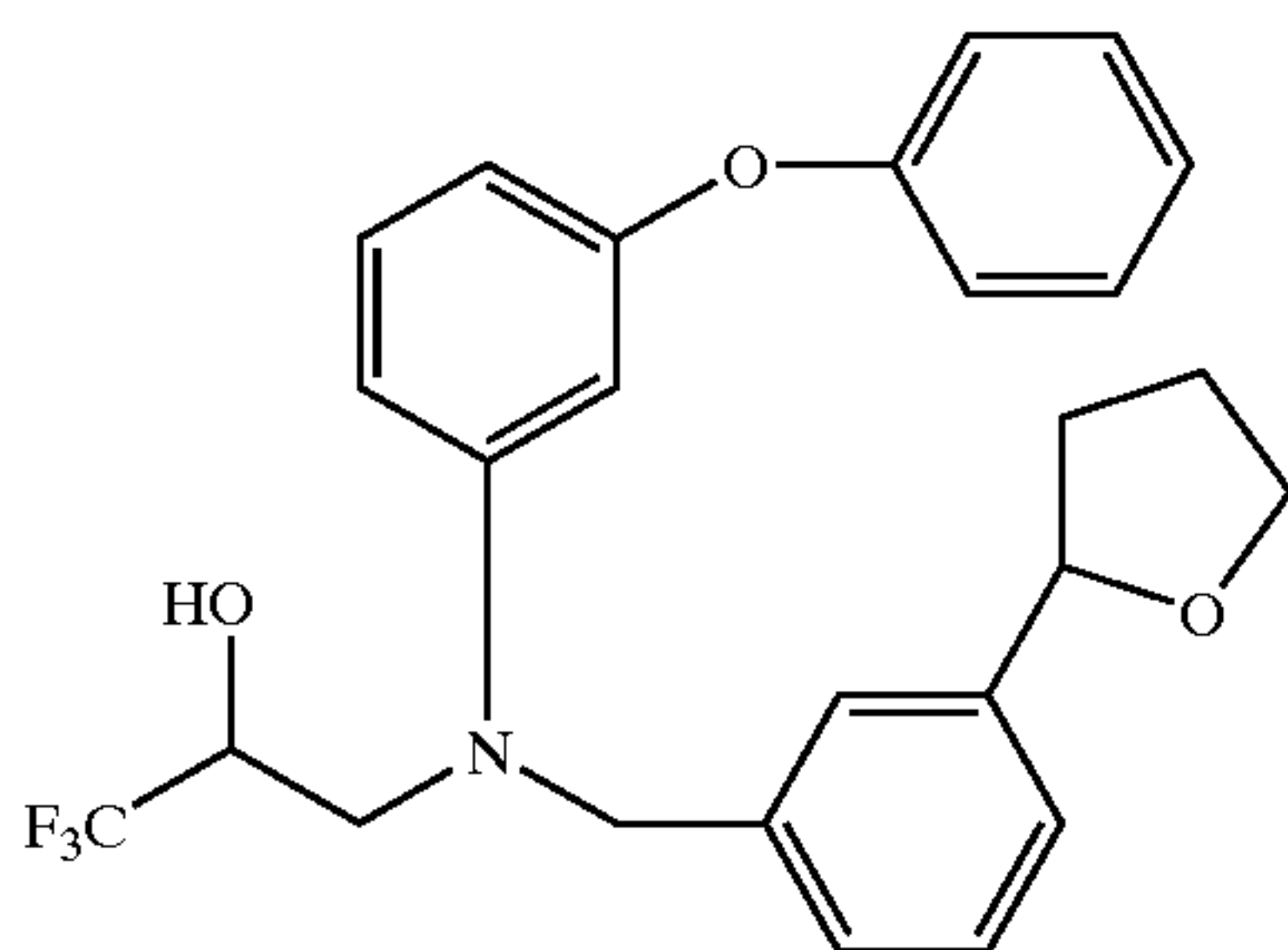
3-[(3-phenoxyphenyl)[[3-(tetrahydro-2-furanyl)phenyl]methyl]amino]-1,1,1-trifluoro-2-propanol
