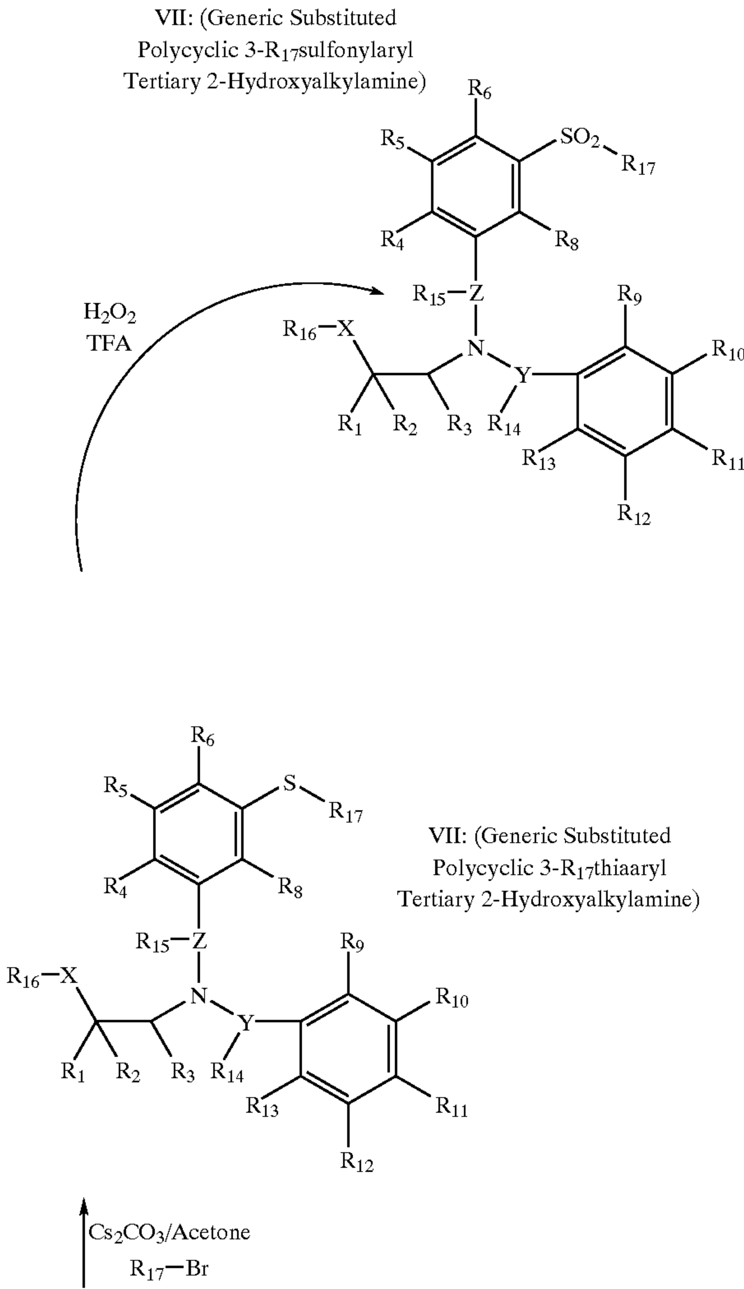
Scheme 19
