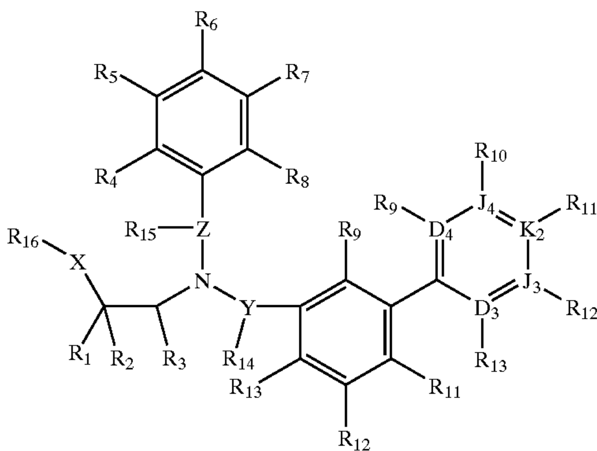
Scheme 41
