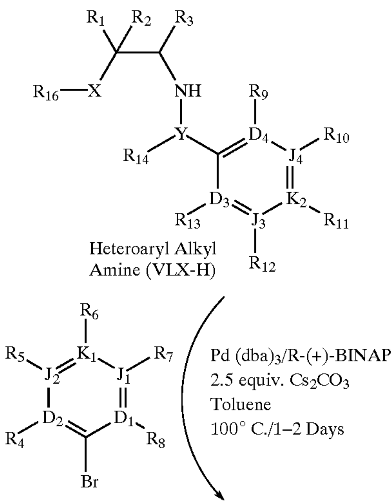
Scheme 47
