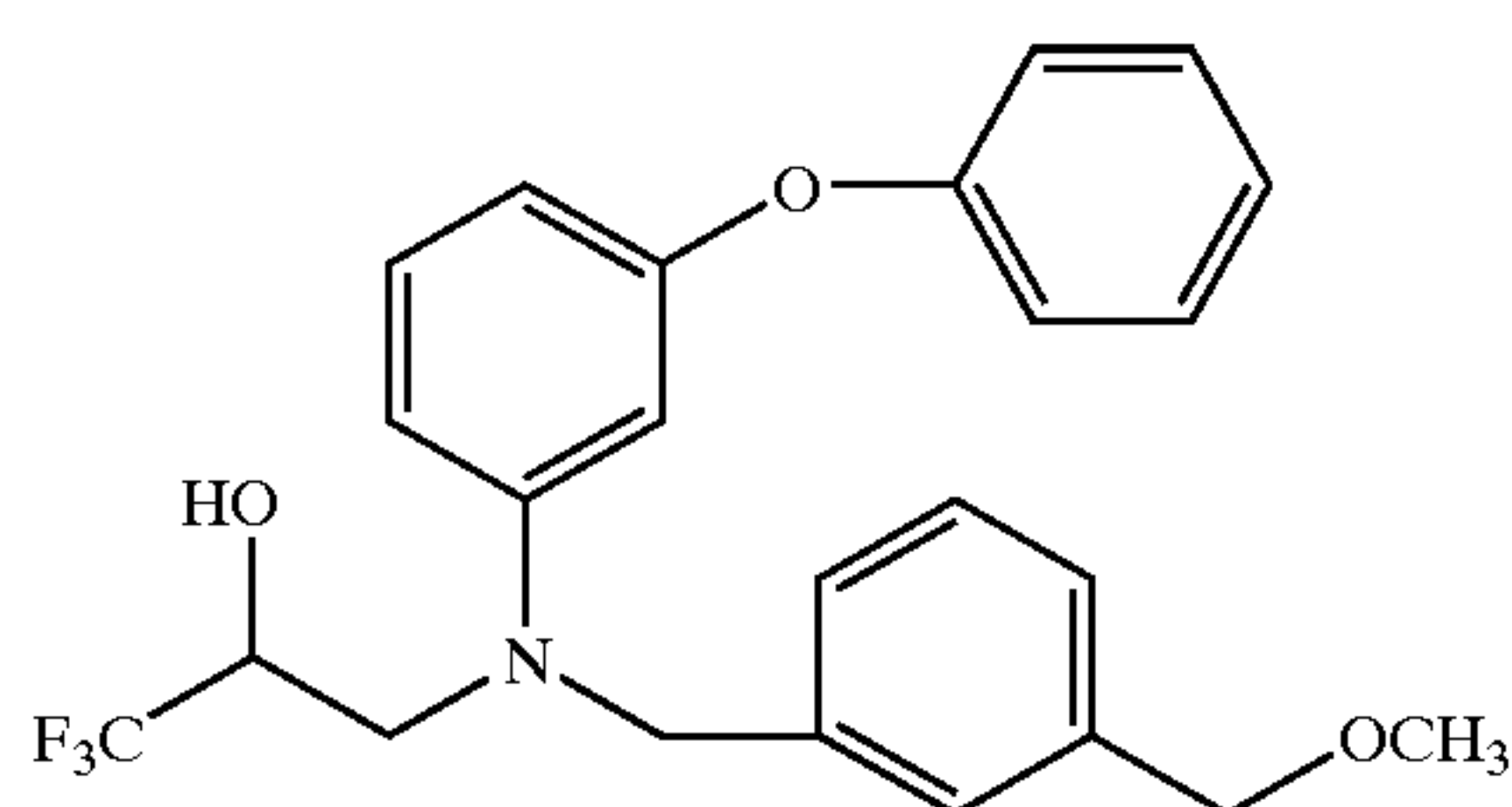
3-[[3-(3-phenoxyphenyl)(3,3,3-trifluoro-2-hydroxypropyl) amino]methyl]methoxymethylbenzene
