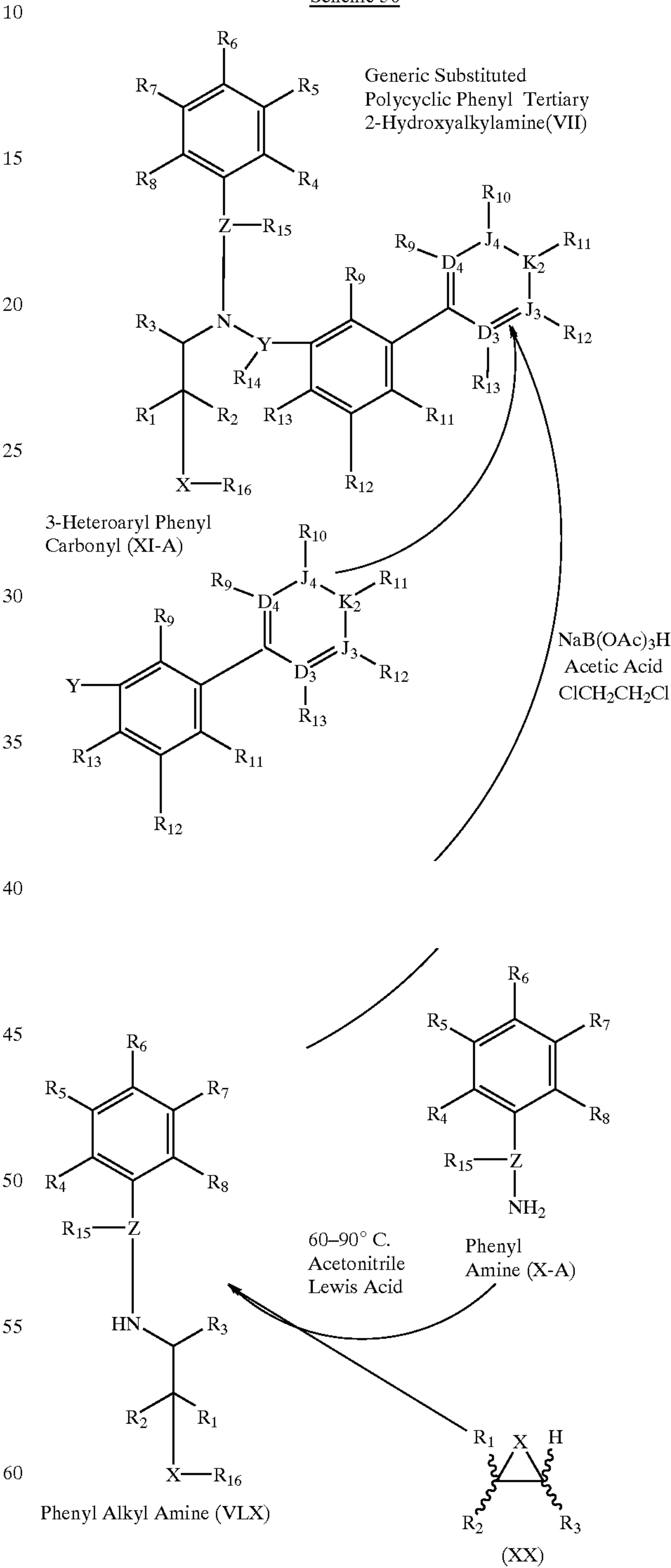
Scheme 56
