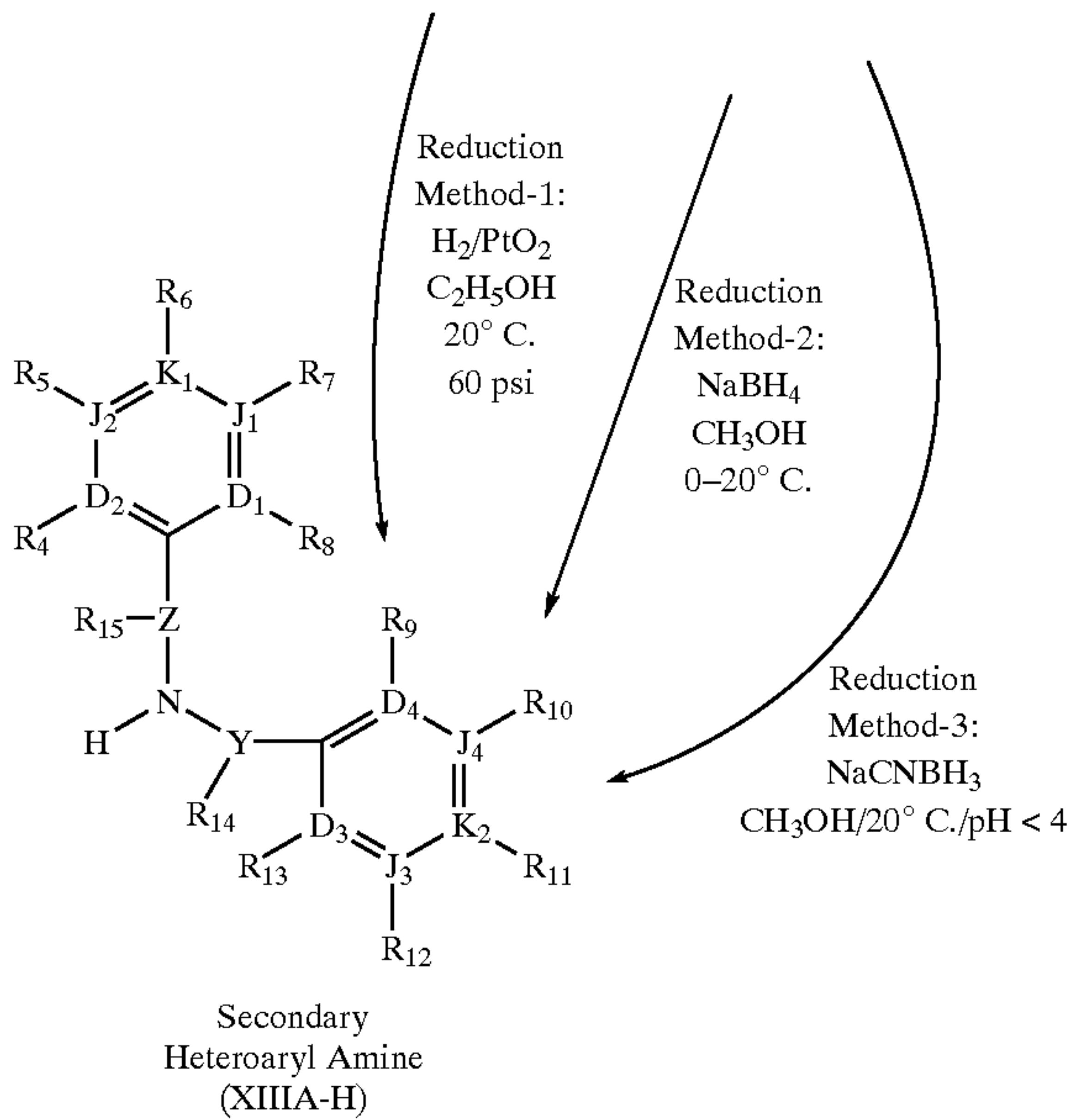
Scheme 4
