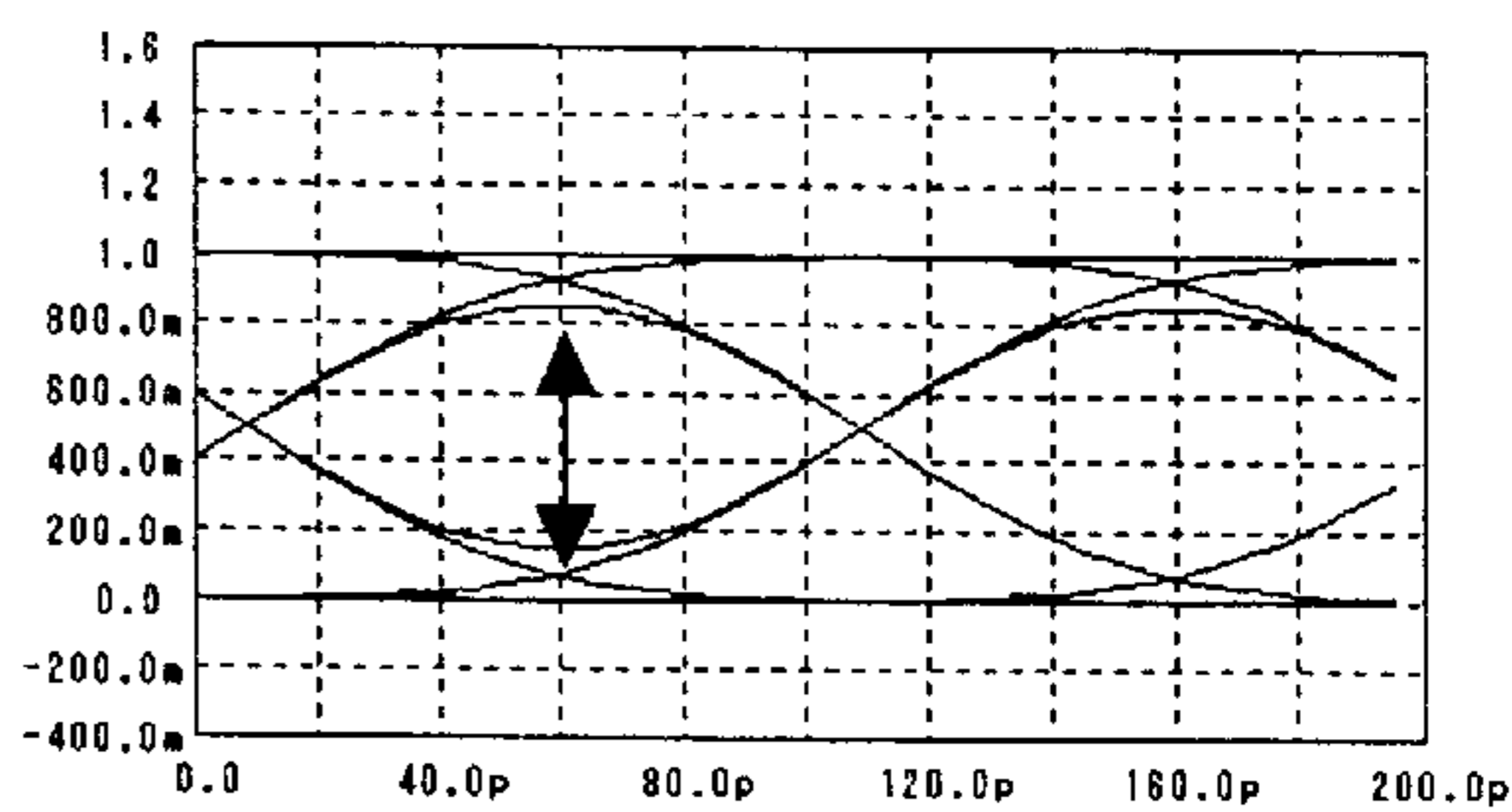
CASE IN WHICH APERTURE IN AMPLITUDE DIRECTION DECREASES
