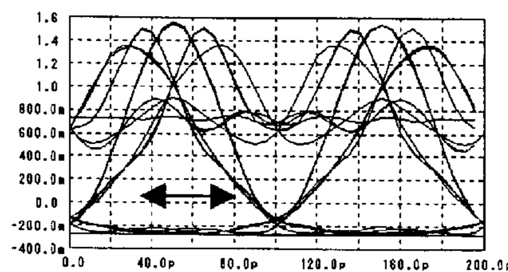
CASE IN WHICH APERTURE IN PHASE DIRECTION DECREASES
