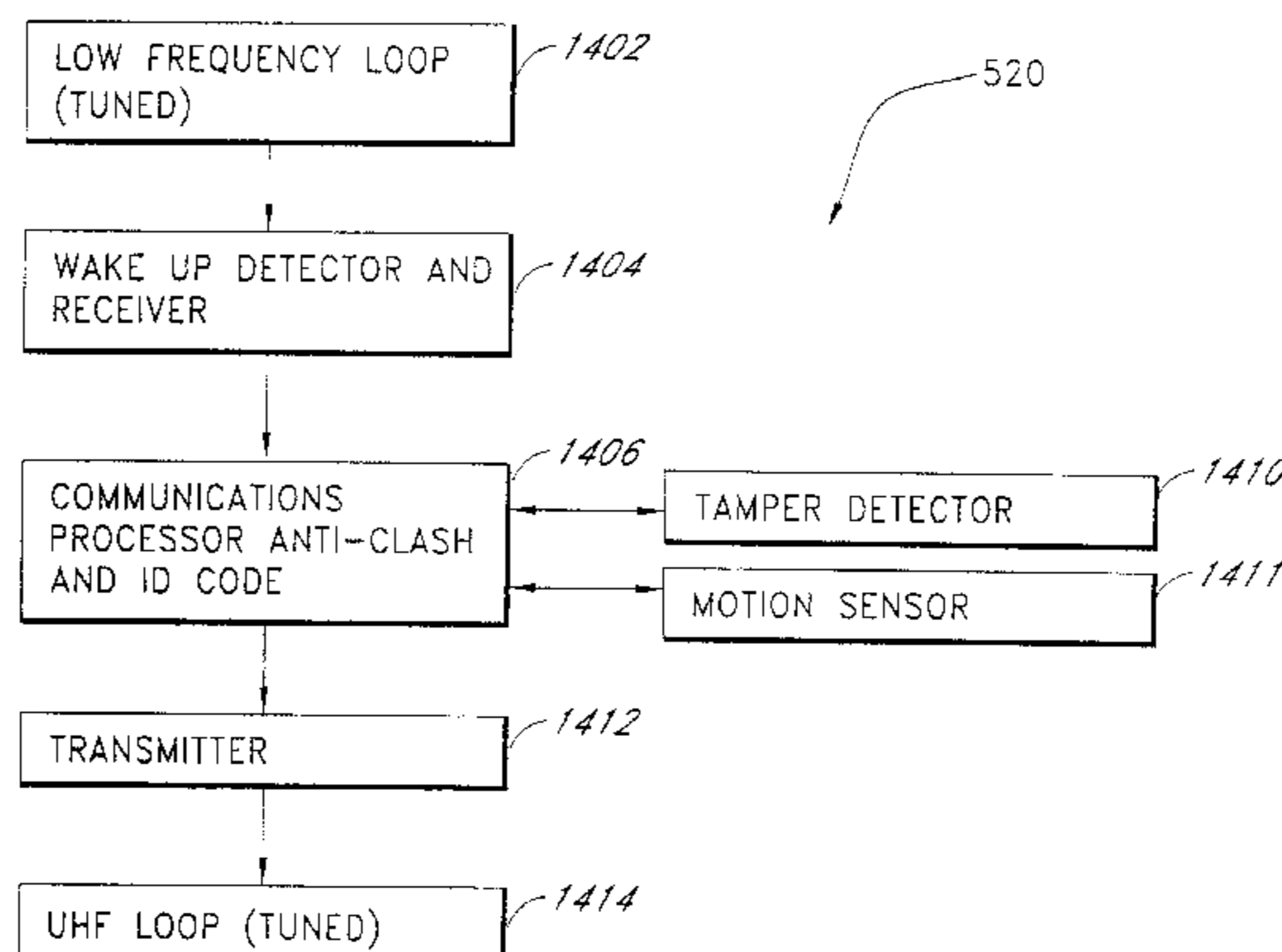
ASSET TAG/TRANSPONDER CONFIGURATION
