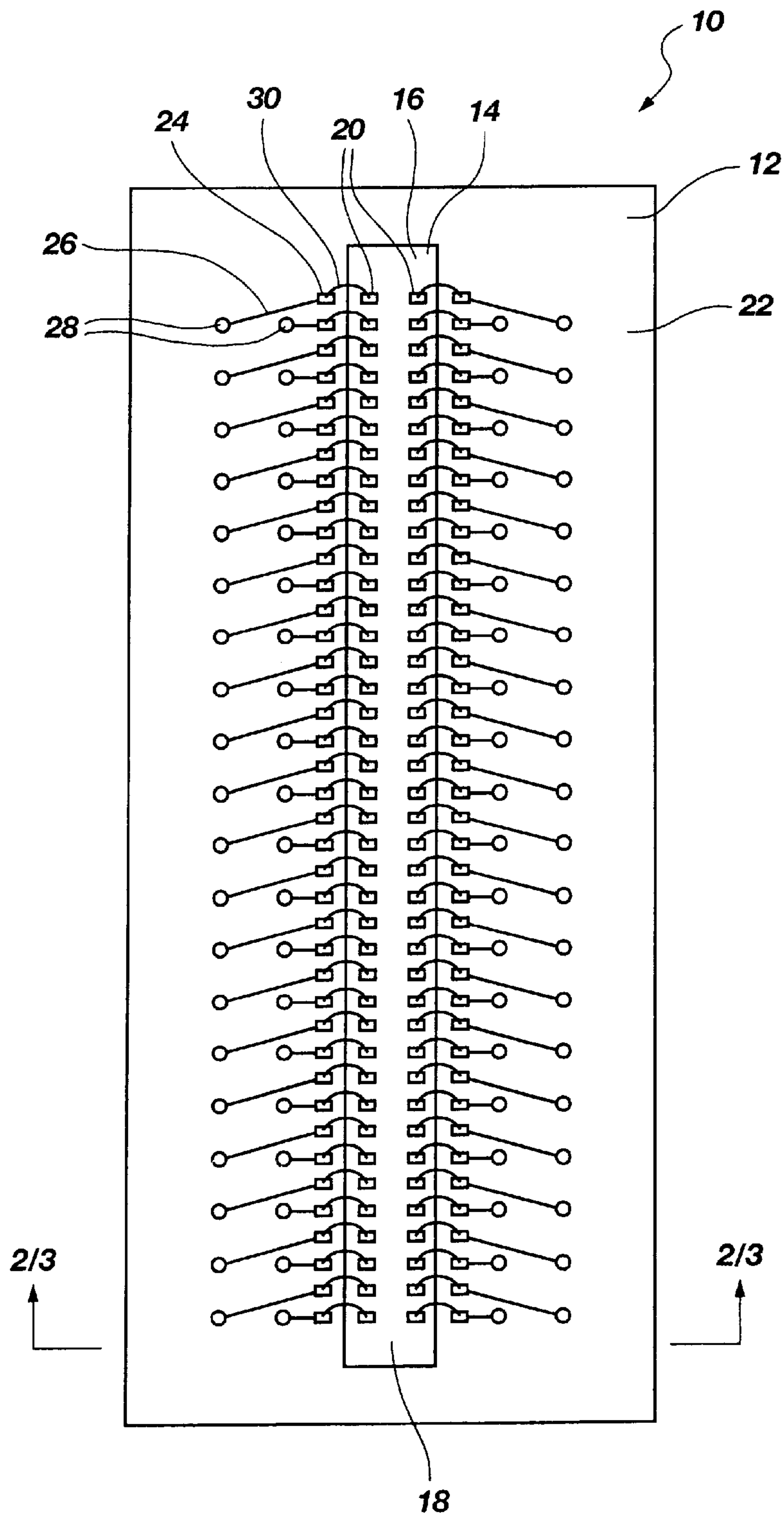
Fig. 1 (PRIOR ART)
