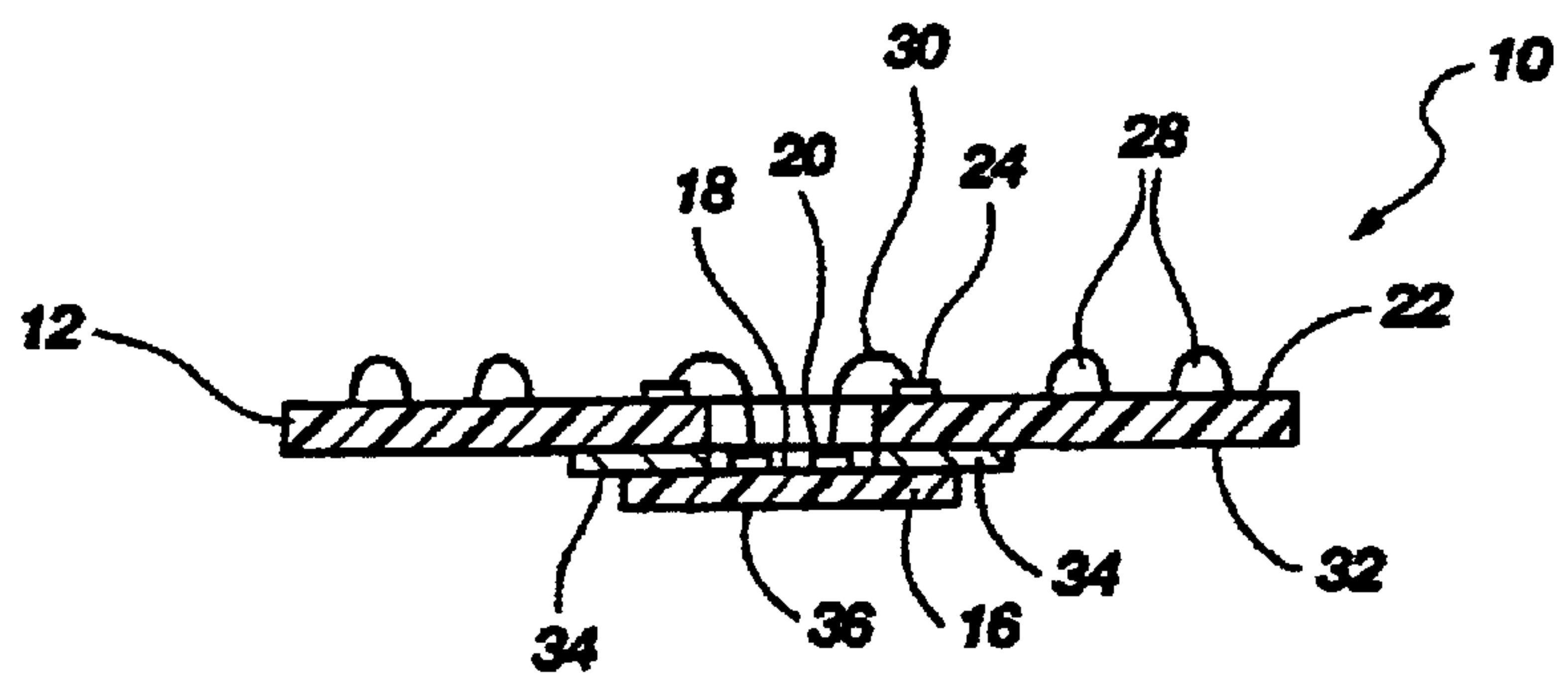
Fig. 2 (PRIOR ART)
