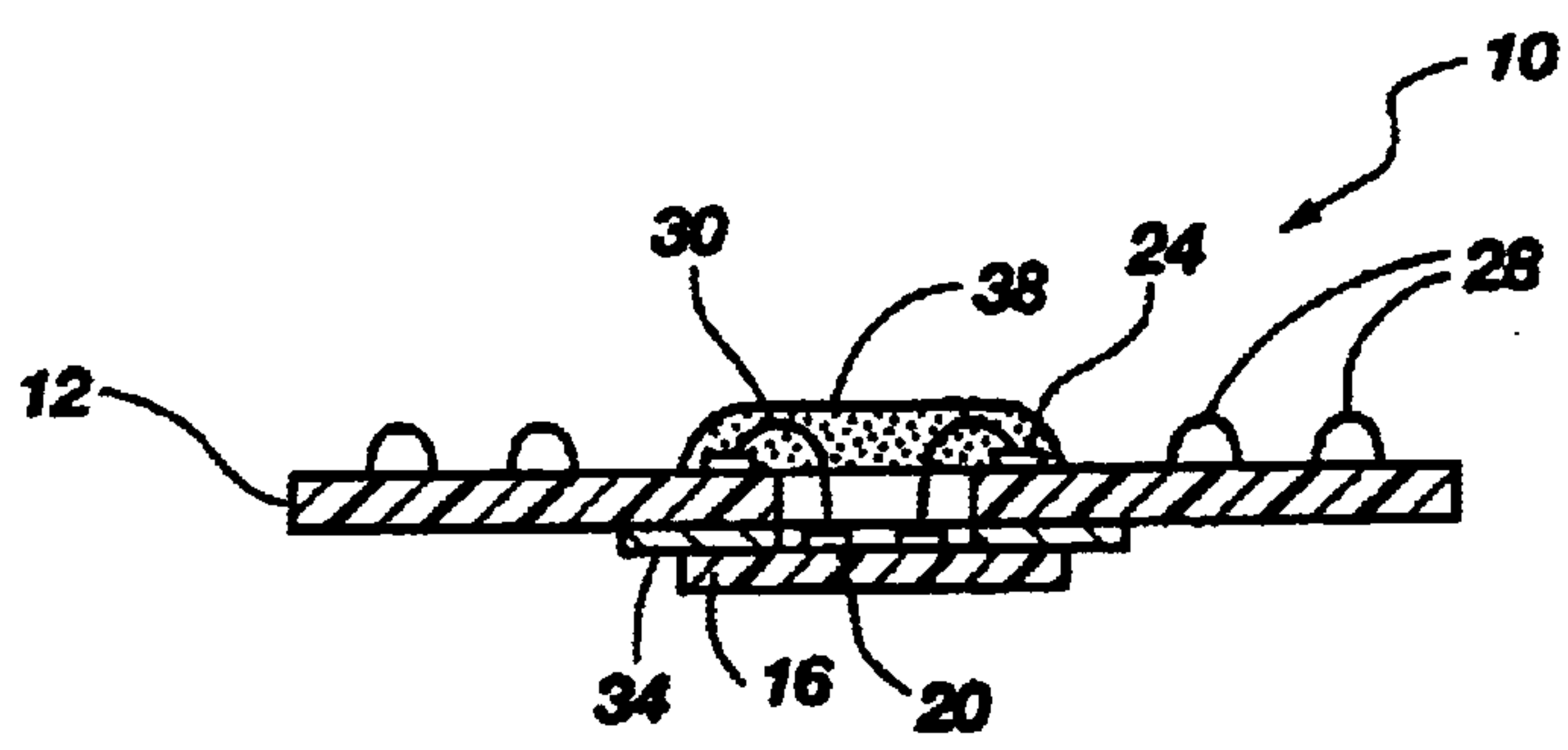
Fig. 3 (PRIOR ART)
