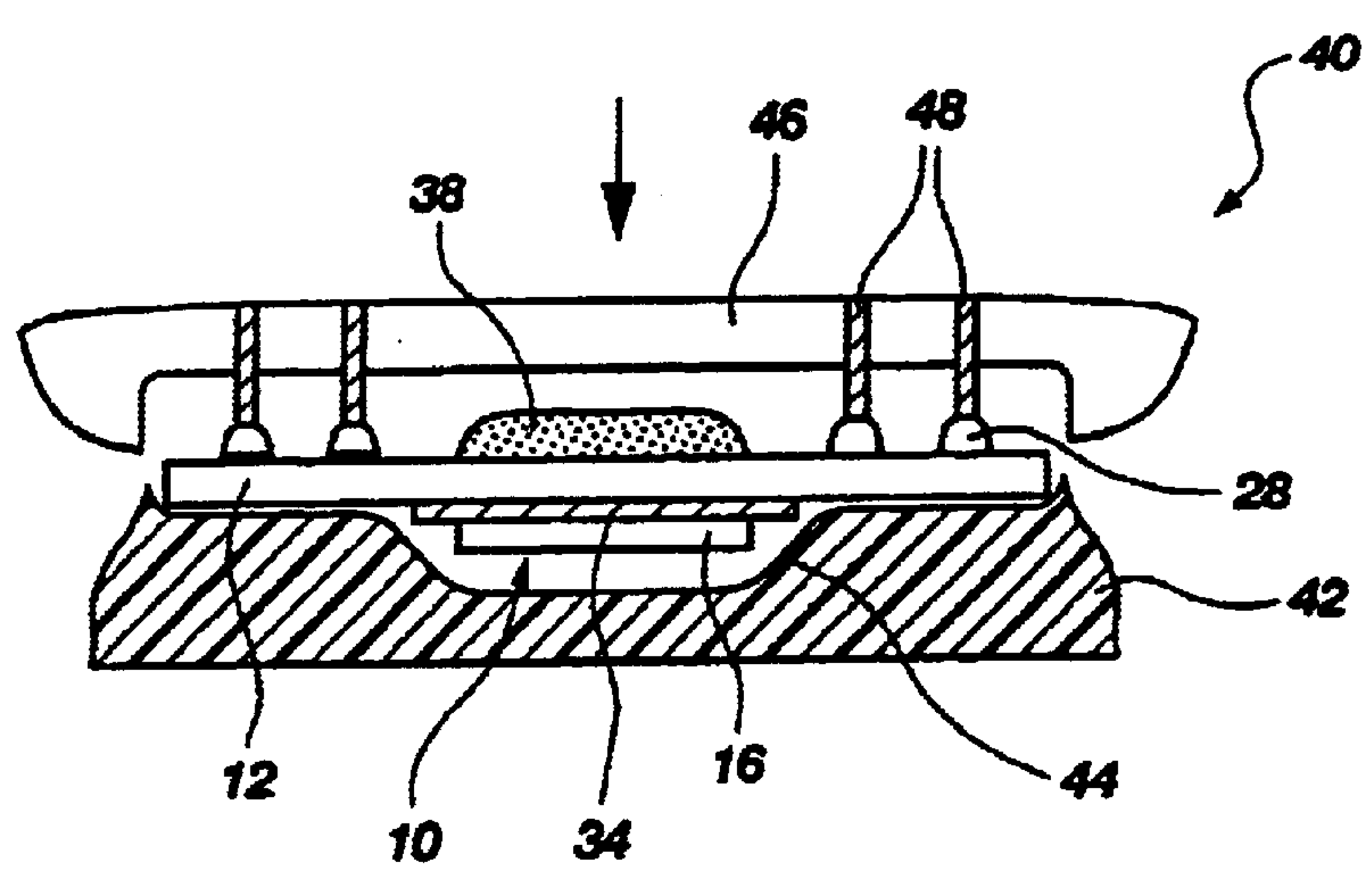
Fig. 4 (PRIOR ART)
