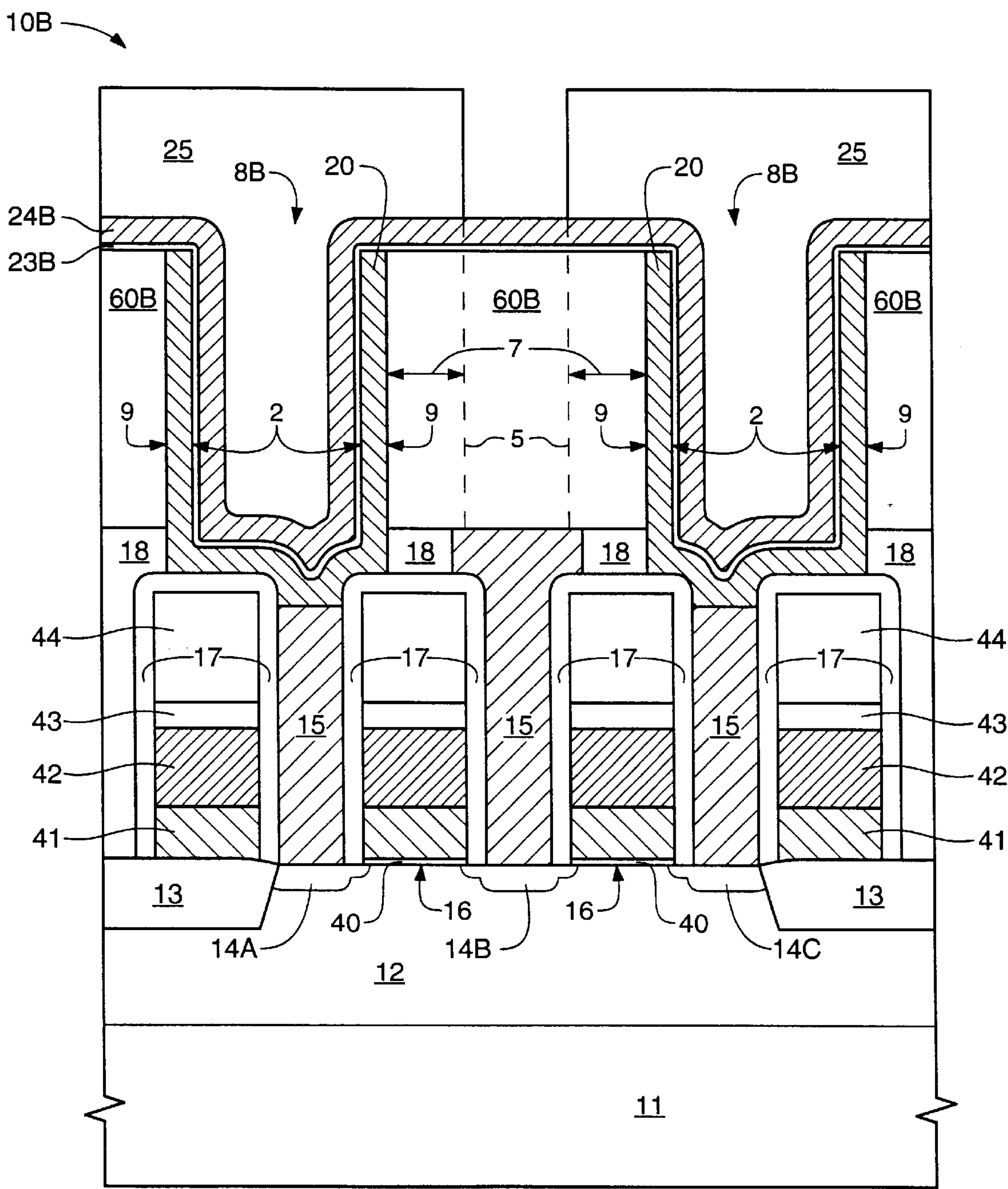
FIG. 3 (PRIOR ART)
