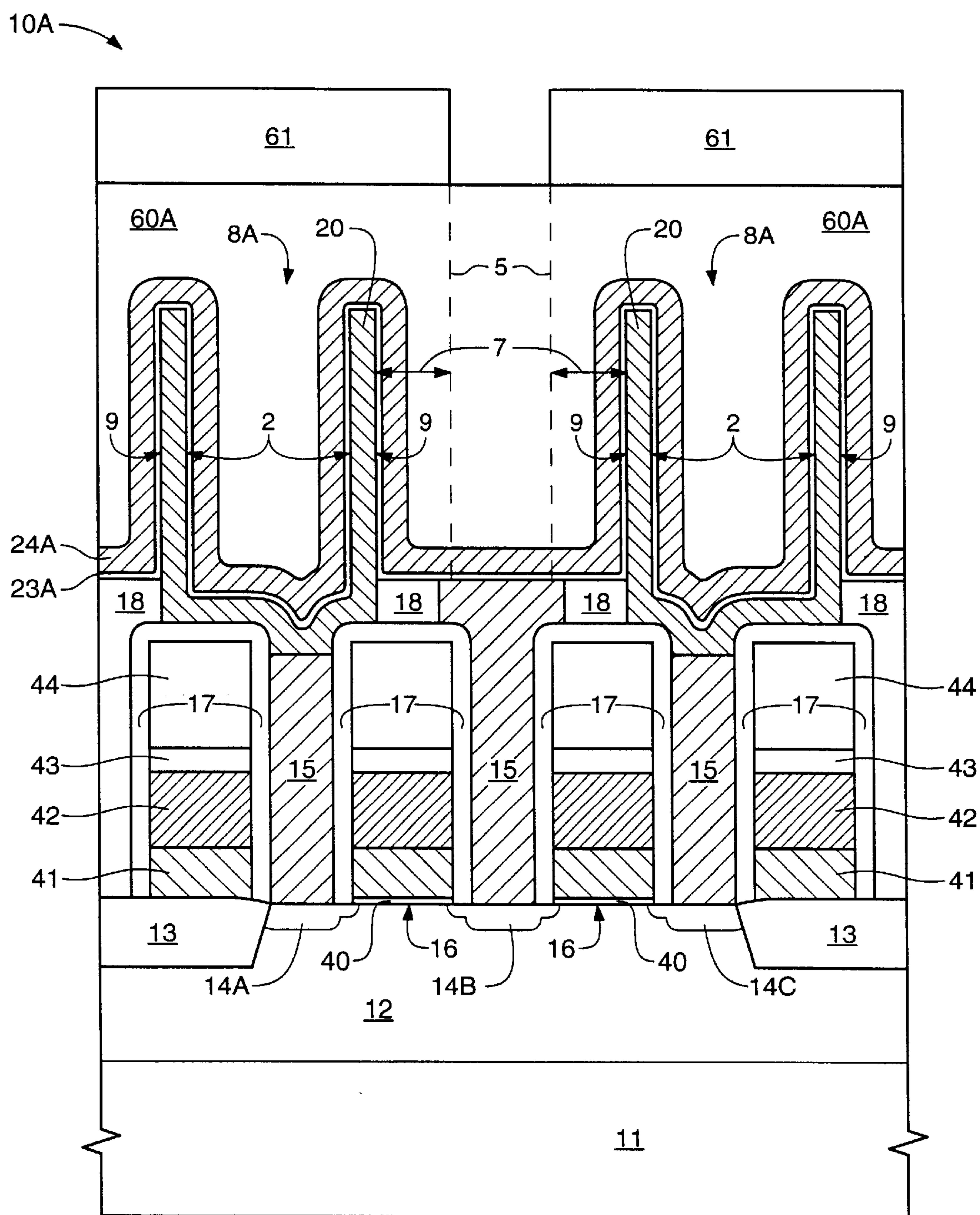
FIG. 2 (PRIOR ART)
