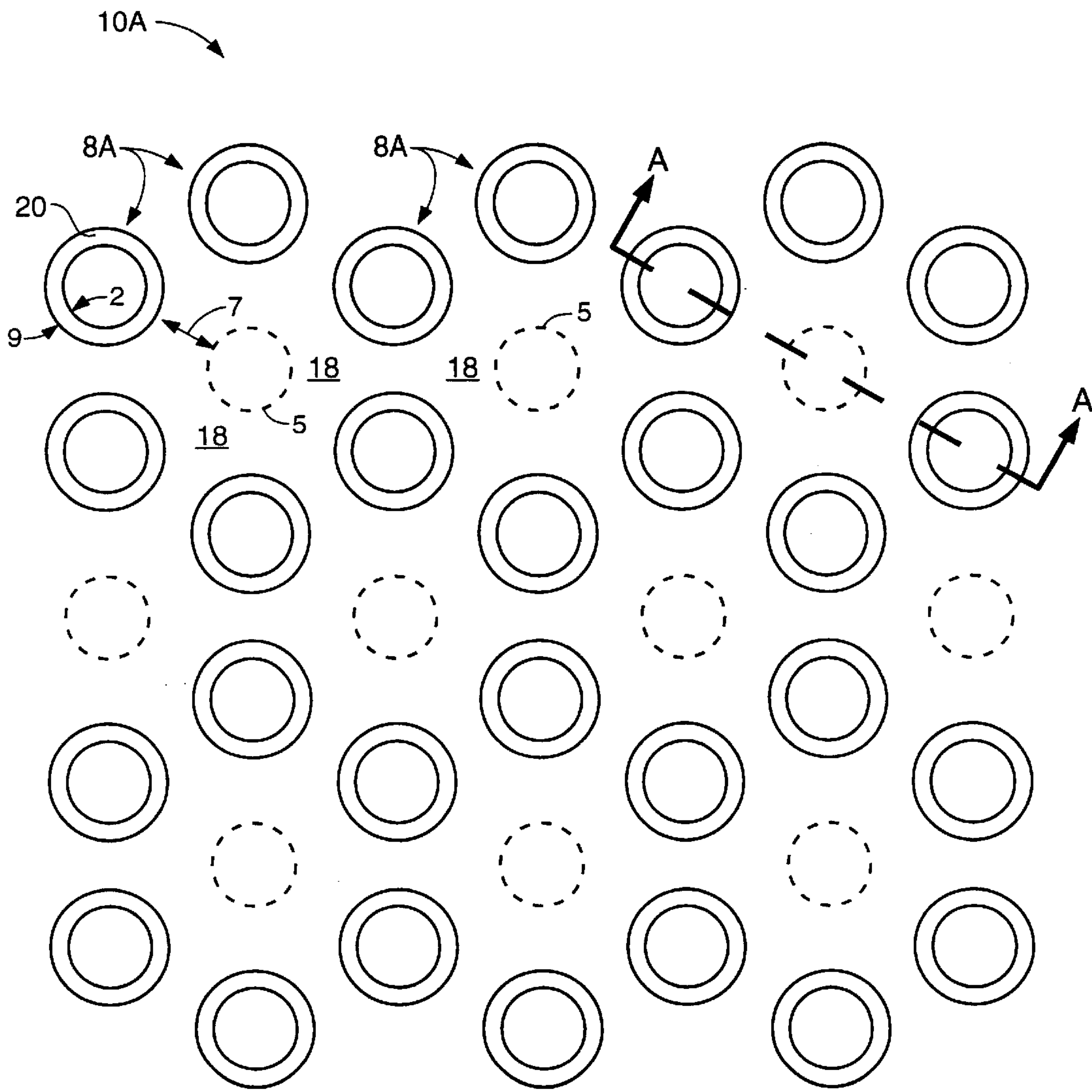
FIG. 1 (PRIOR ART)
