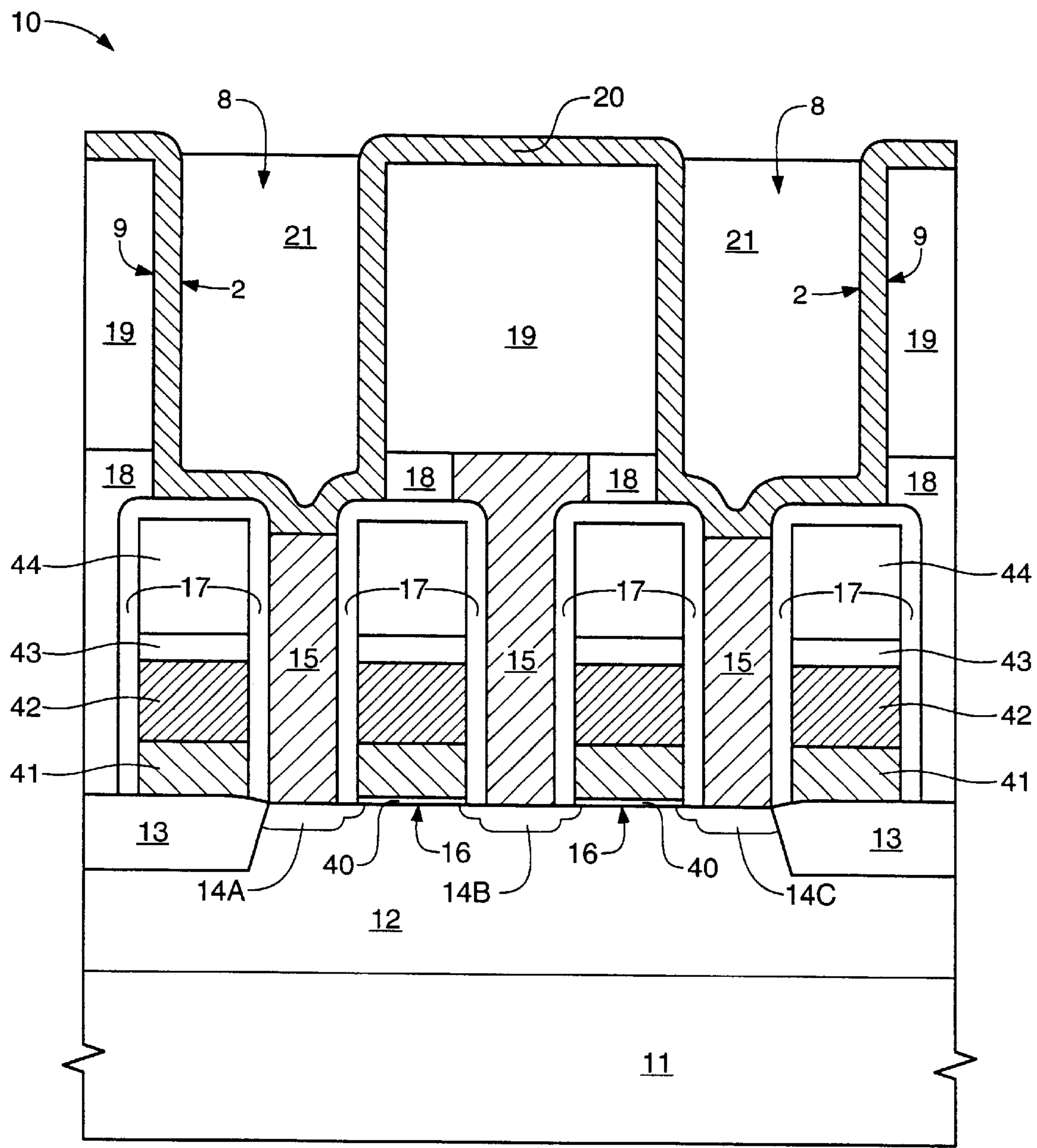
FIG. 5 (PRIOR ART)
