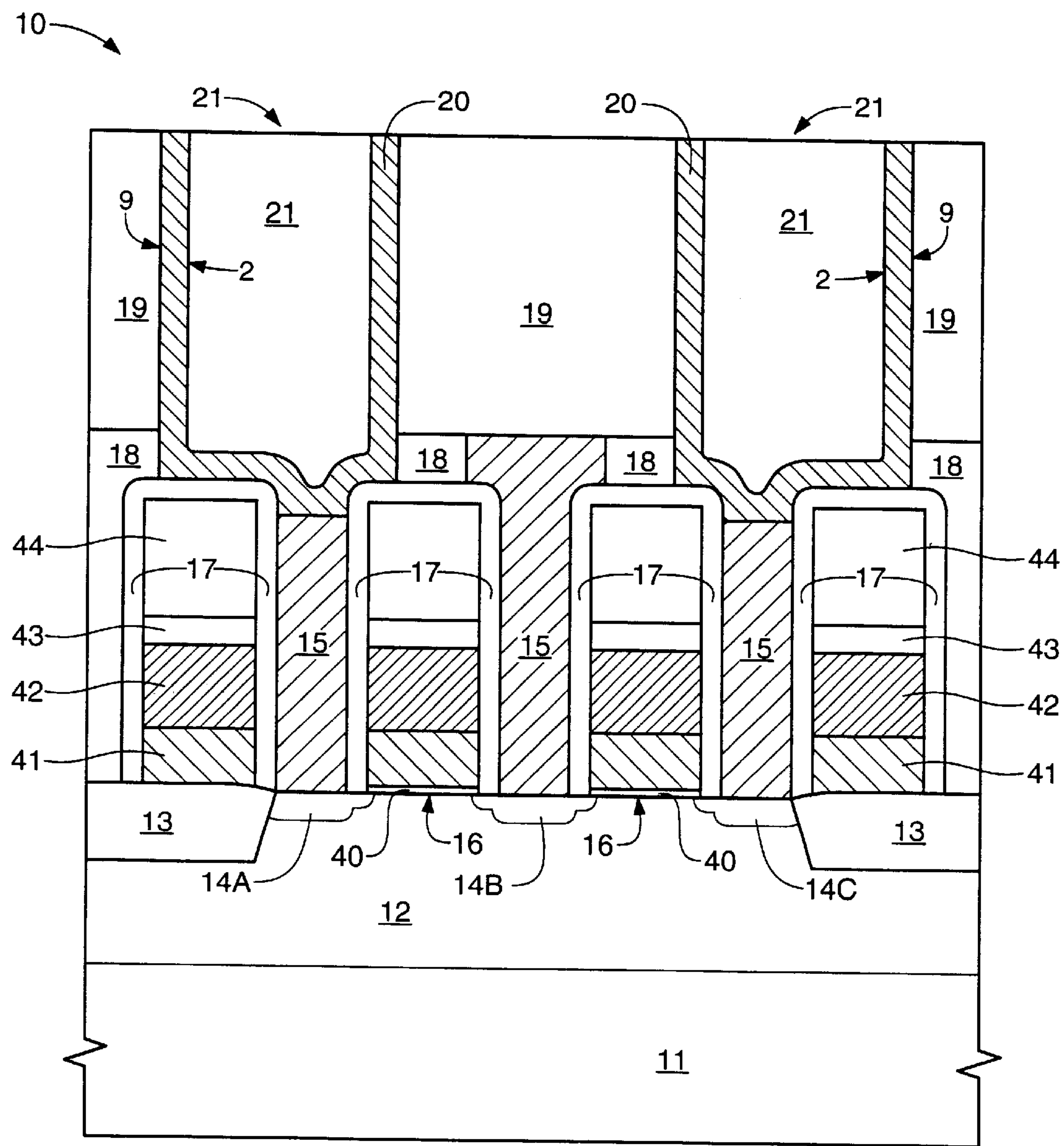
FIG. 6 (PRIOR ART)
