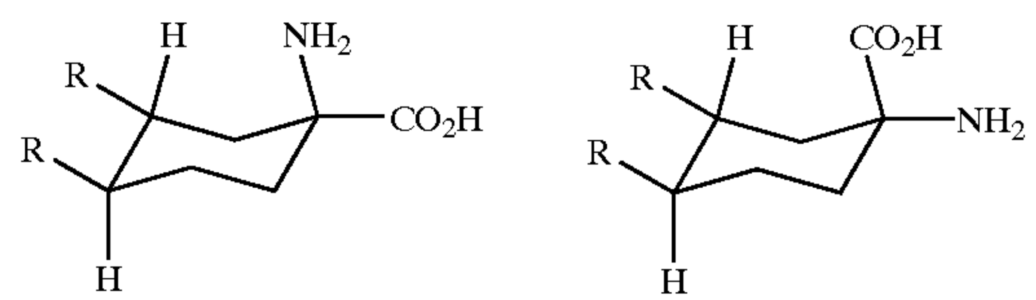
Bucherer-Bergs synthesis ( \beta isomer)
