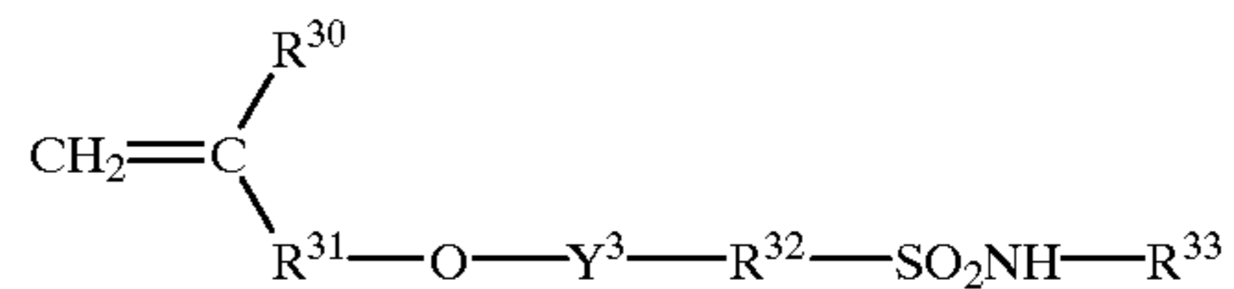
General formula (5)
