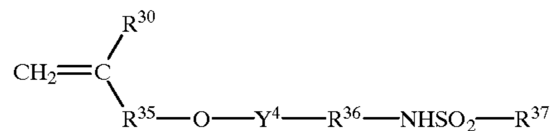
General formula (5)
