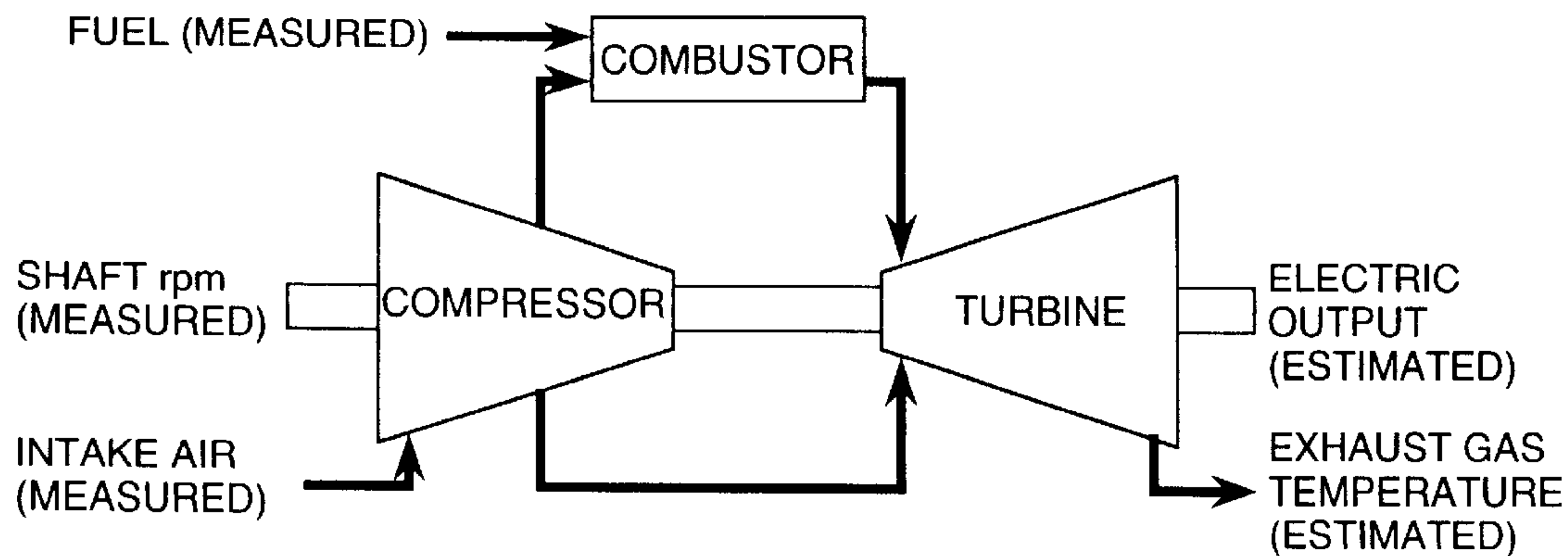
MACHINE MODEL
