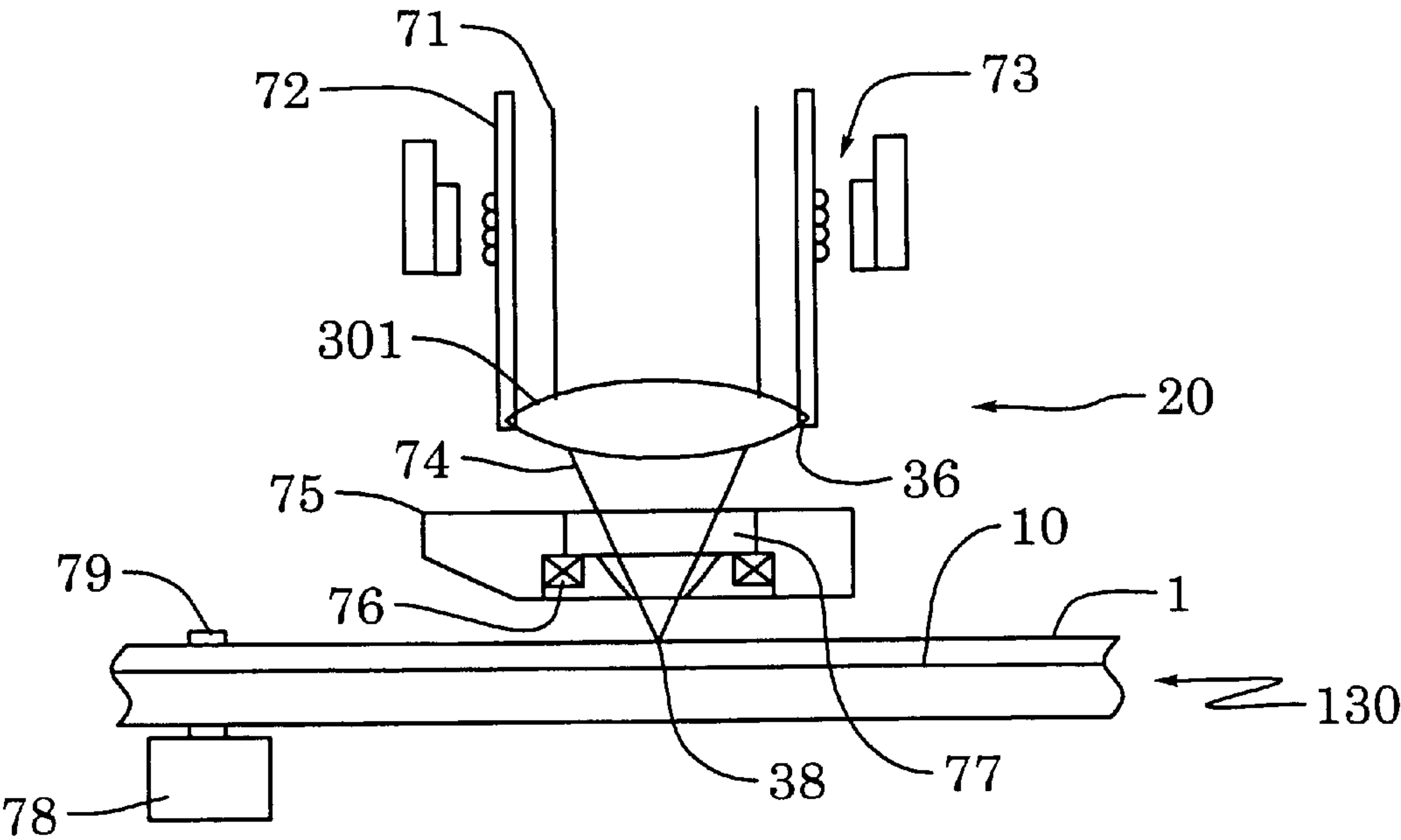
Fig. 21 PRIOR ART
