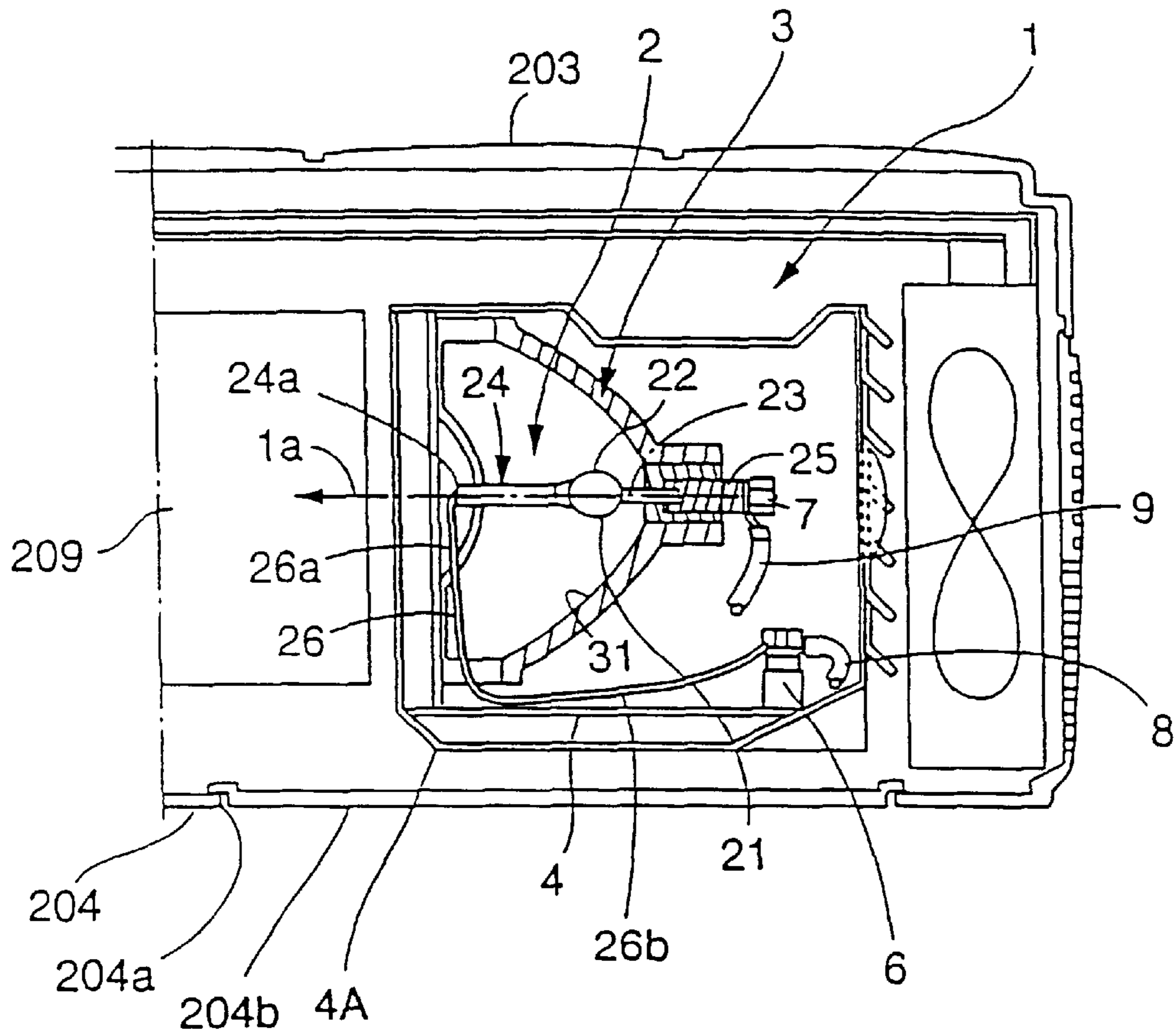
(CROSS SECTION ALONG B-B)
