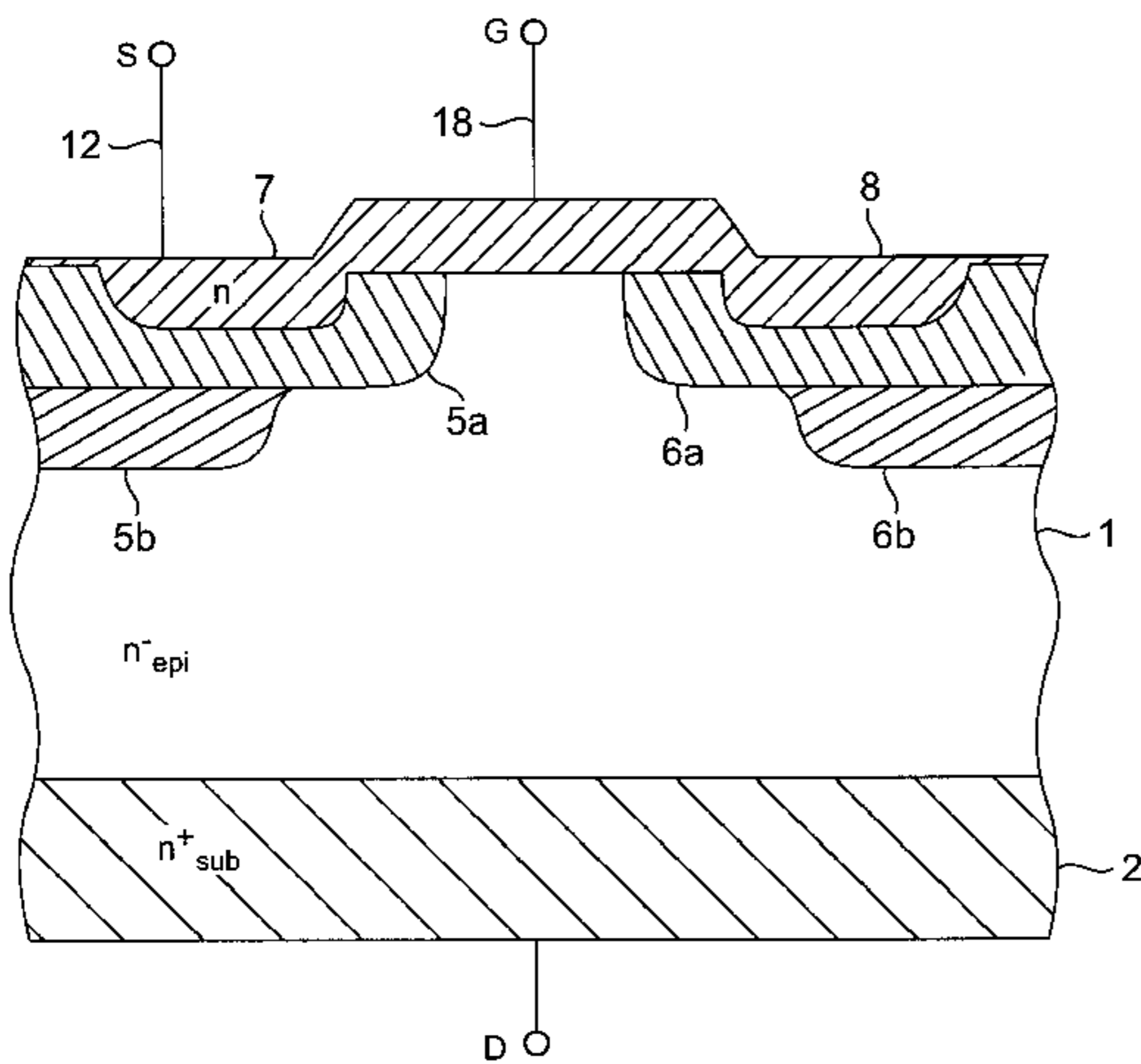
CONVENTIONAL MOSFET
