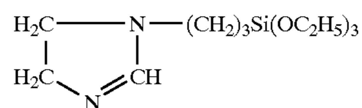
3,4,5-Dihydroimidazol-1-yl-propyl-triethoxysilane
