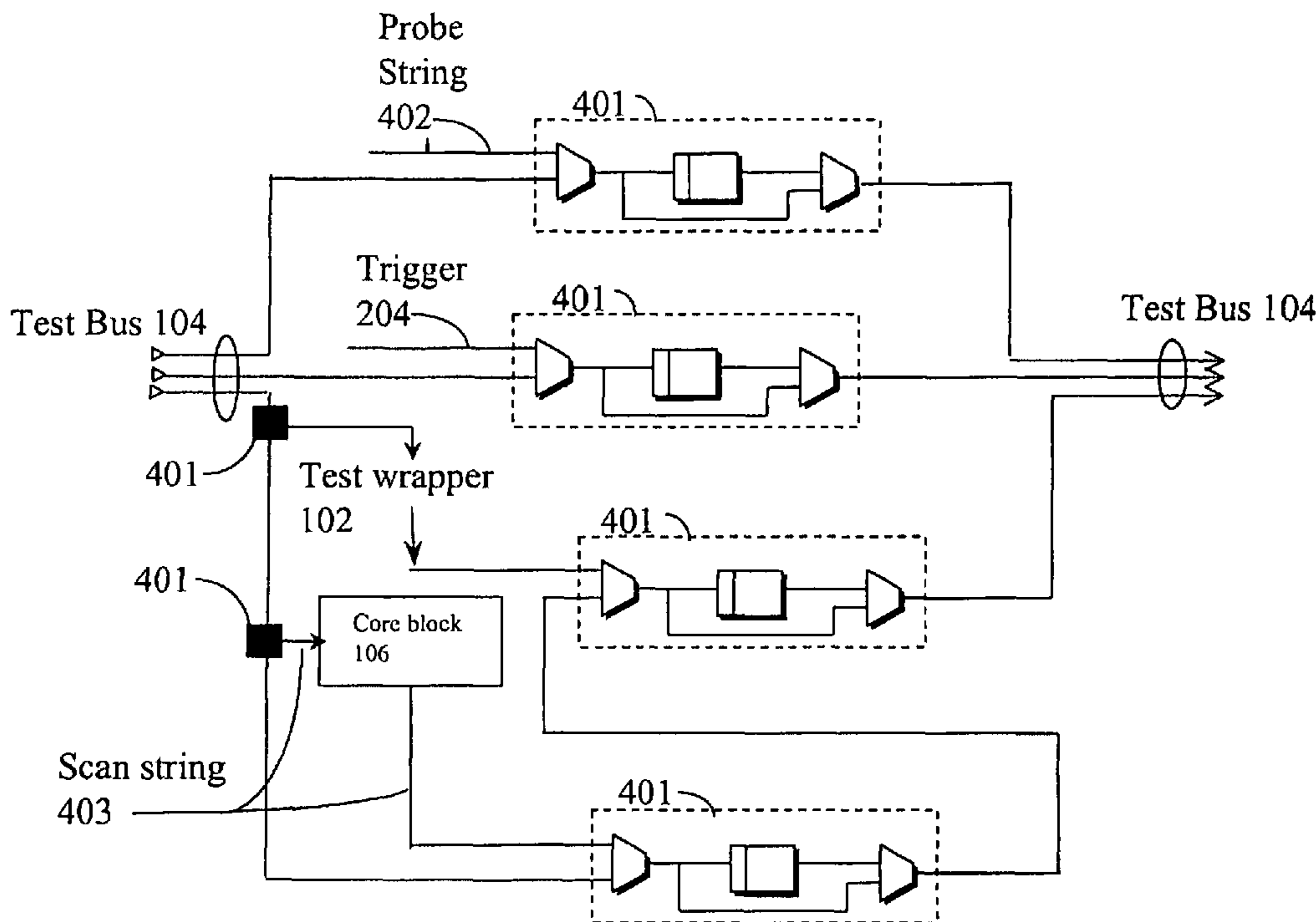
Connecting Probe String, Test Wrapper or Scan String to Test Bus
