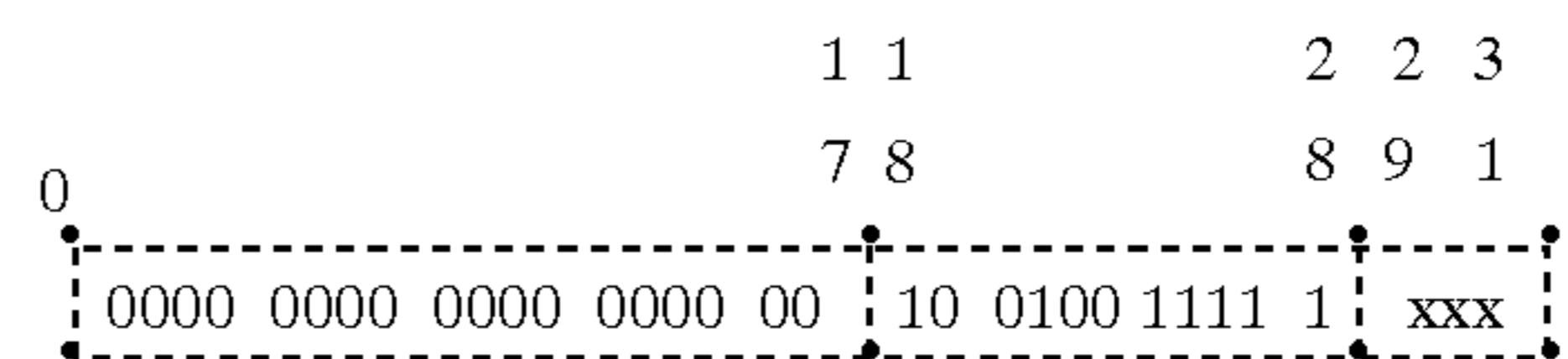
CONTROL UNIT 32 BIT TIMER
