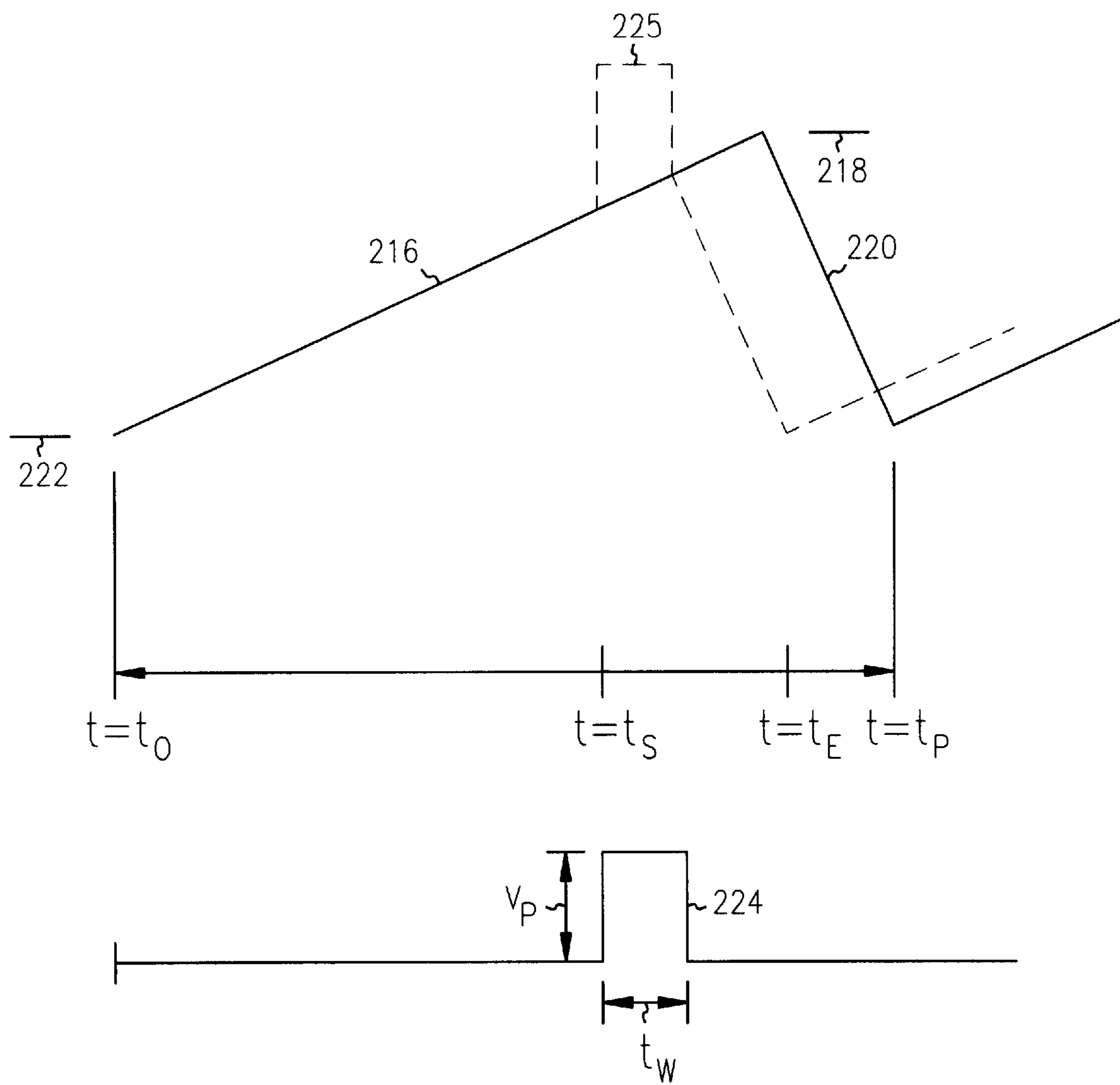
FIG. 2 (PRIOR ART)
