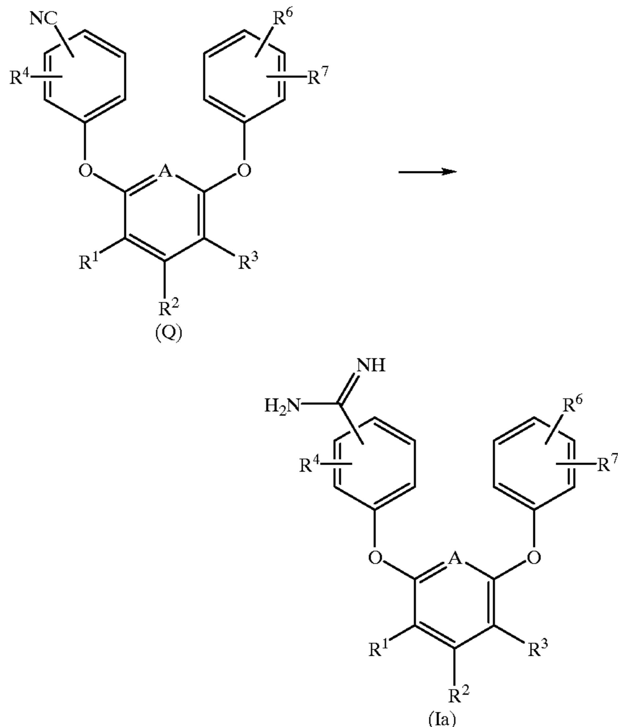
REACTION SCHEME 6
