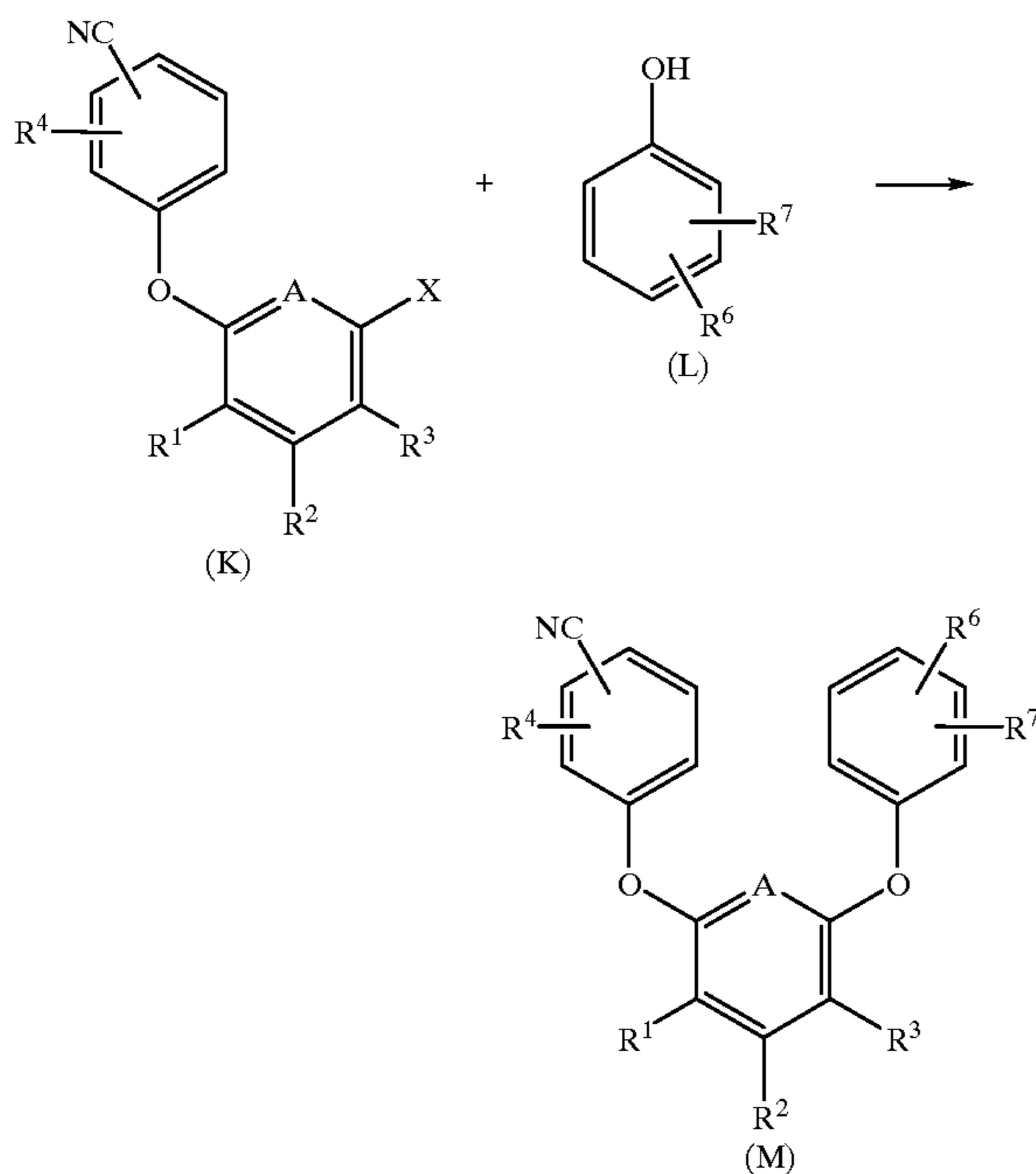
REACTION SCHEME 4
