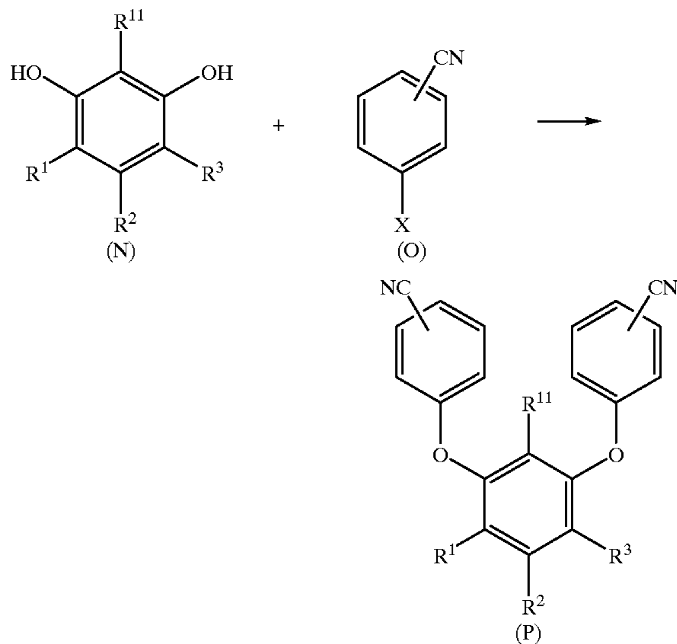
REACTION SCHEME 5
