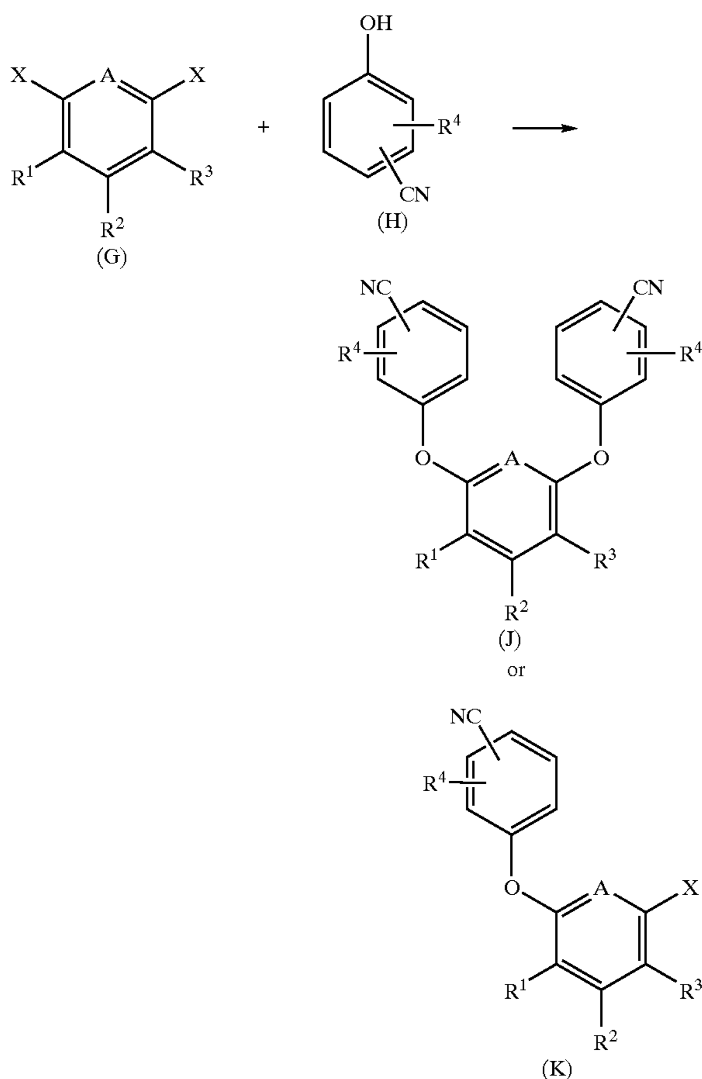
REACTION SCHEME 3
