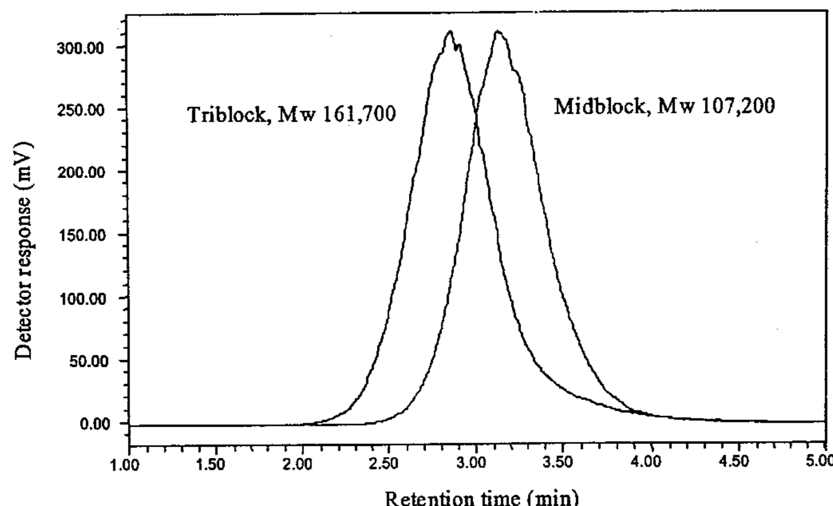
SEC traces of midblock and triblock polymers
