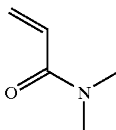
N,N-dimethylacrylamide (DMA)
