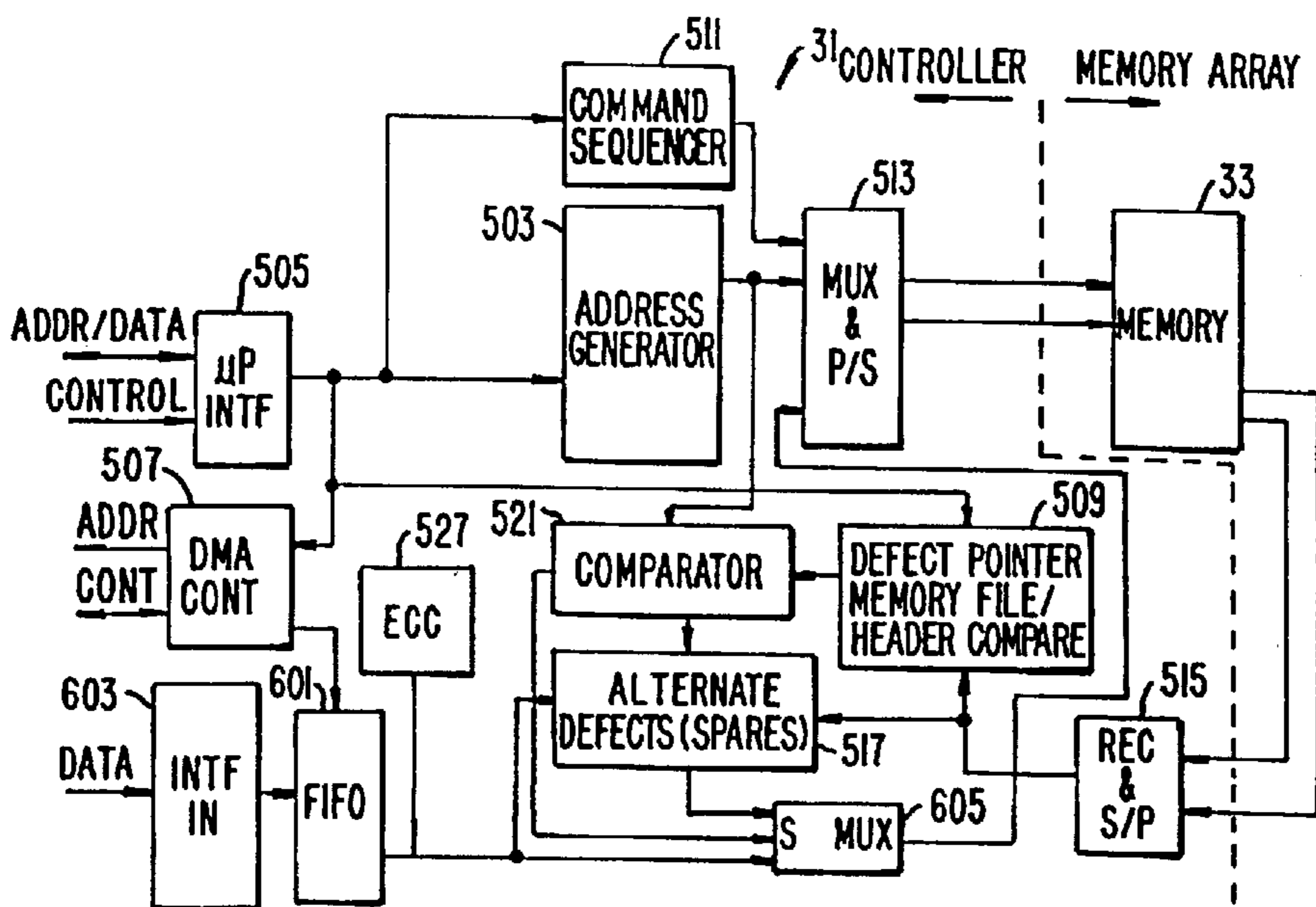
WRITE DATA PATH CONTROL
