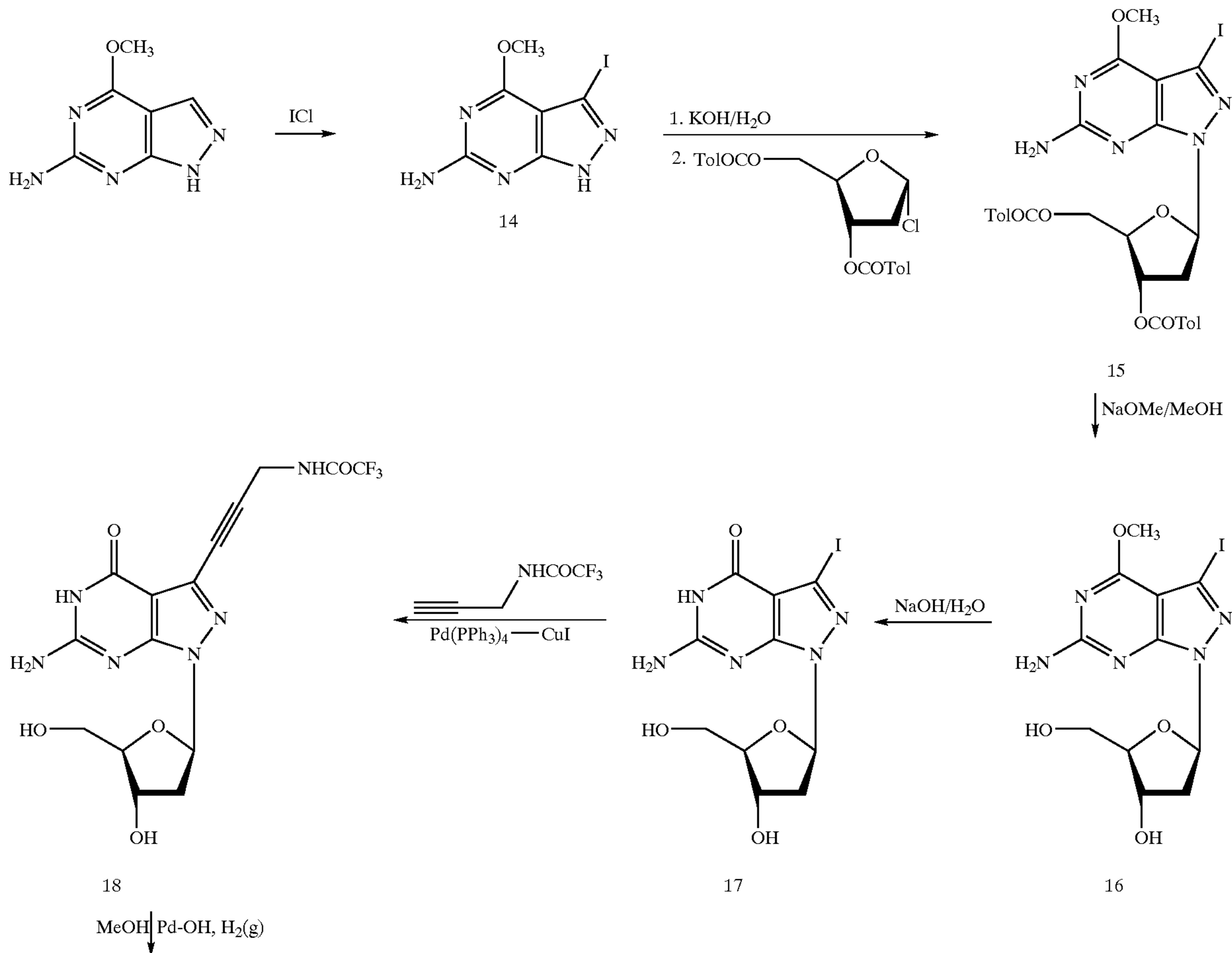
Reaction Scheme 4
