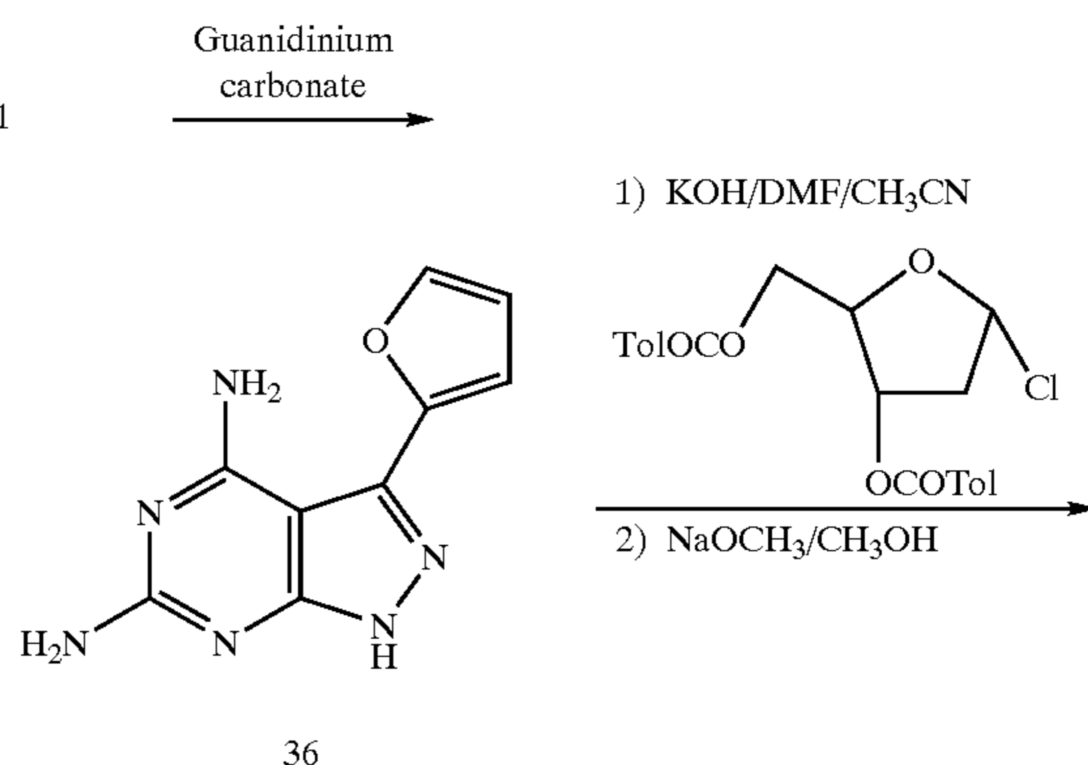
Reaction Scheme 9
