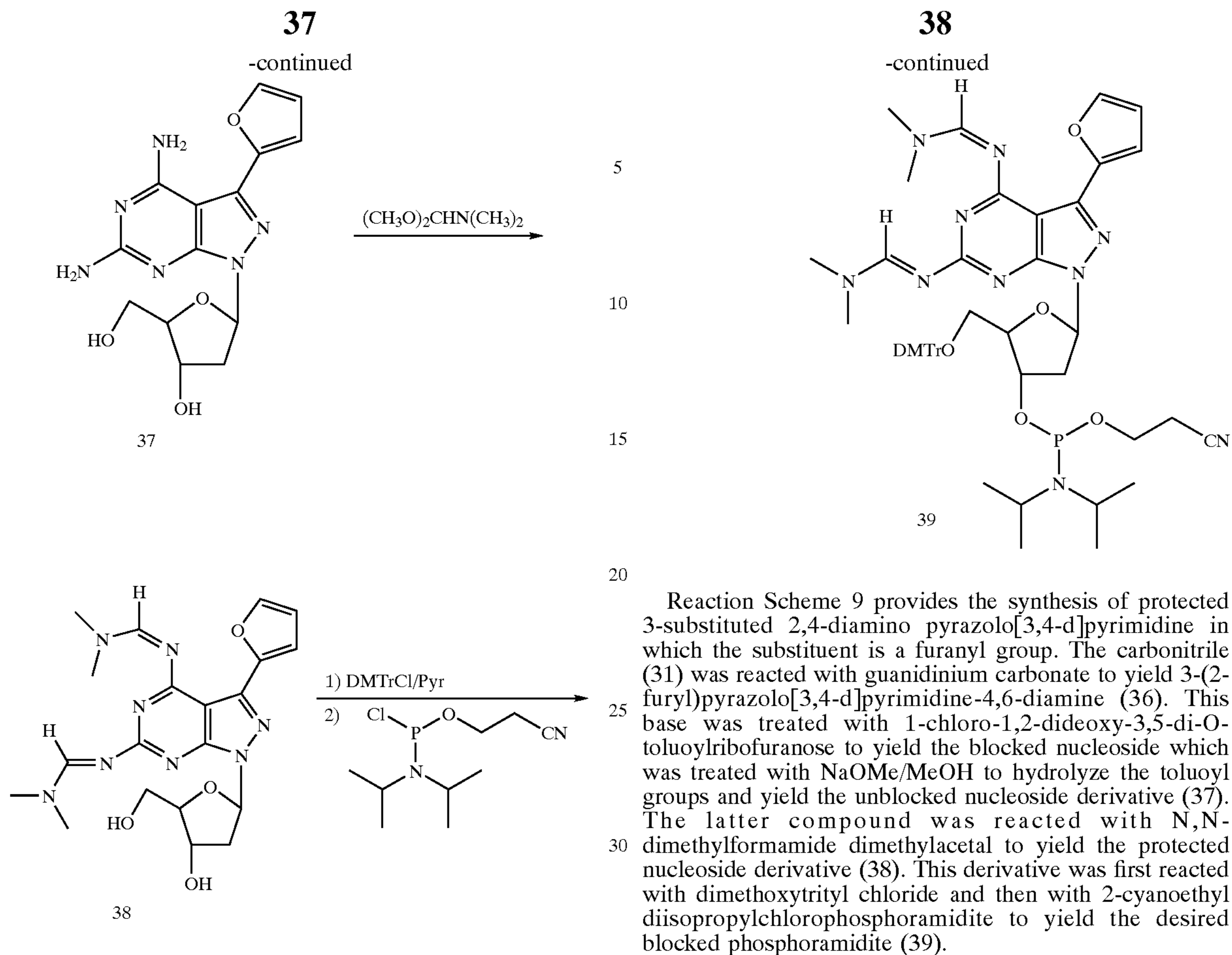
Reaction Scheme 10
