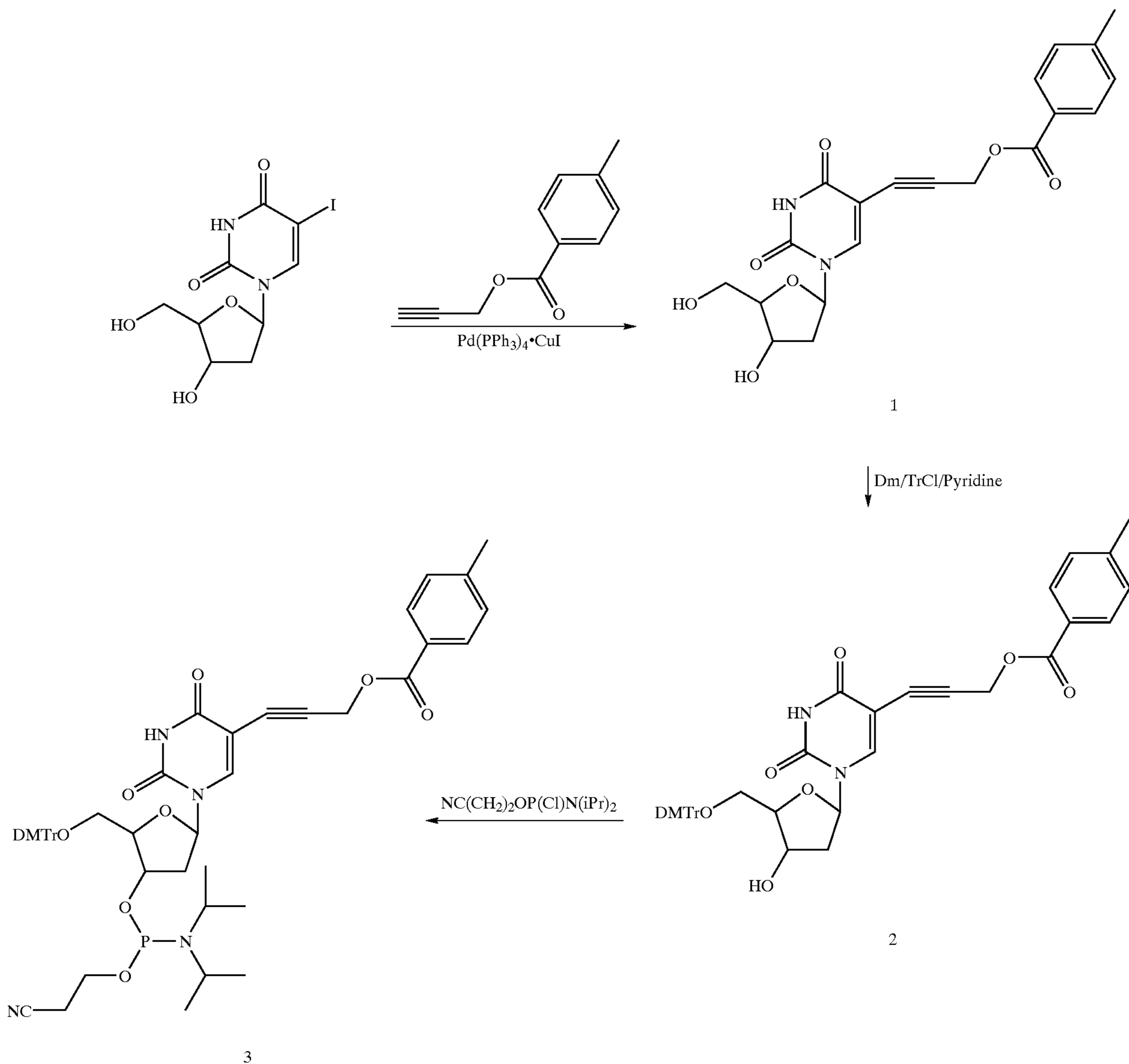
Reaction Scheme 1
