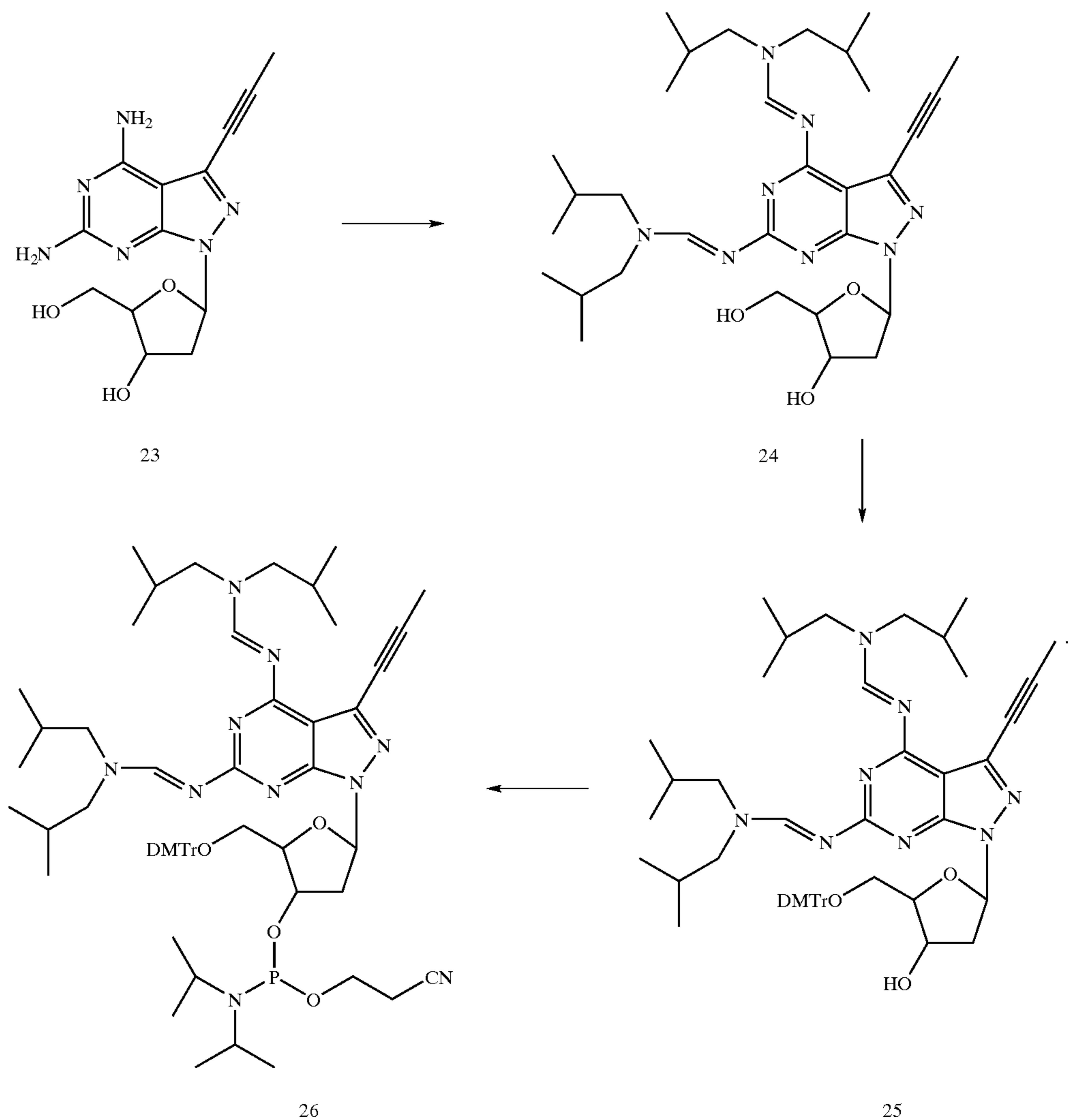
Reaction Scheme 5
