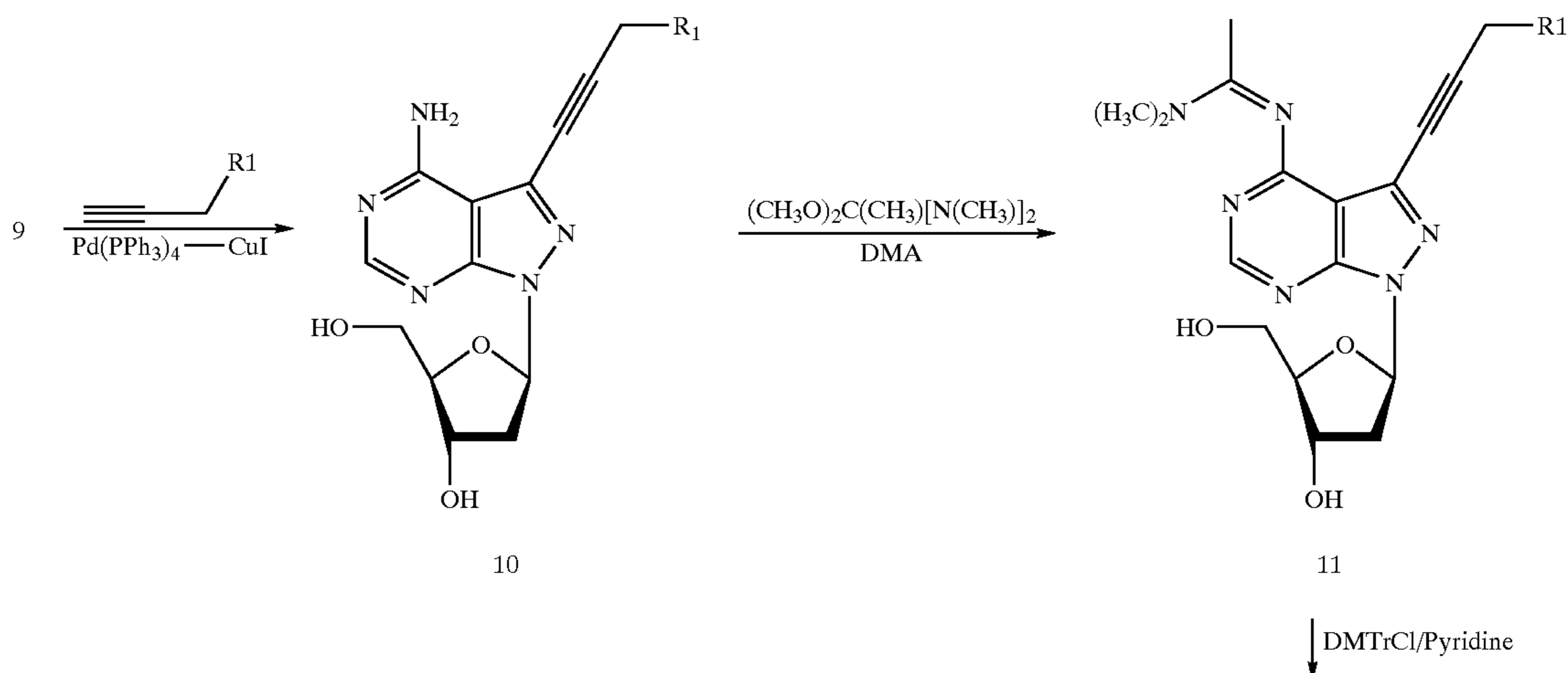
Reaction Scheme 3
