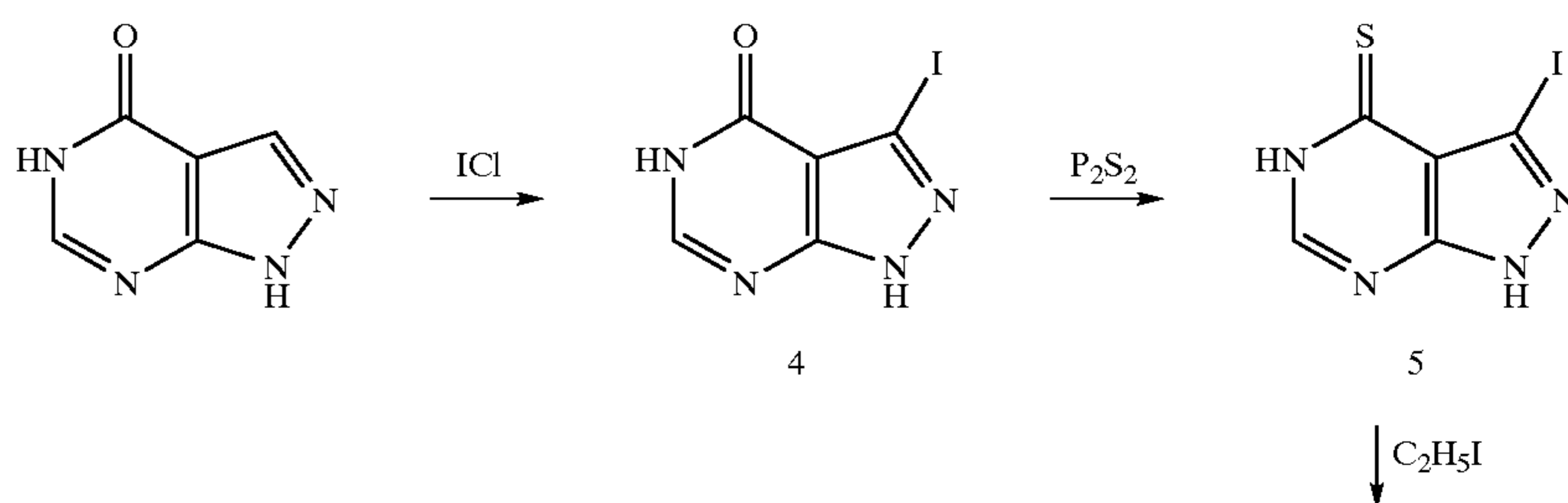
Reaction Scheme 2
