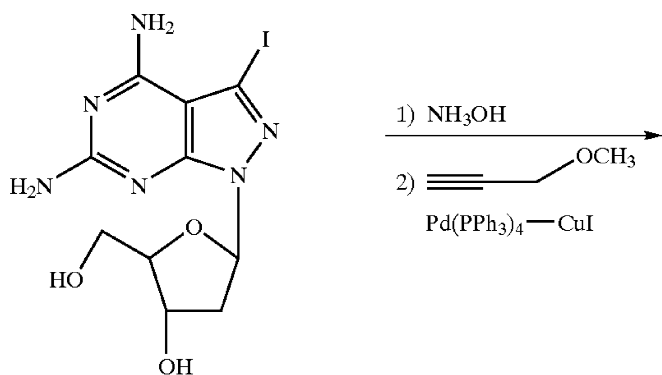
Reaction Scheme 7
