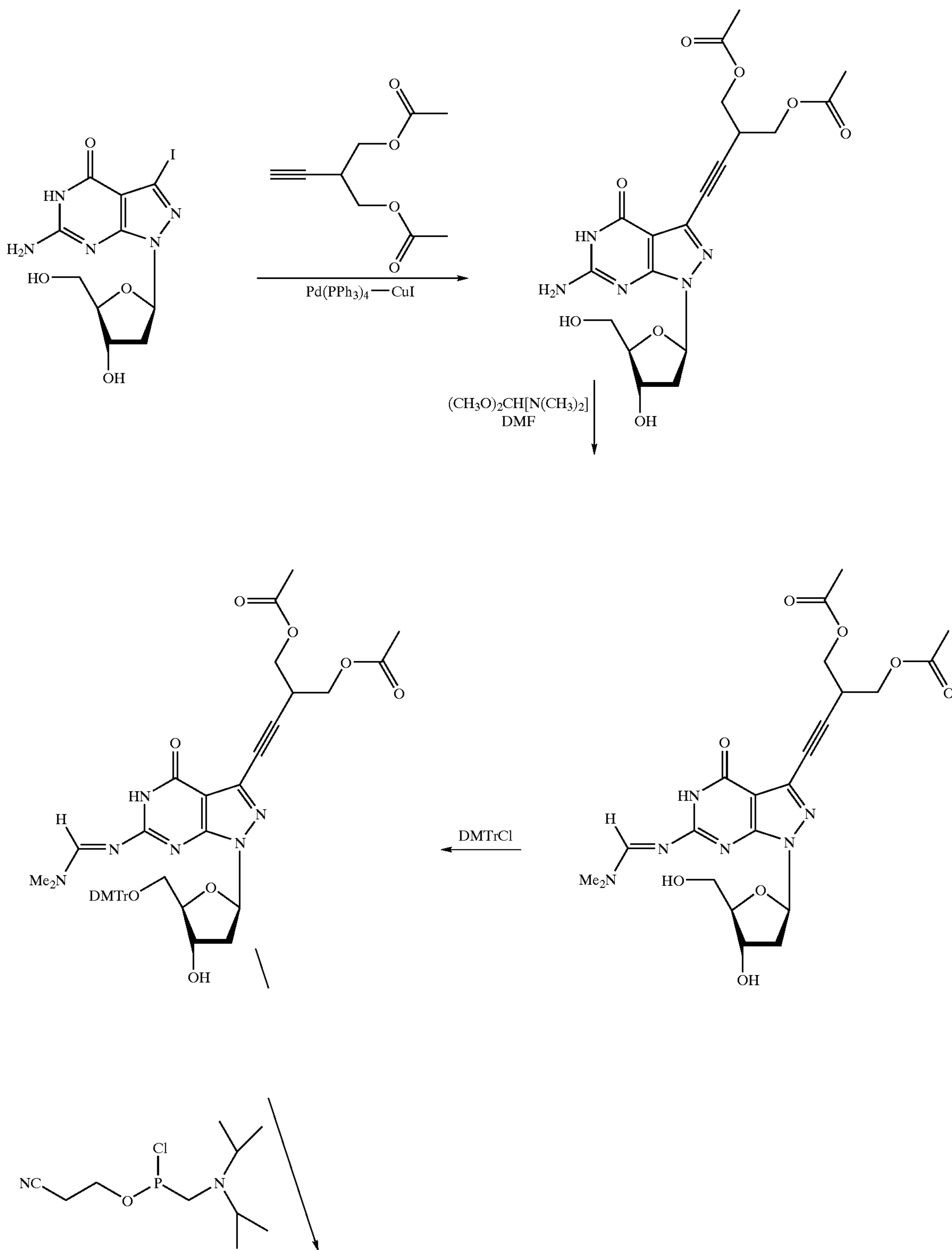
Reaction Scheme 6
