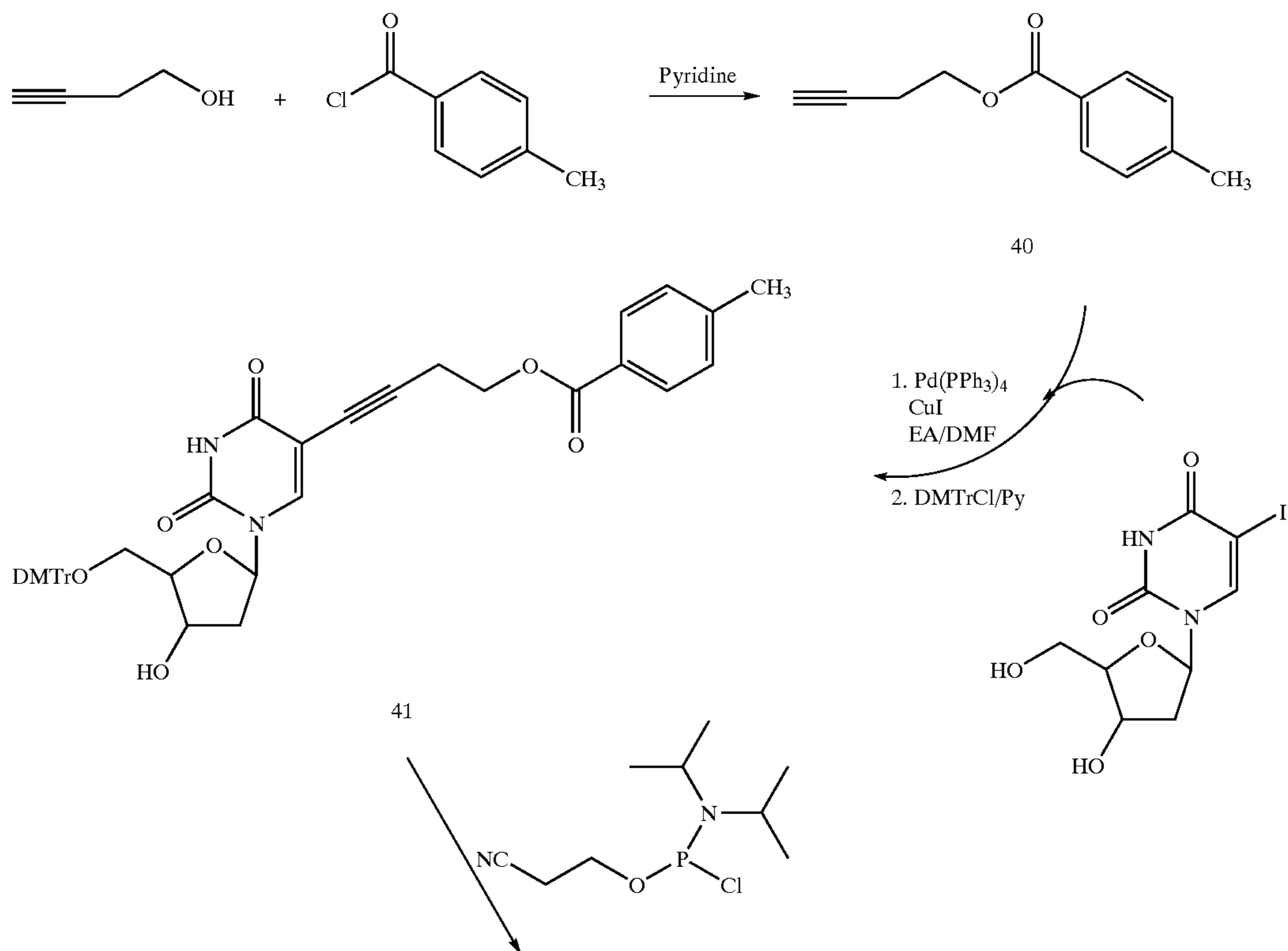
Reaction Scheme 10
