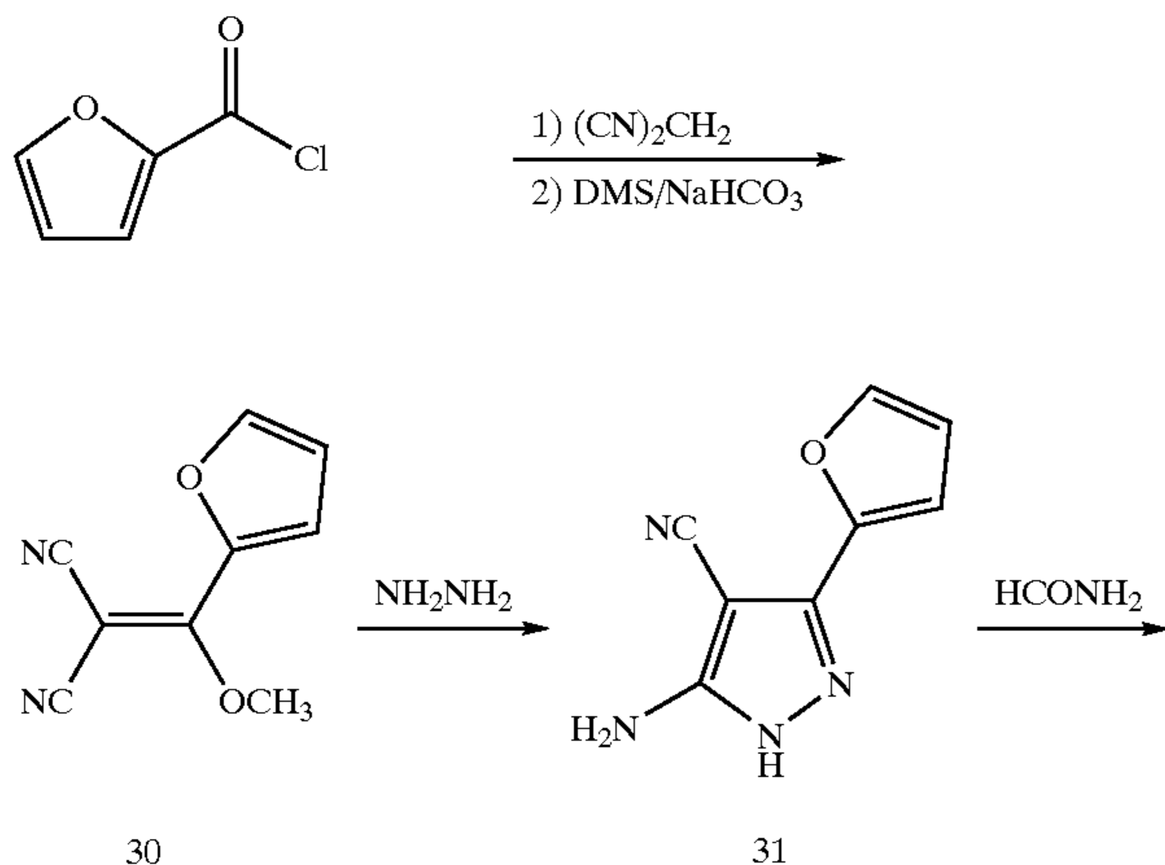
Reaction Scheme 8
