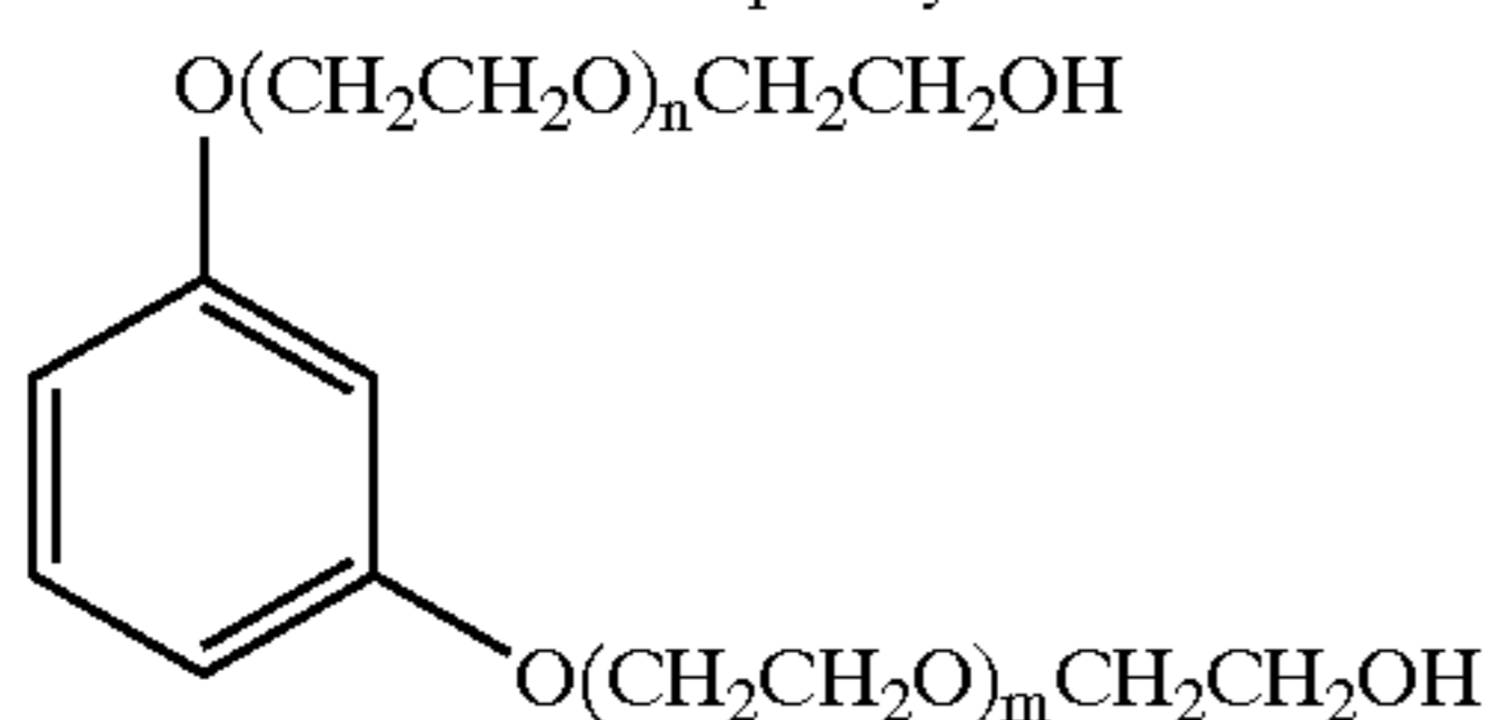
FIG. 1: o-phenylene
