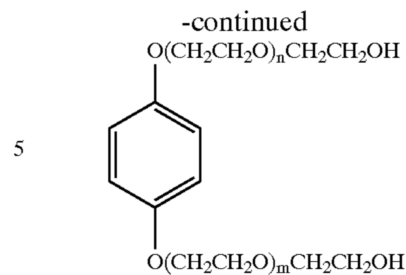
FIG. 3: p-phenylene
