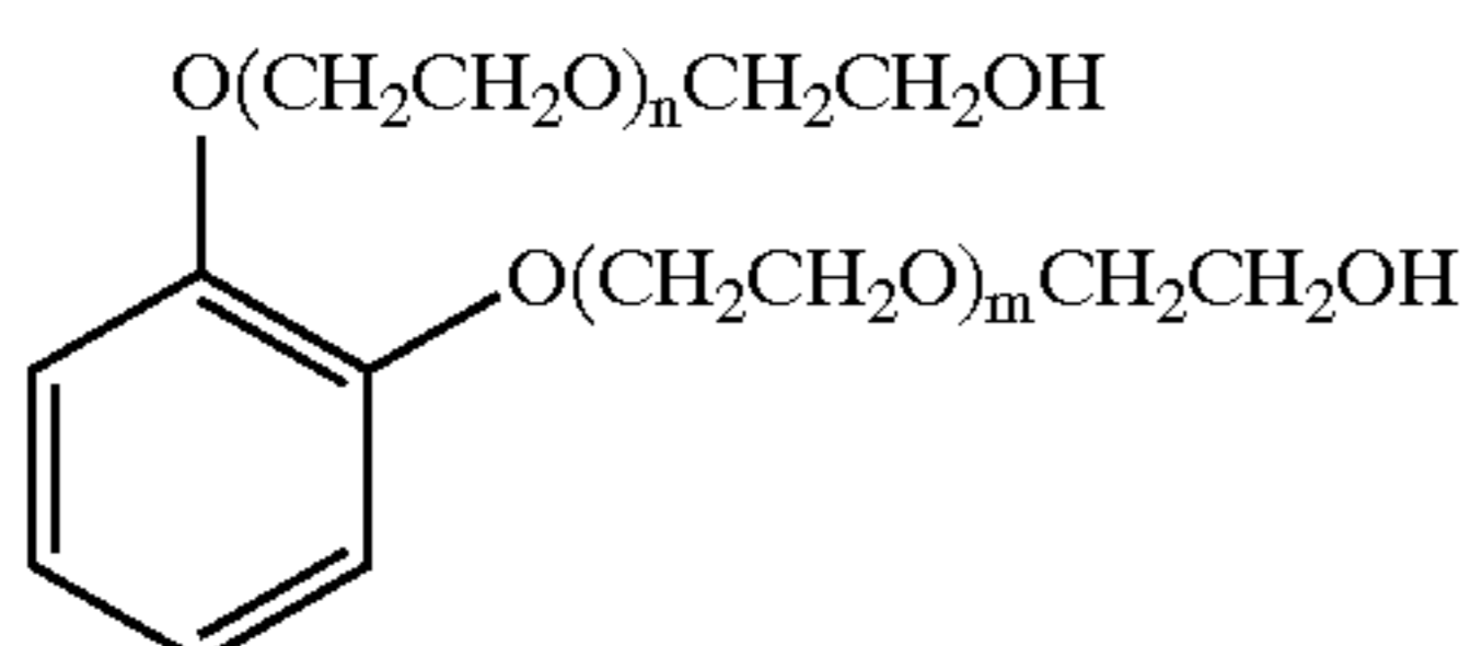
FIG. 1: o-phenylene
