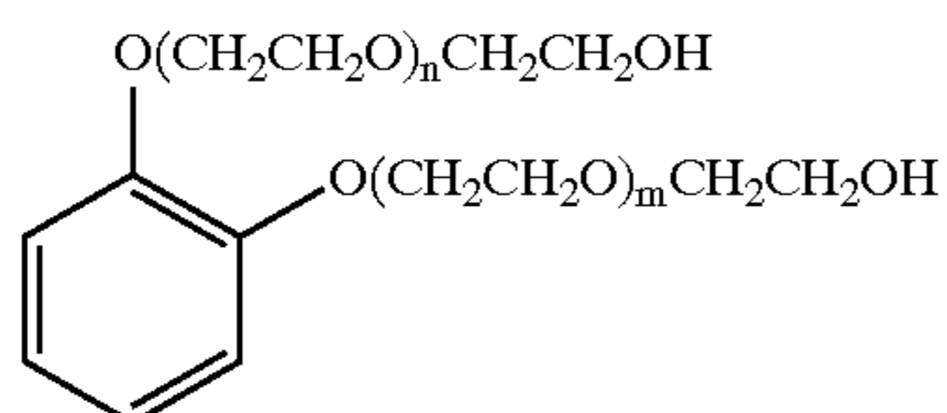
FIG. 1: o-phenylene
