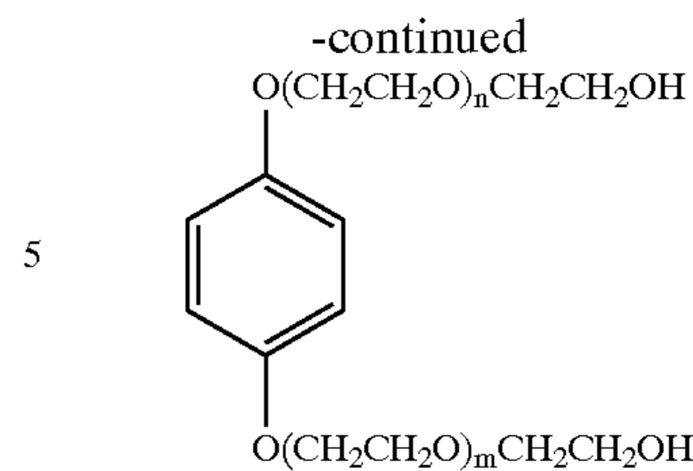
FIG. 3: p-phenylene
