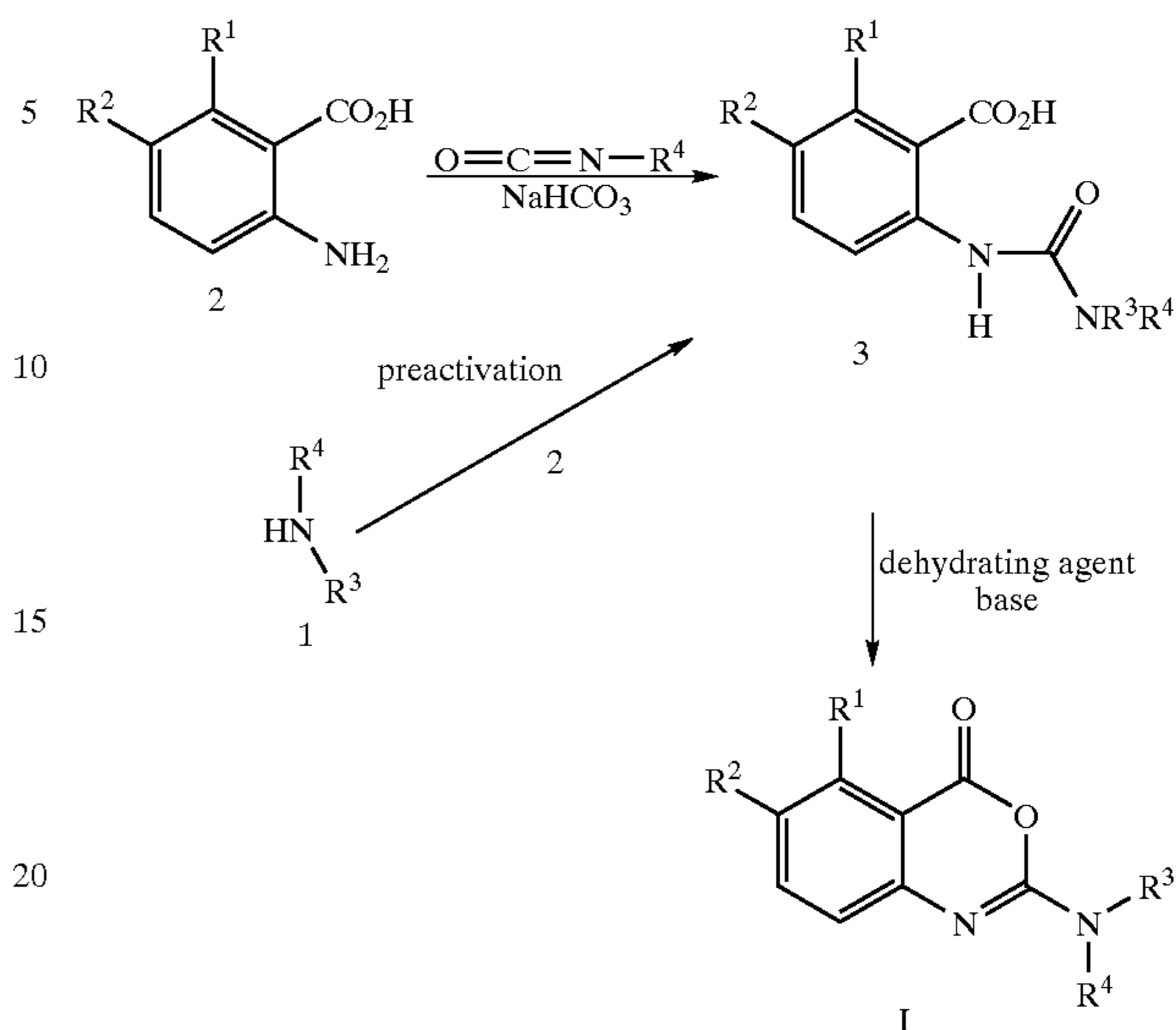
Scheme I
