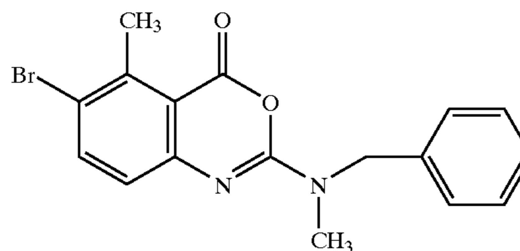
6-Bromo-5-methyl-2-[methyl(phenylmethyl)amino]-4H-3,1-benzoxazin-4-one
