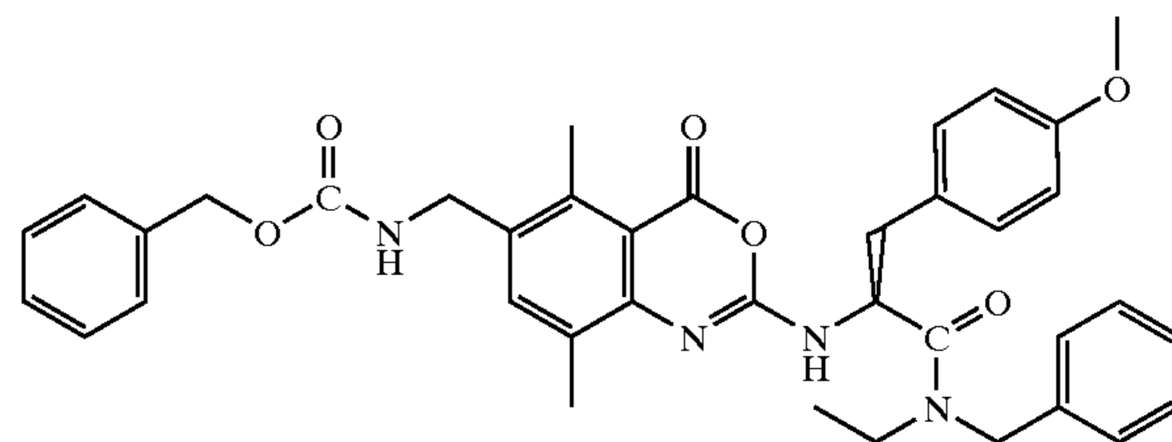
Phenylmethyl[[2-[[2-[ethyl(phenylmethyl)amino]-1S-[(4-methoxyphenyl)methyl]-2-oxoethyl]amino]-5,8-dimethyl-4-oxo-4H-3,1-benzoxazin-6-yl]methyl]carbamate
