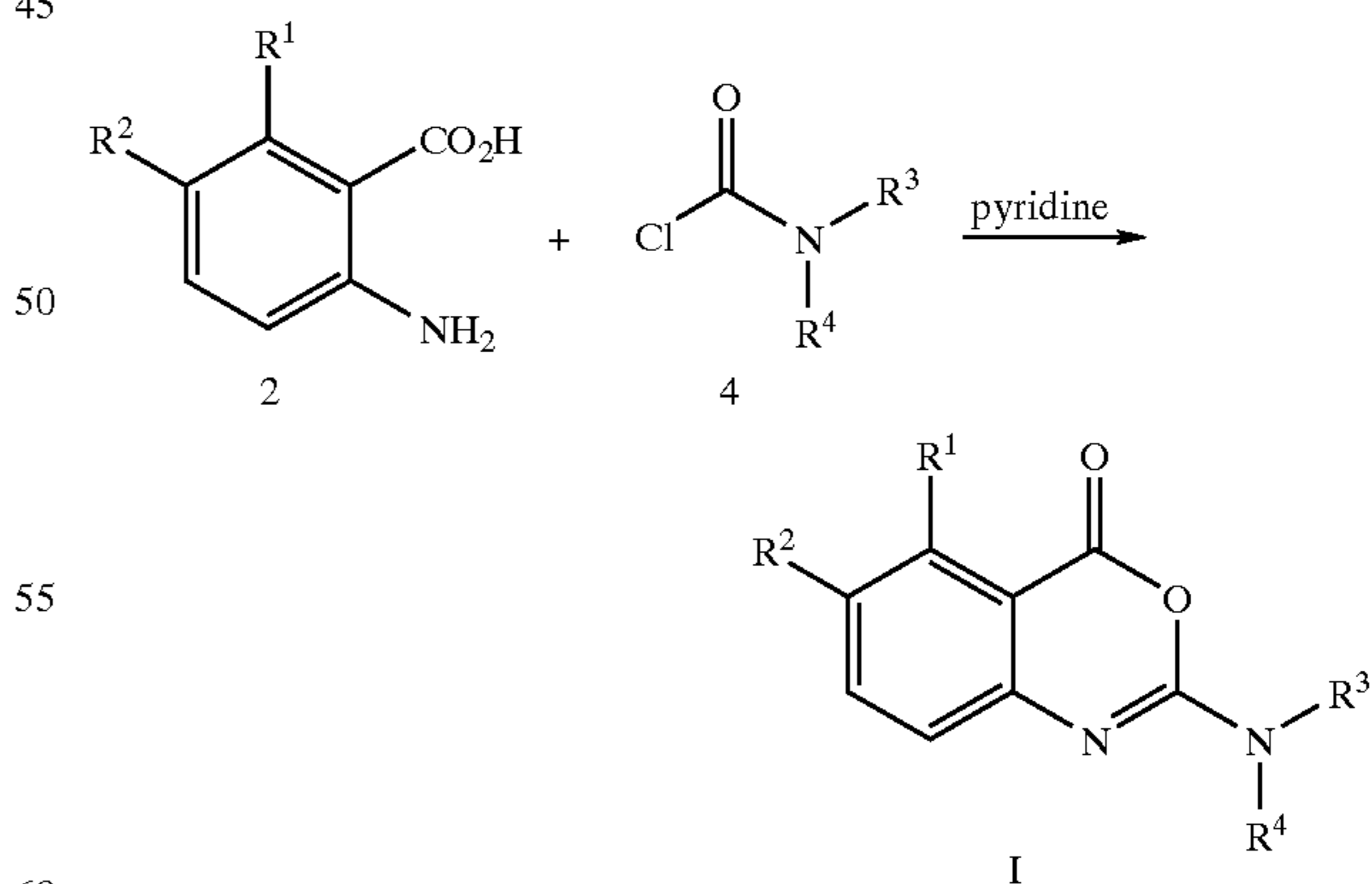
Scheme II
