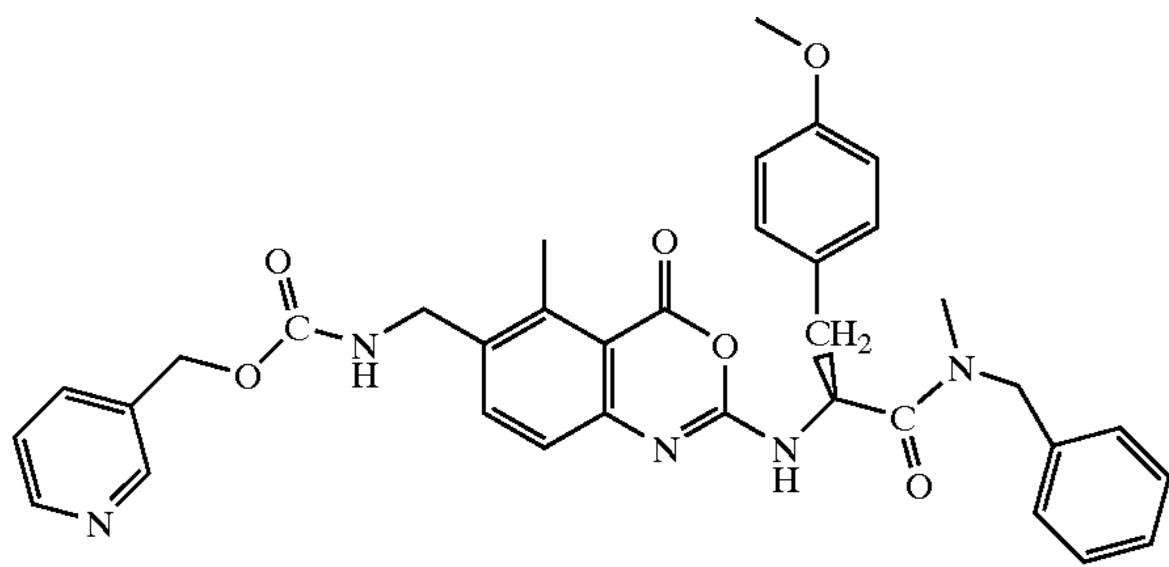
3-Pyridinylmethyl[[2-[[1S-[(4-methoxyphenyl)methyl]-2-[methyl(phenylmethyl)amino]-2-oxoethyl]amino]-5-methyl-4-oxo-4H-3,1-benzoxazin-6-yl]methyl]carbamate
