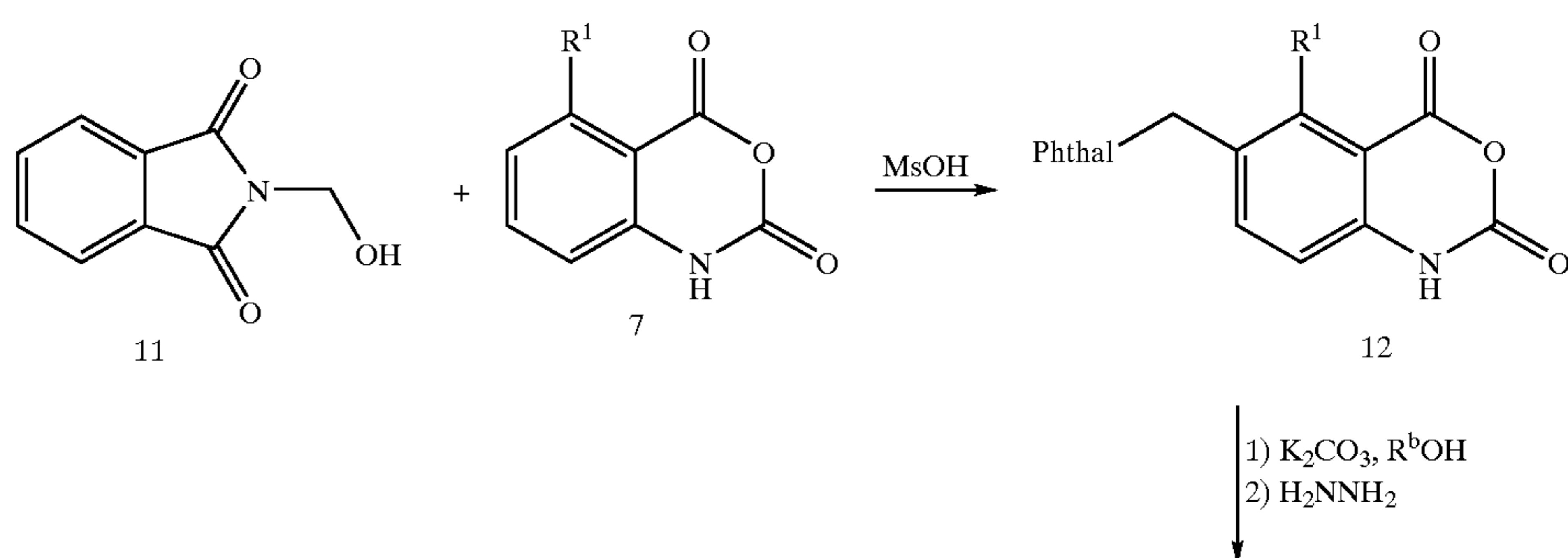
Scheme V
