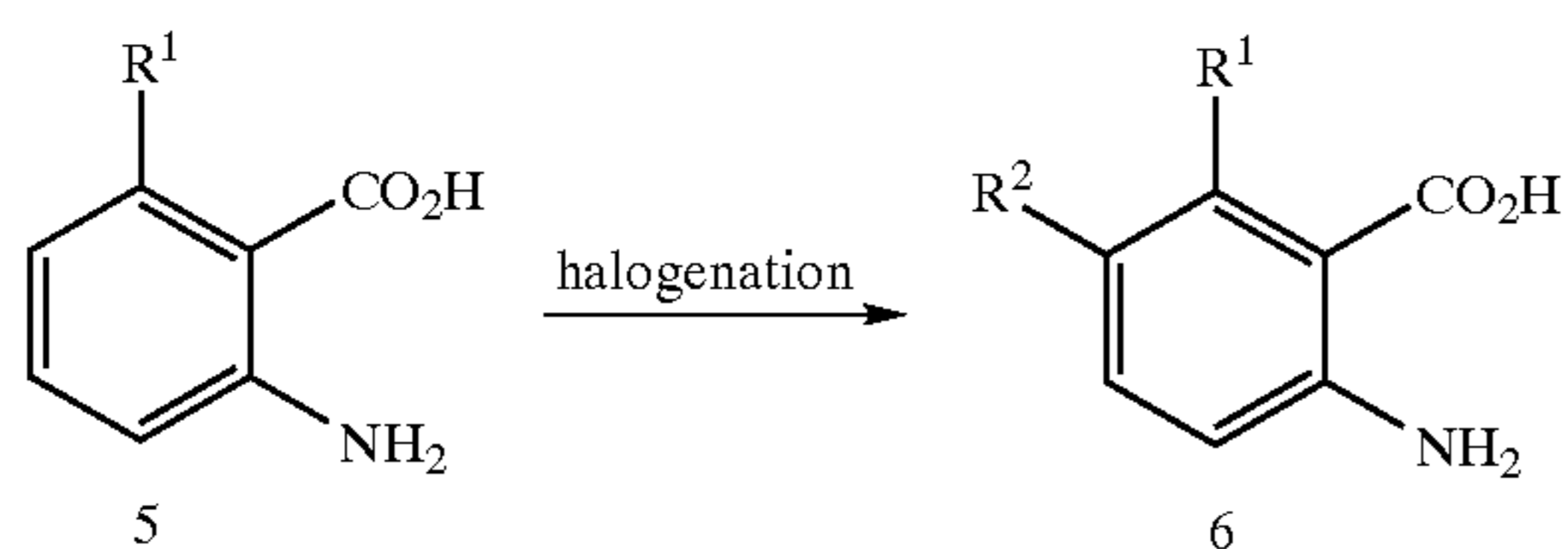
Scheme III
