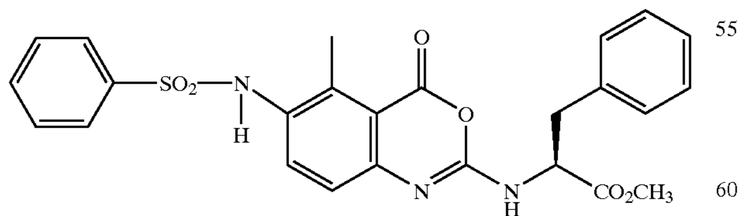
N-[6-[Benzenesulfonyl]amino]-5-methyl-4-oxo-4H-3,1-benzoxazin-2-yl]-L-phenylalanine, Methyl Ester
