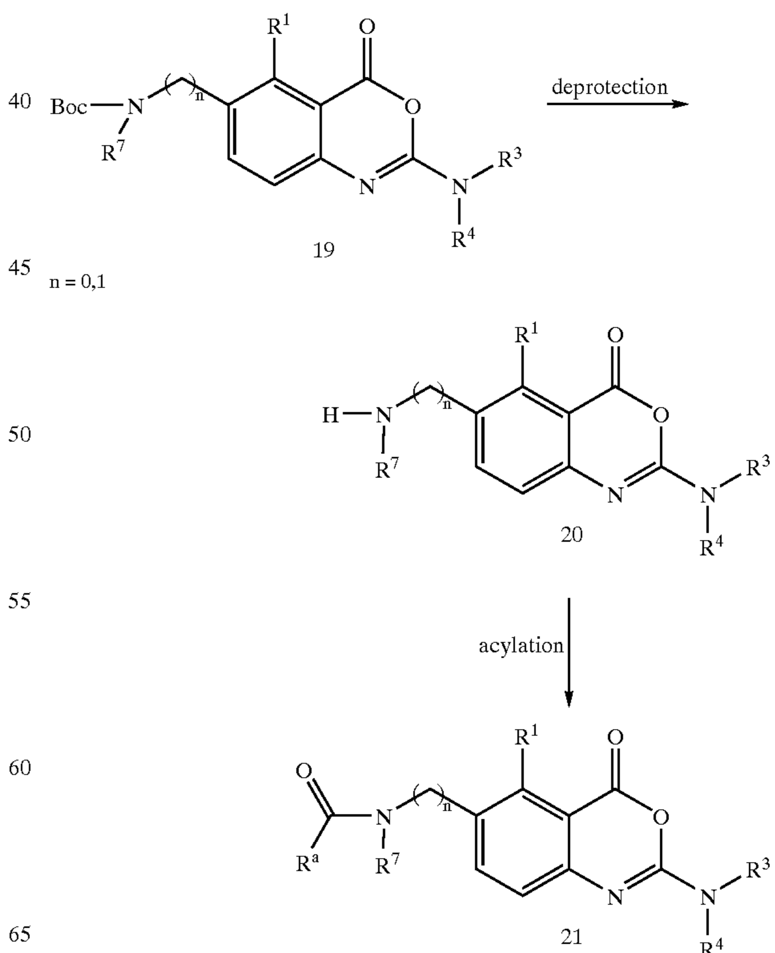
Scheme VII
