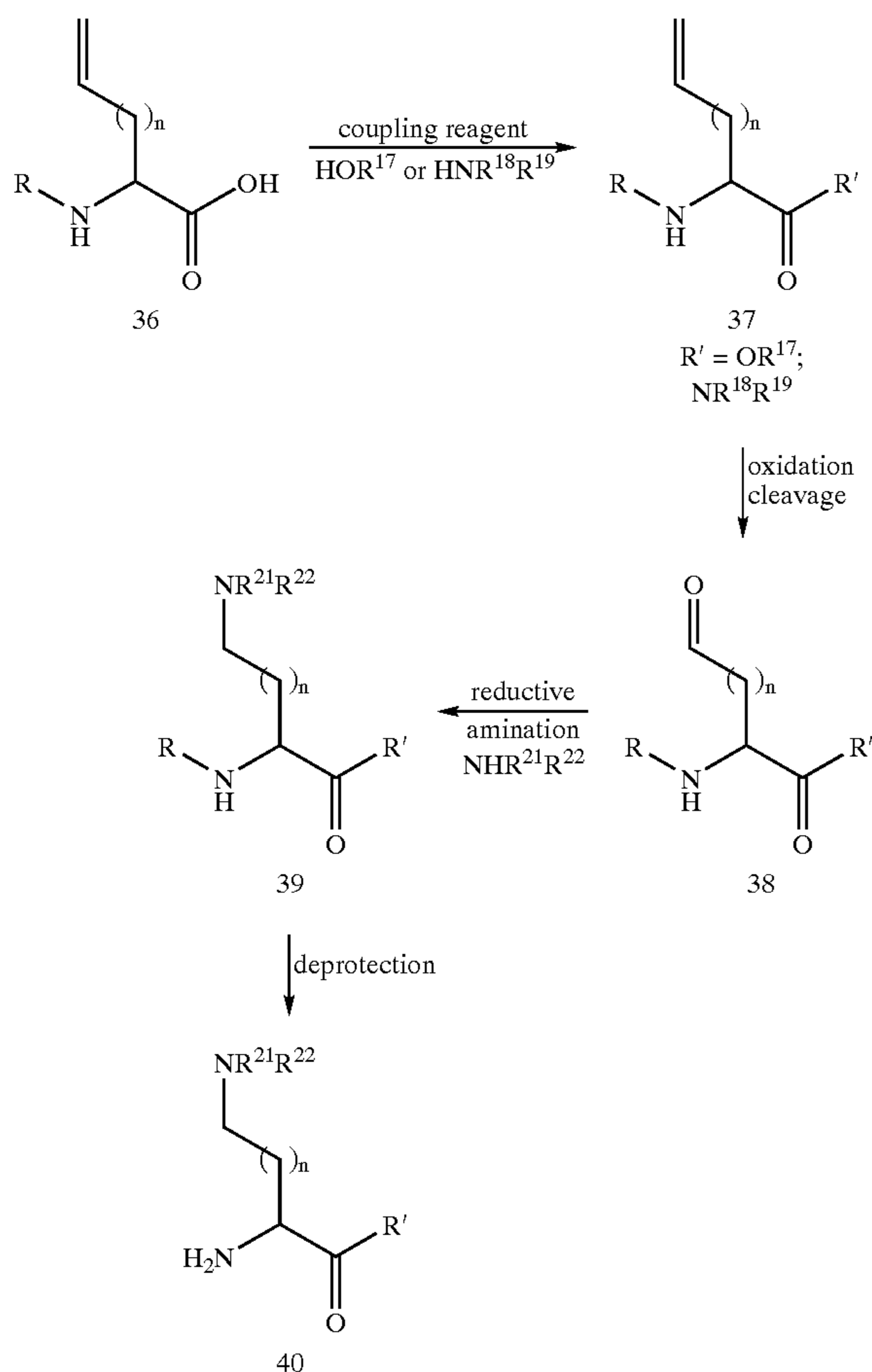
Scheme XIII
