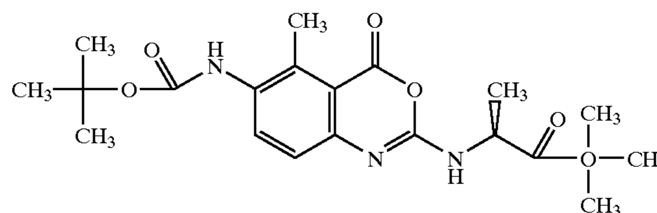
N-[6-[[[(1,1-Dimethylethoxy)carbonyl]amino]-5-methyl-4-oxo-4H-3,1-benzoxazin-2-yl]-L-alanine, 1-dimethylethyl Ester
