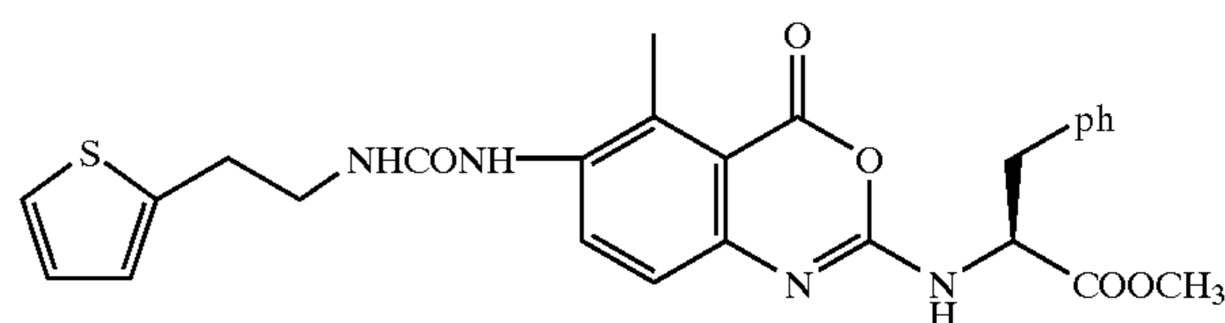
N-[6-[[[2-(2-Thienyl)ethyl]amino]carbonyl]amino]-5-methyl-4-oxo-4H-3,1-benzoxazin-2-yl]-L-phenylalanine, Methyl Ester
