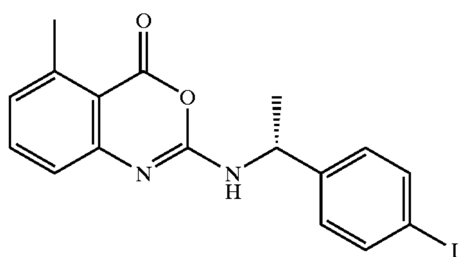
5-Methyl-2-[[1R)-(4-iodophenyl)ethyl]amino]-4H-3,1-benzoxazin-4-one
