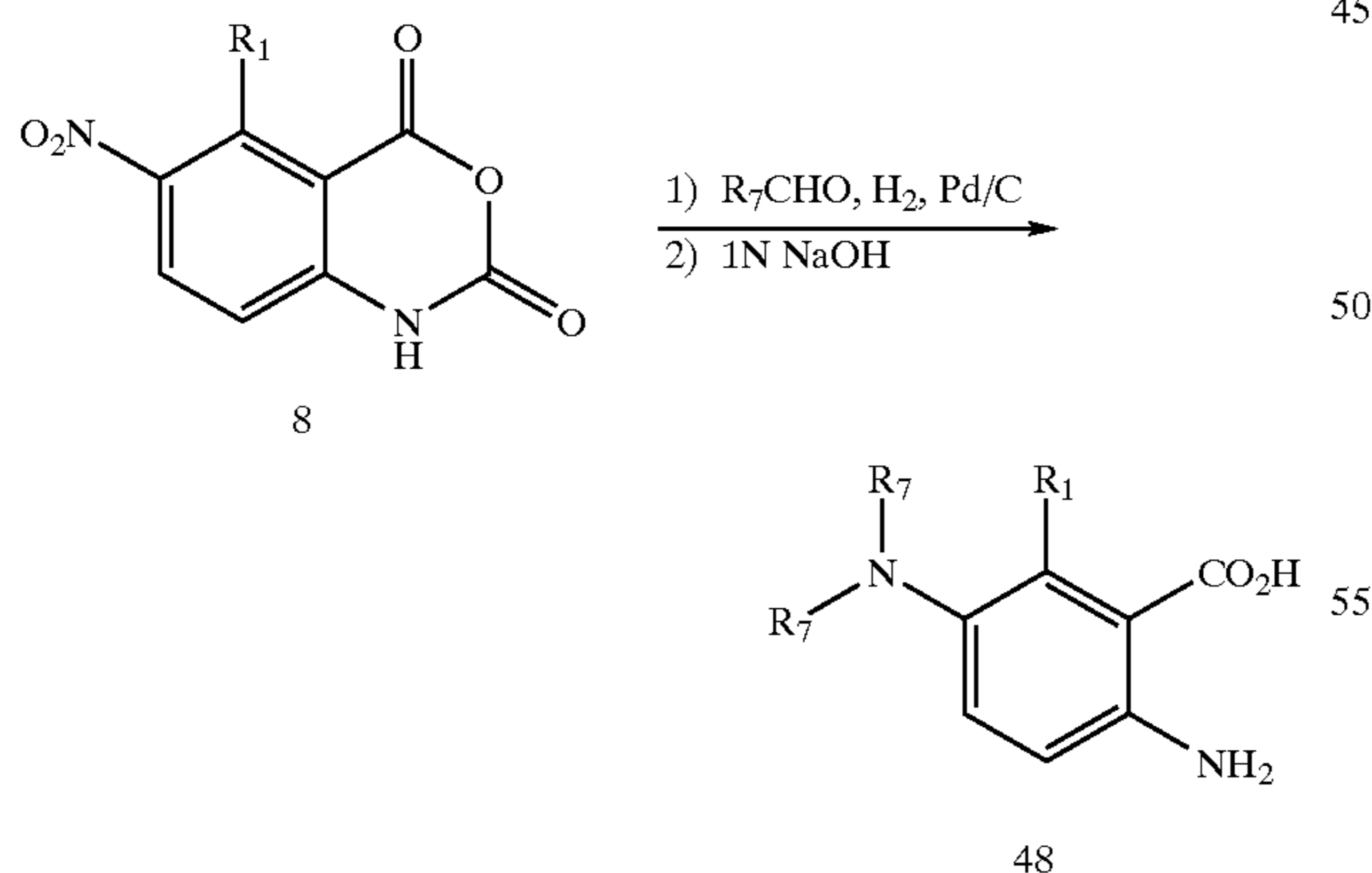
Scheme XVI
