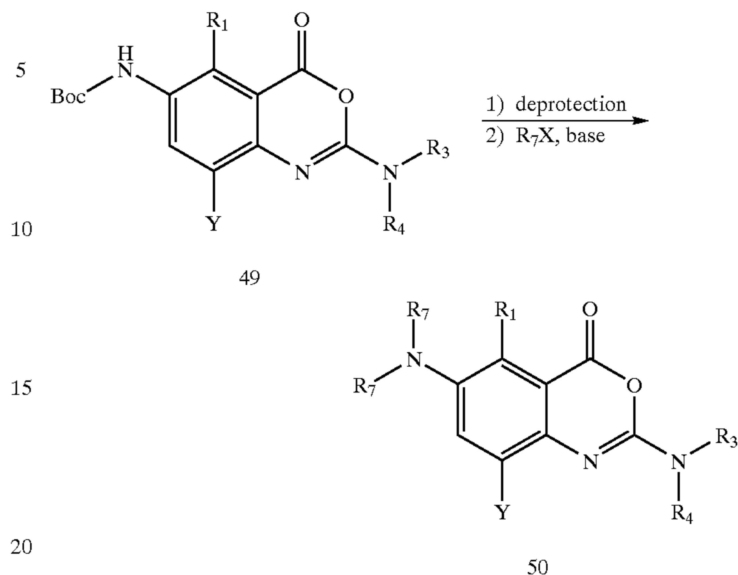
Scheme XVII
