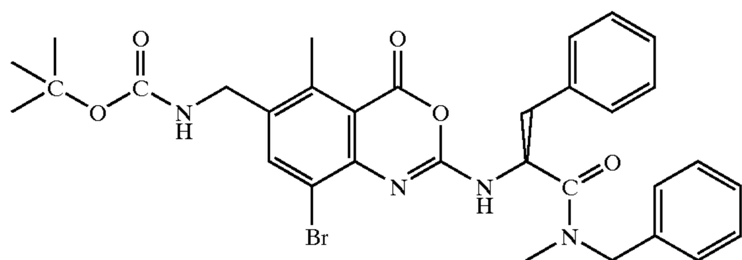
1,1-Dimethylethyl[[8-bromo-5-methyl-2-[[2-[methyl(phenylmethyl)amino]-2-oxo-1S-(phenylmethyl)ethyl]amino]-4-oxo-4H-3,1-benzoxazin-6-yl]methyl] Carbamate
