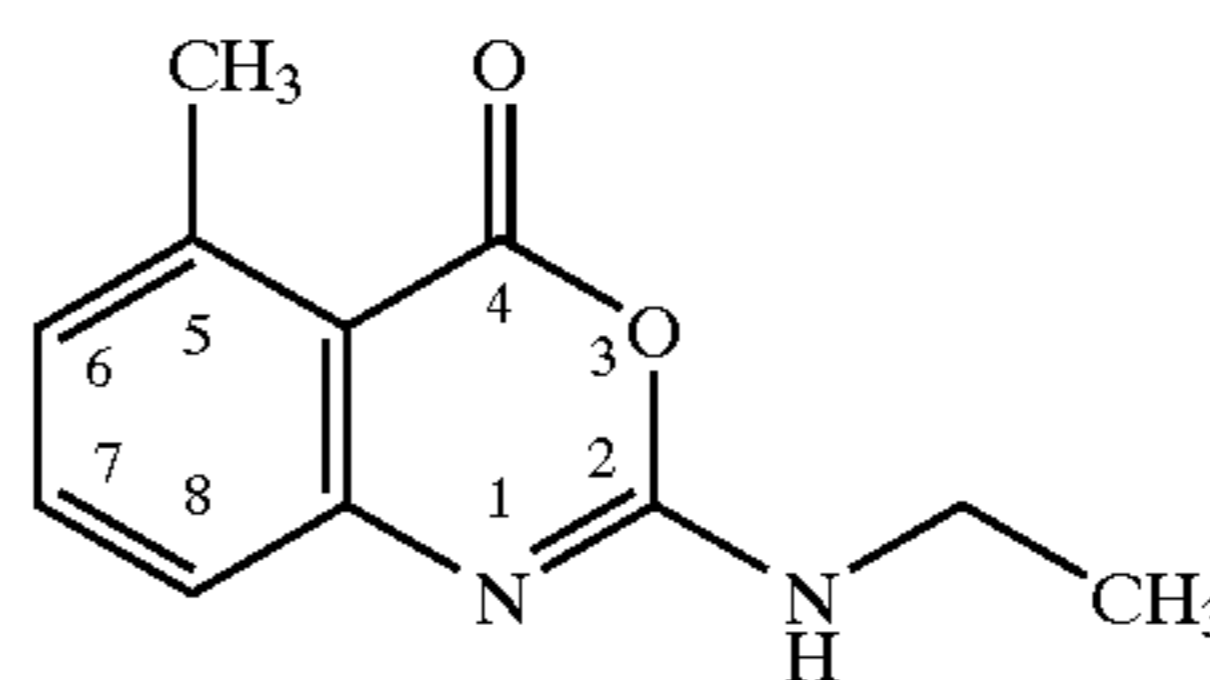
2-Ethylamino-5-methyl-4H-3,1-benzoxazin-4-one
