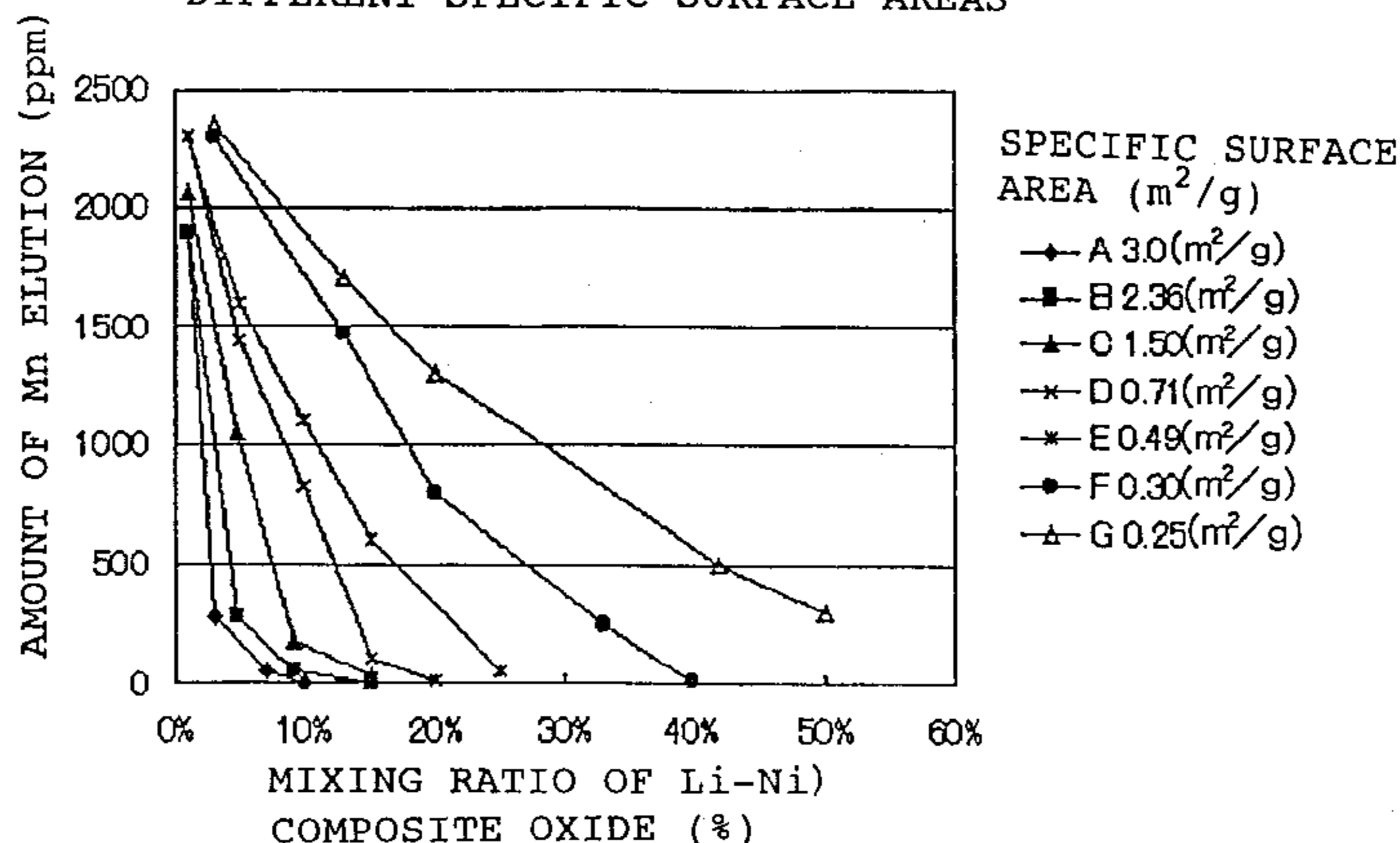
AMOUNT OF Mn ELUTION WITH RESPECT TO MIXING RATIO OF Li-Ni COMPOSITE OXIDE HAVING DIFFERENT SPECIFIC SURFACE AREAS
