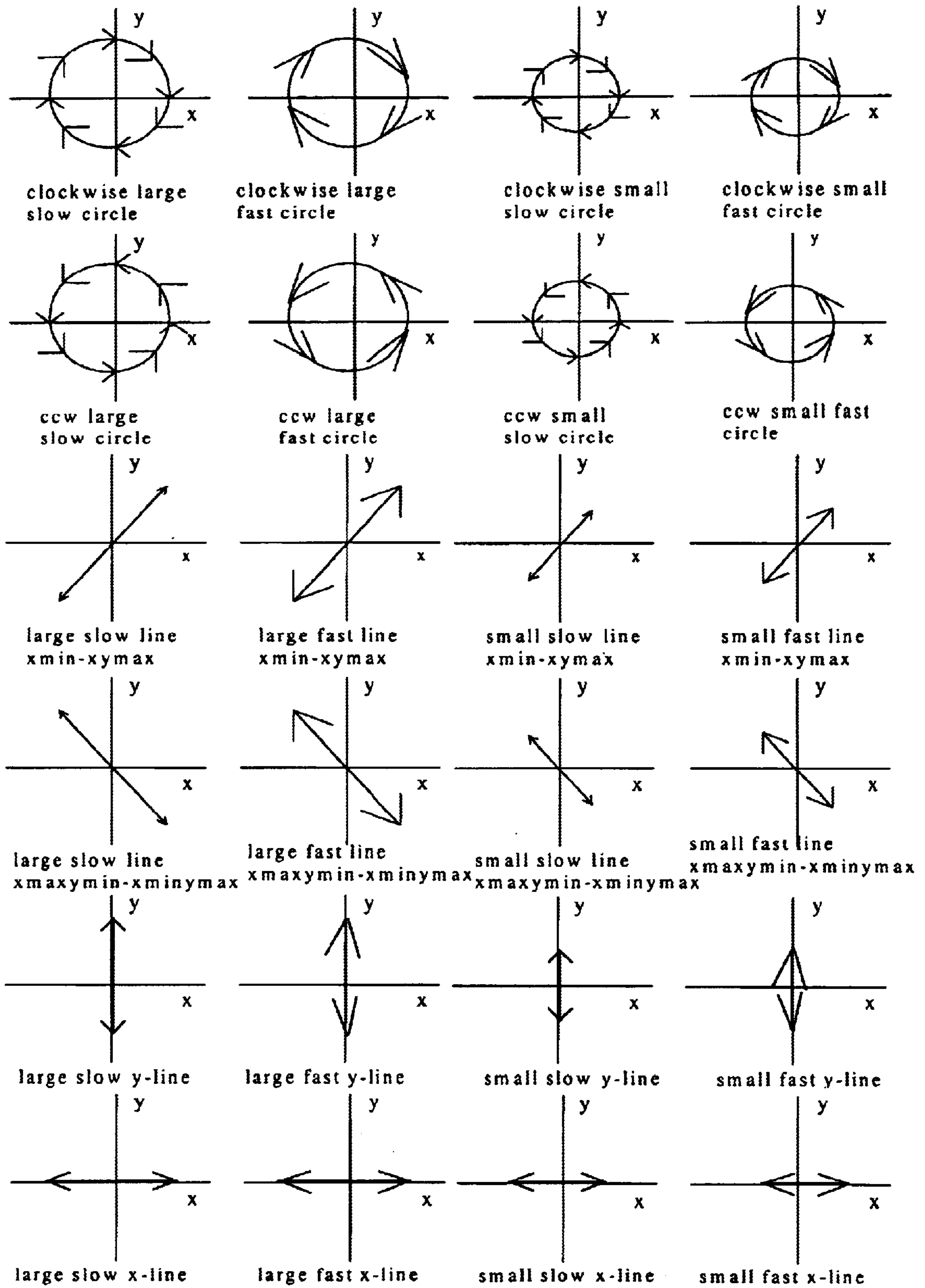
Figure 6: An Example 24 Gesture Lexicon.
