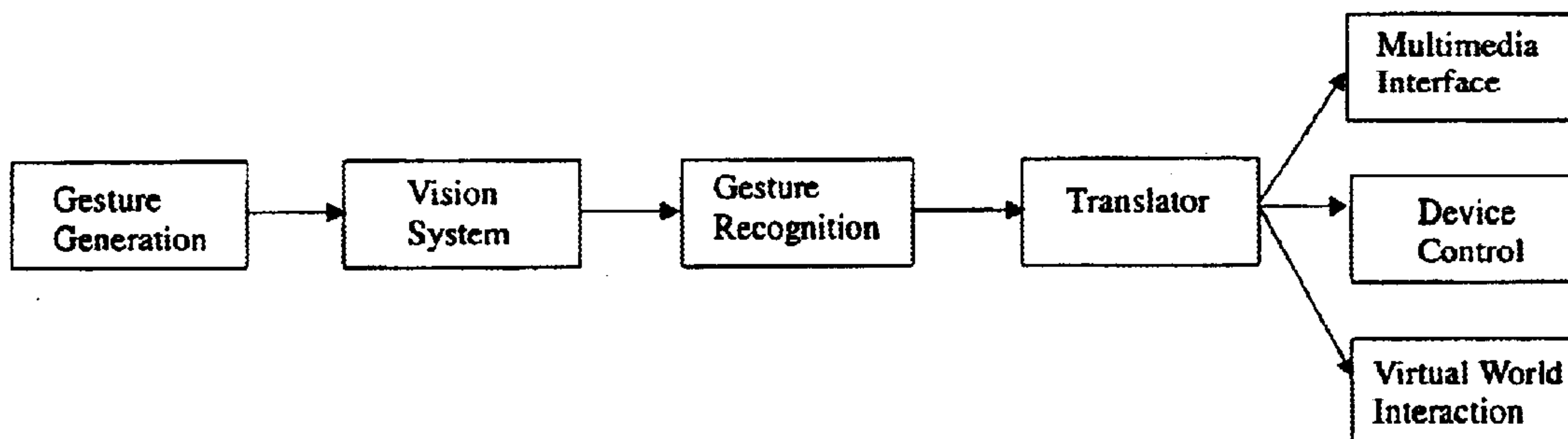
Figure 2: Gesture Recognition System Flow Chart.
