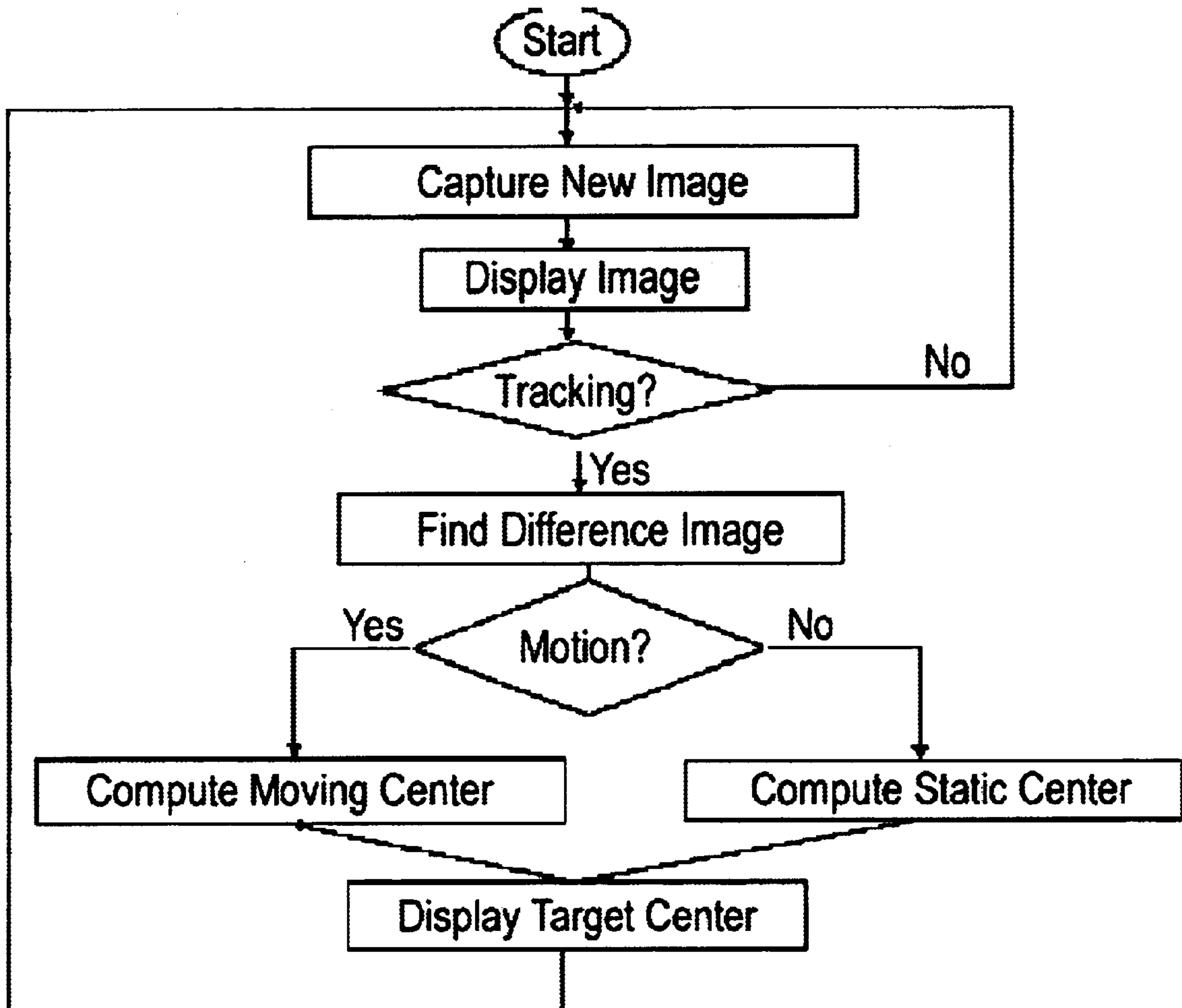
Figure 27: Flowchart of the CTS.
