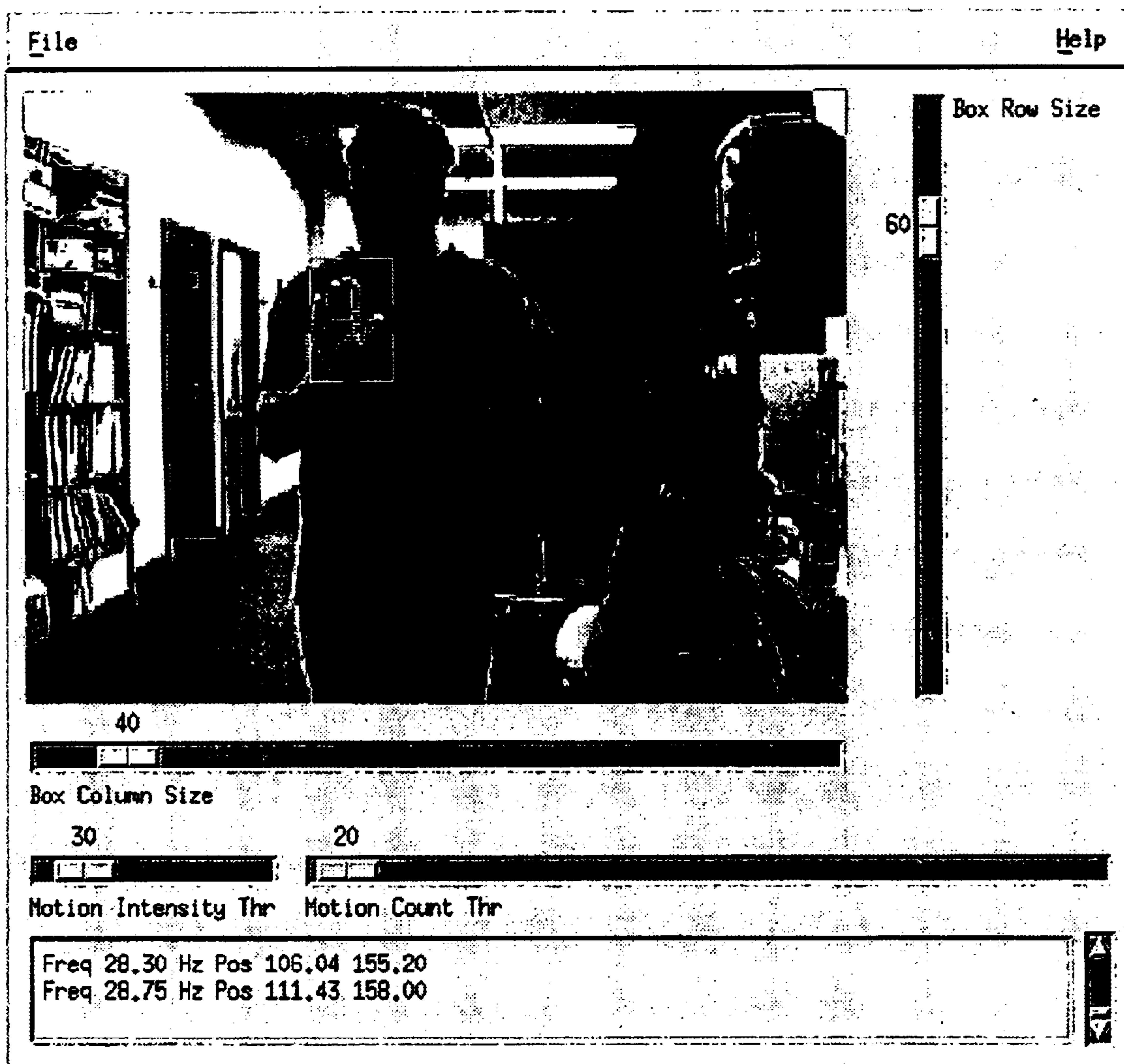
Figure 28: Graphical User Interface of the CTS.
