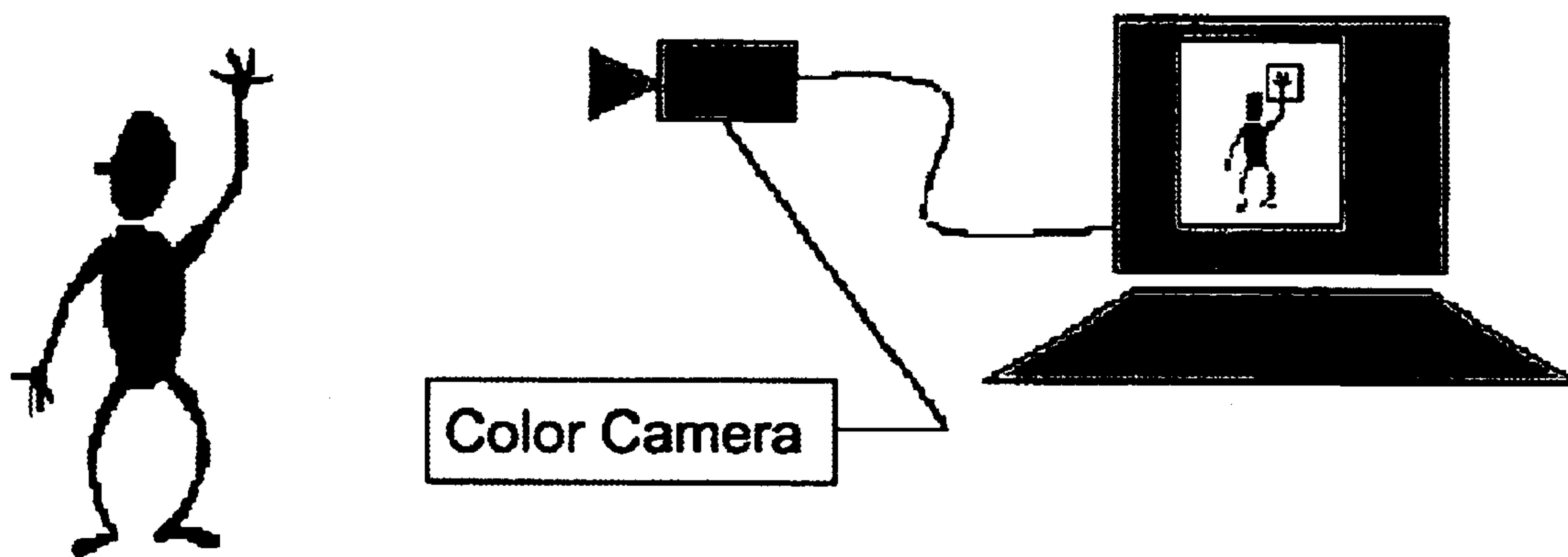
Figure 26: Schematic of the Hand Tracking System Hardware.
