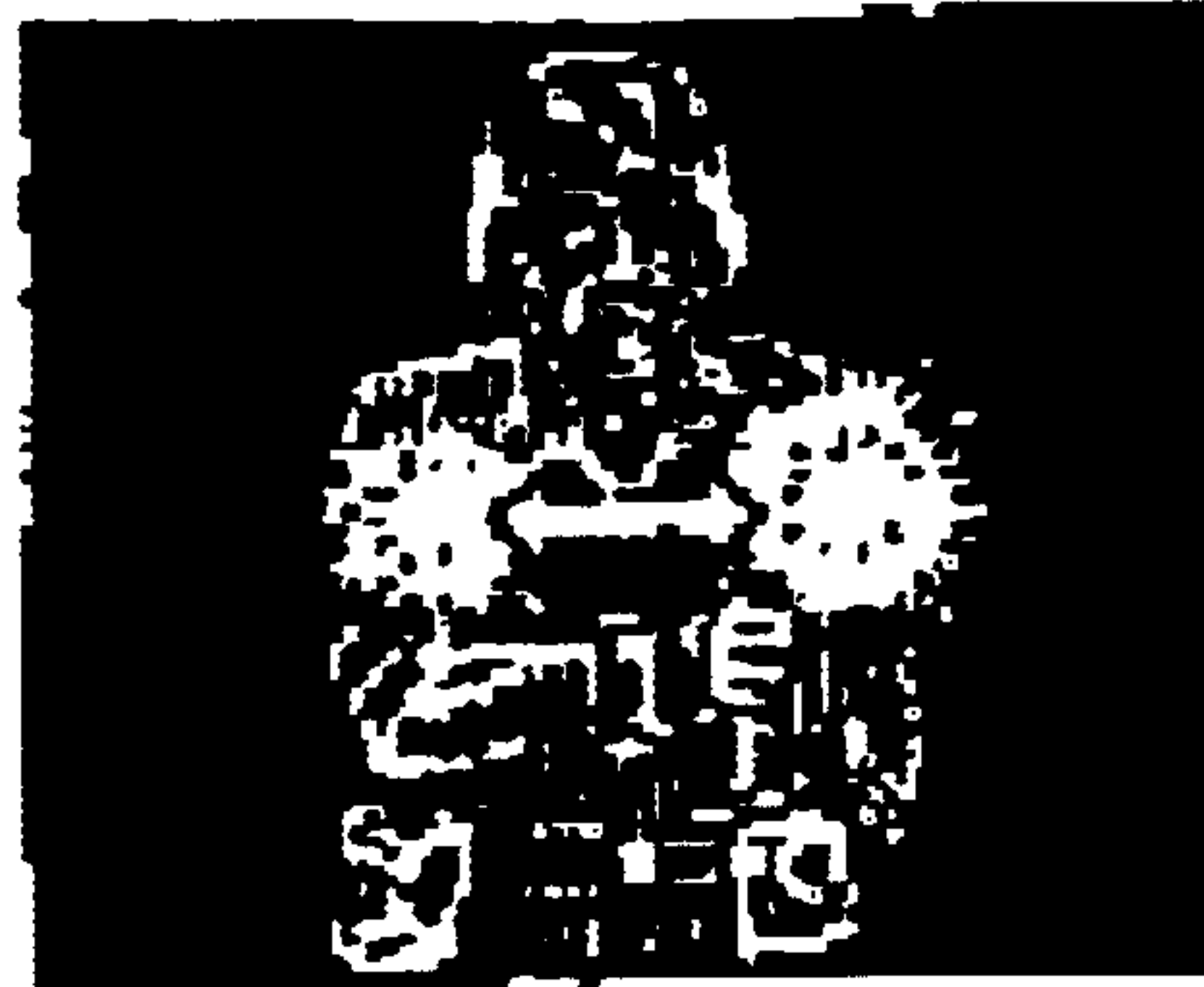
Figure 10: Stop Gesture.
