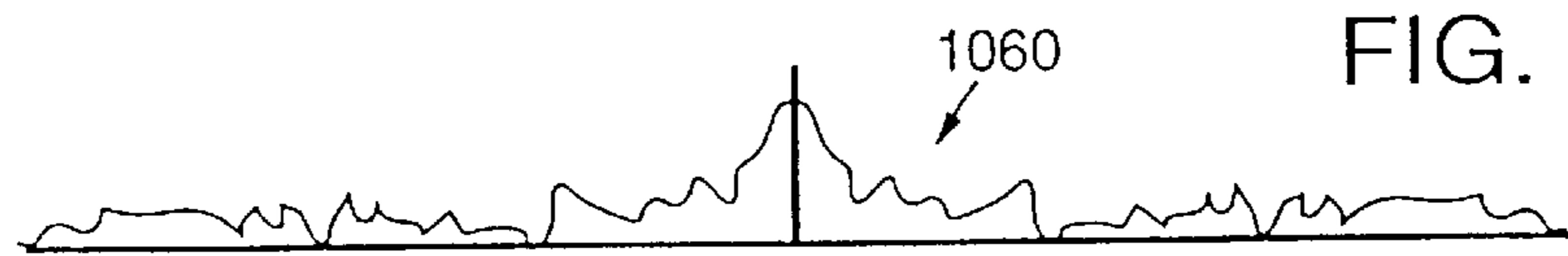
MAGNITUDE OF FOURIER TRANSFORM OF SCAN DATA
