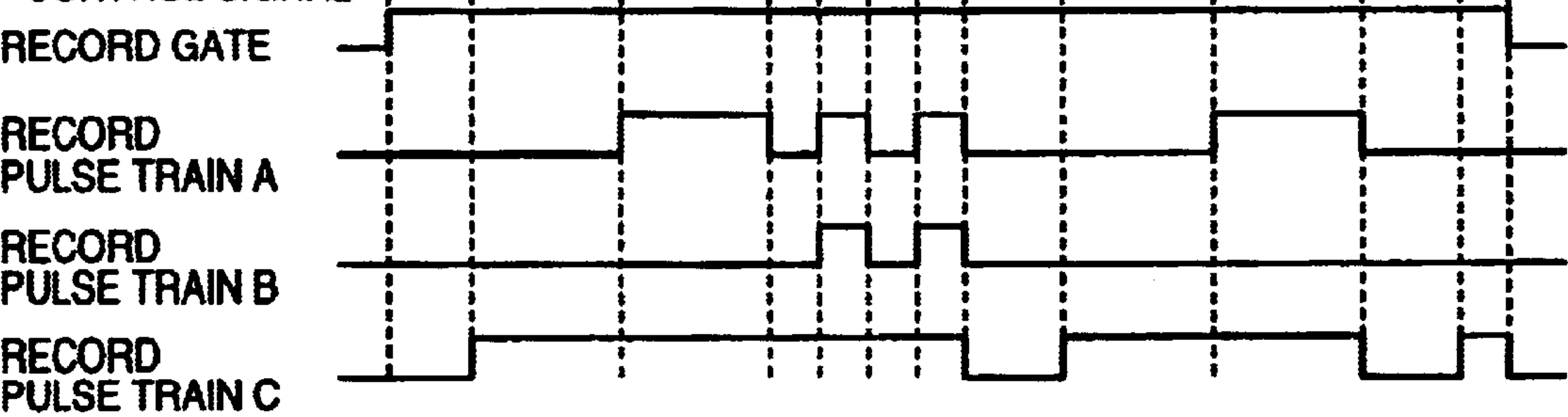
CONTROL SIGNAL
