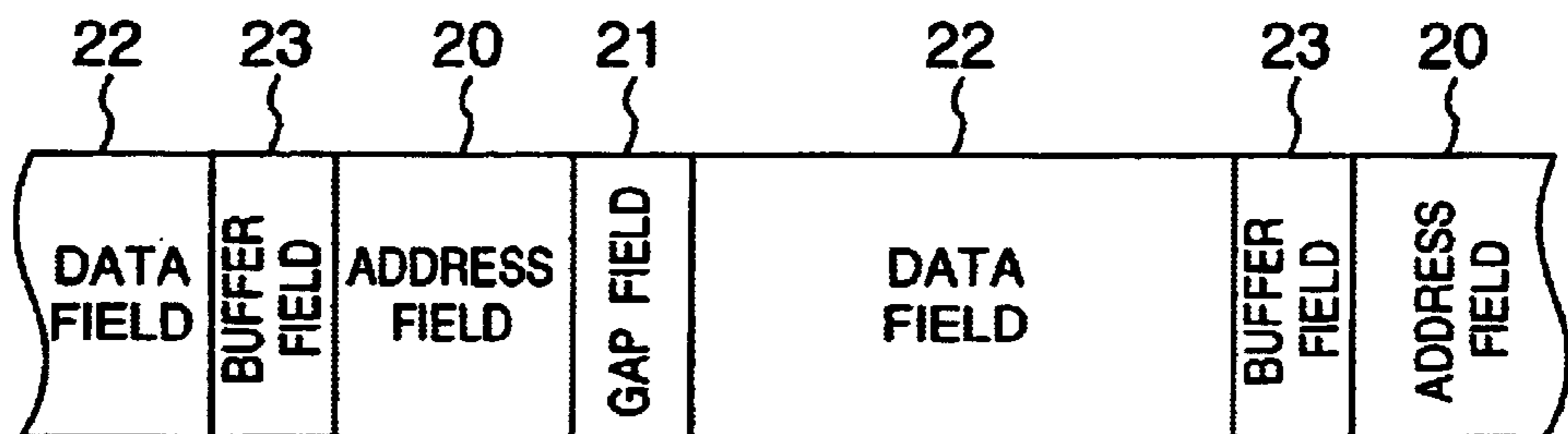
FIG.13A SECTOR FORMAT
