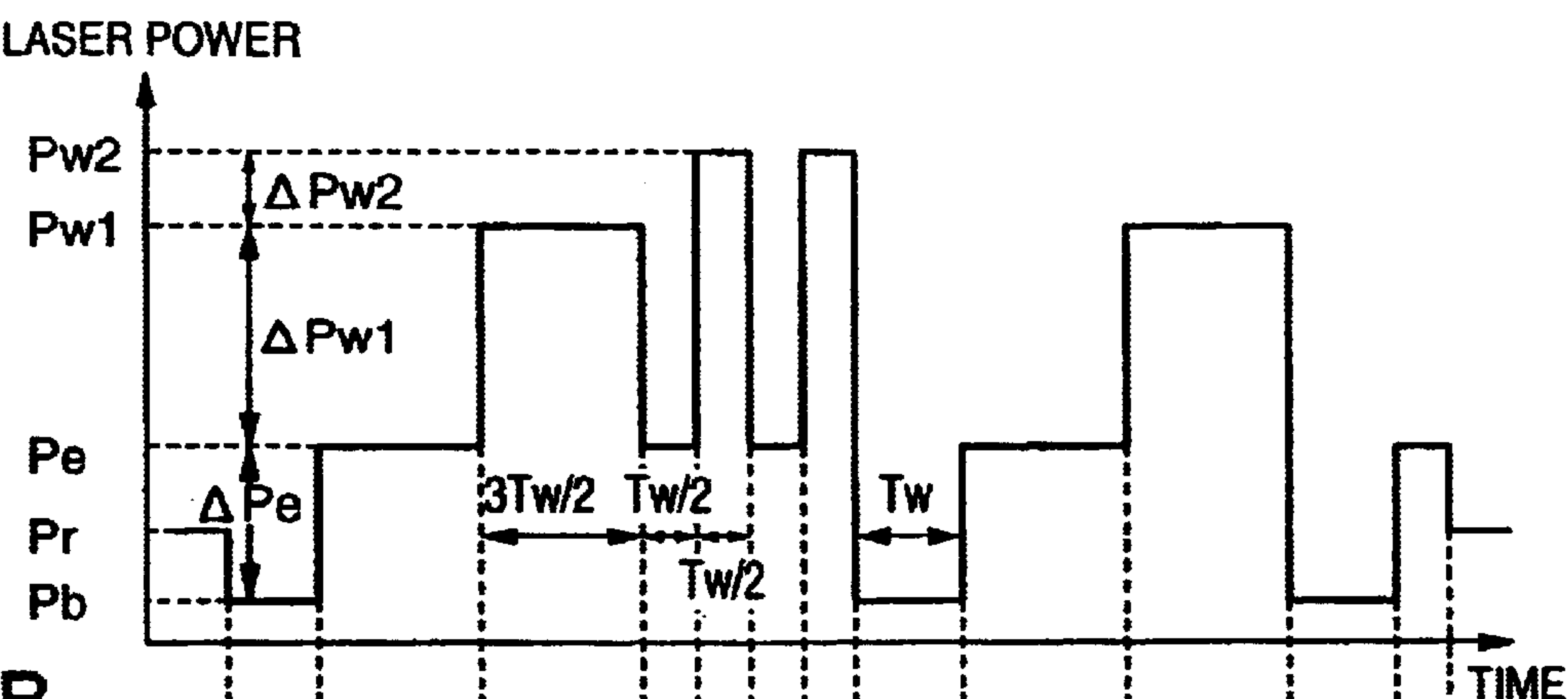
RECORD WAVEFORM
