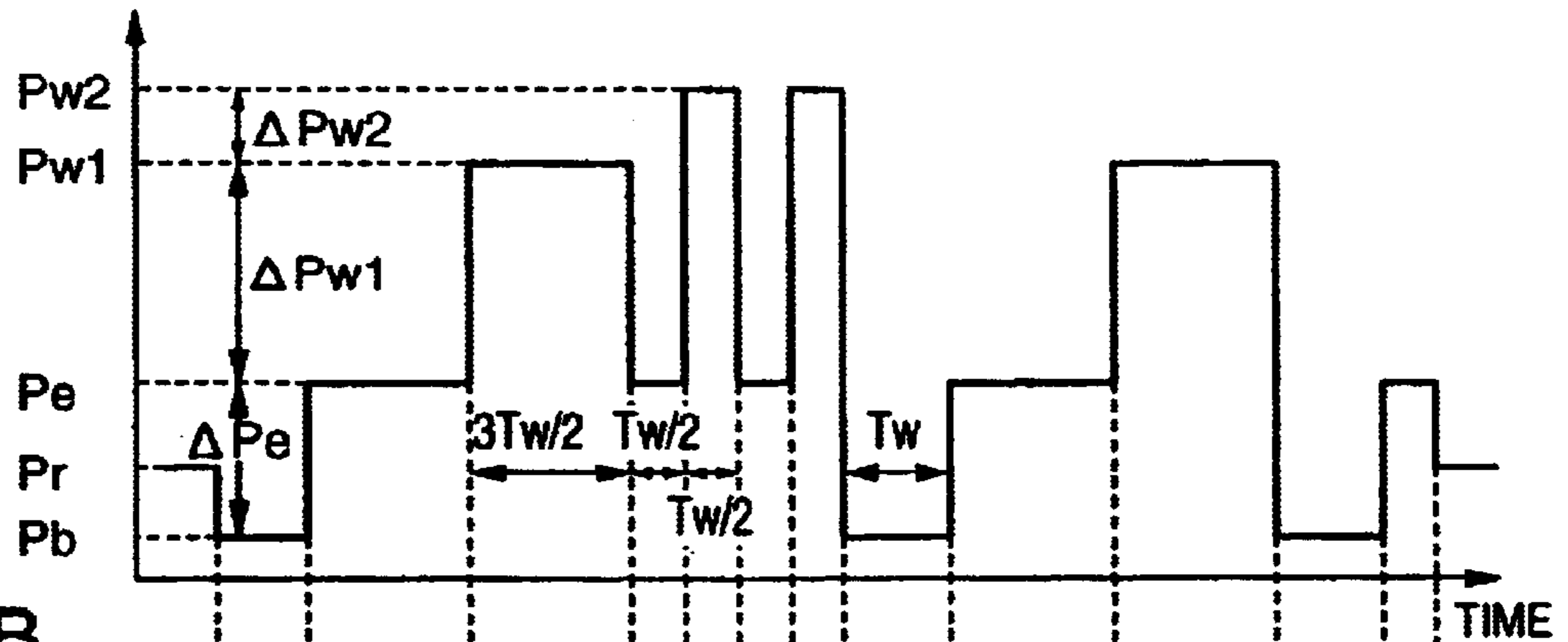
RECORD WAVEFORM
